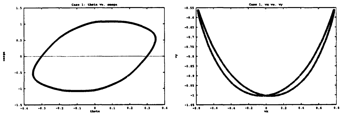
Figure 5: Lossless casel with \theta_0 = 0.3\text{rad} , \dot{\theta}_0 = 0\text{rad/s} , \kappa = 1.1
