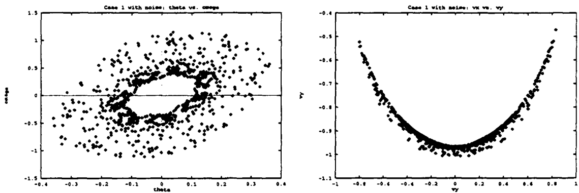
Figure 11: Case 1 with noise
