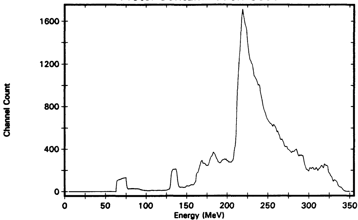
Figure B-15. Isotropic Distribution, Channel 15
