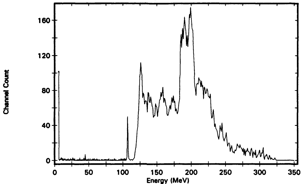
Figure B-1. Isotropic Distribution, Channel 1
