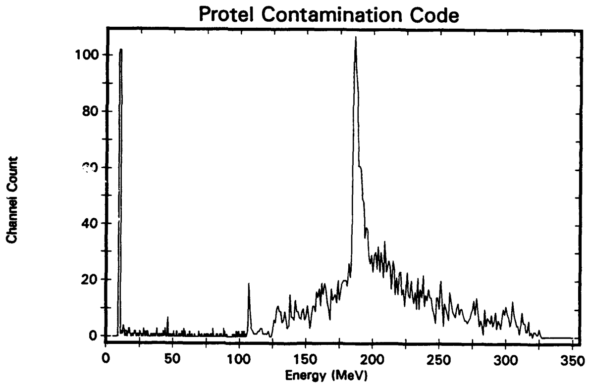
Figure B-4. Isotropic Distribution, Channel 4
