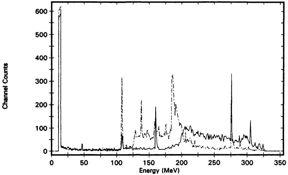
Figure B-21. Mirror Plane Distribution, Channel 5 Solid Line: 0 deg., Dashed: 90 deg. orientation with respect to Magnet
