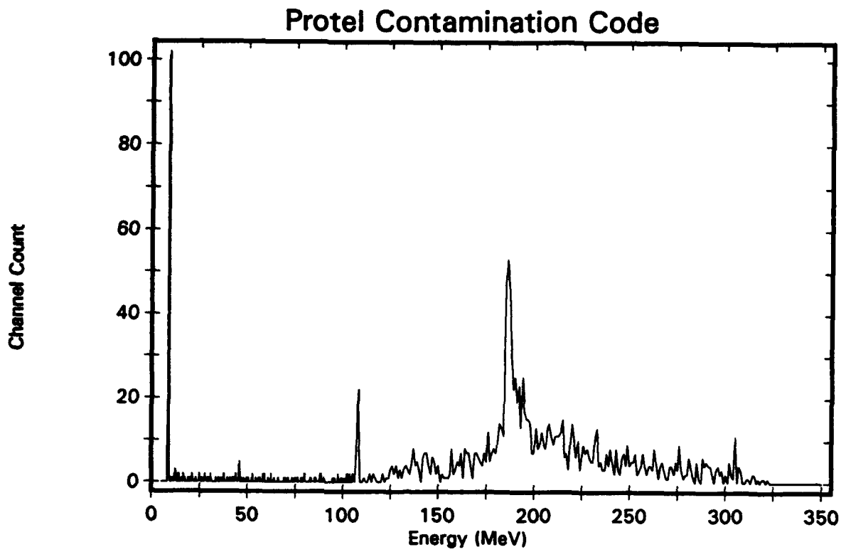
Figure B-3. Isotropic Distribution, Channel 3
