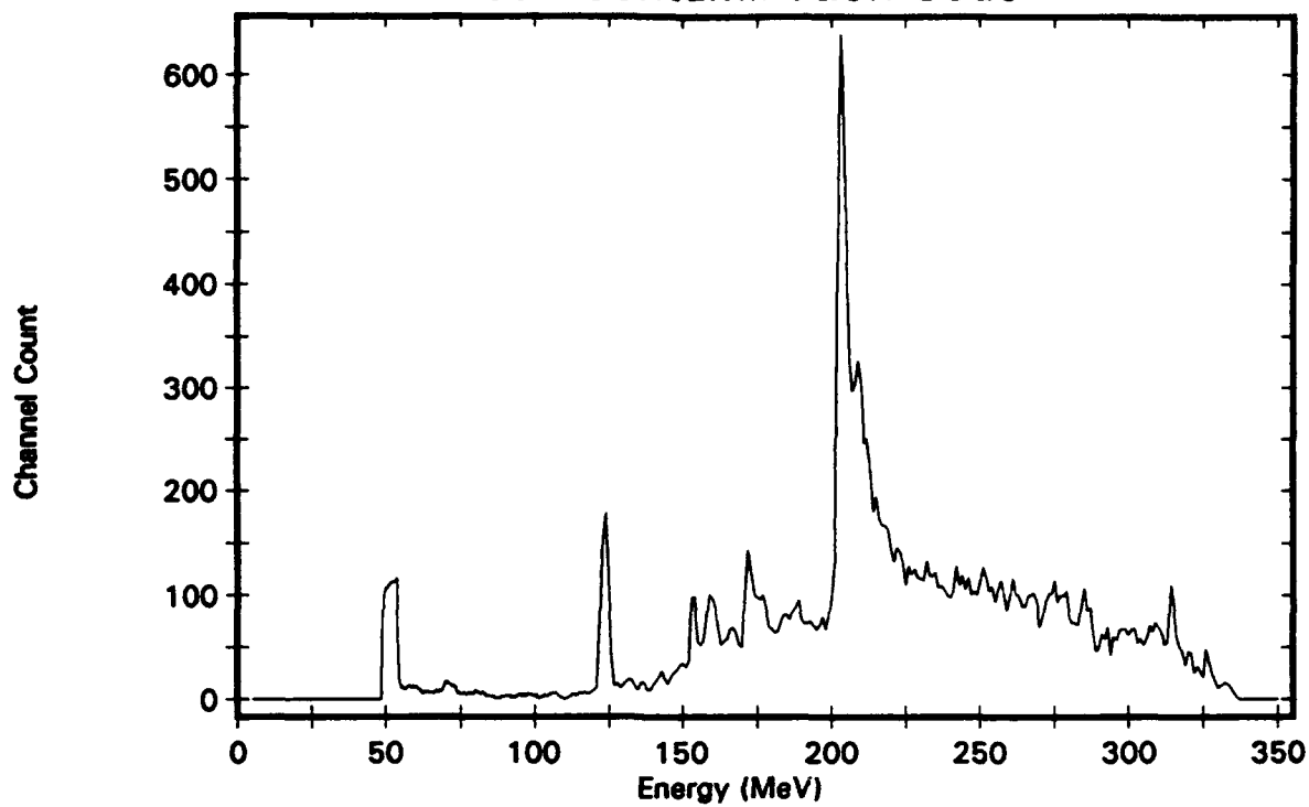
Figure B-13. Isotropic Distribution, Channel 13
