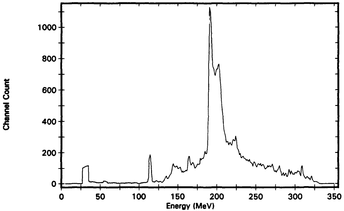
Figure B-10. Isotropic Distribution, Channel 10
