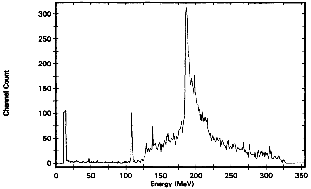
Figure B-5. Isotropic Distribution, Channel 5
