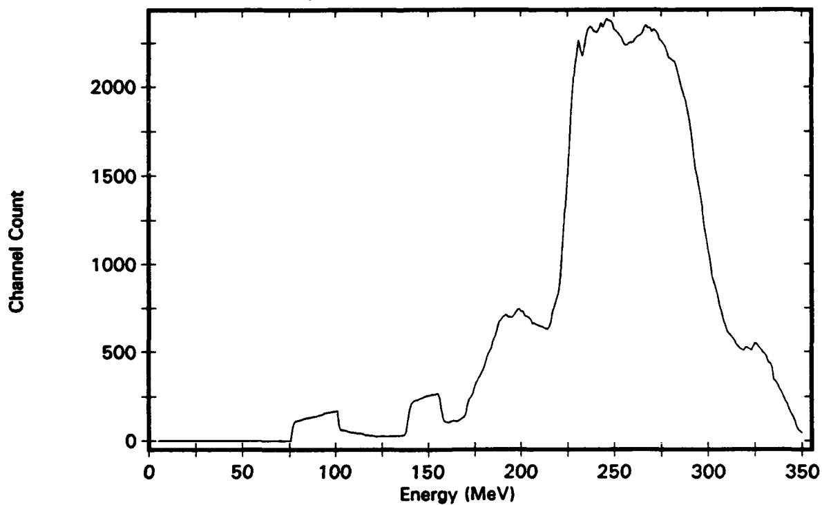
Figure B-16. Isotropic Distribution, Channel 16
