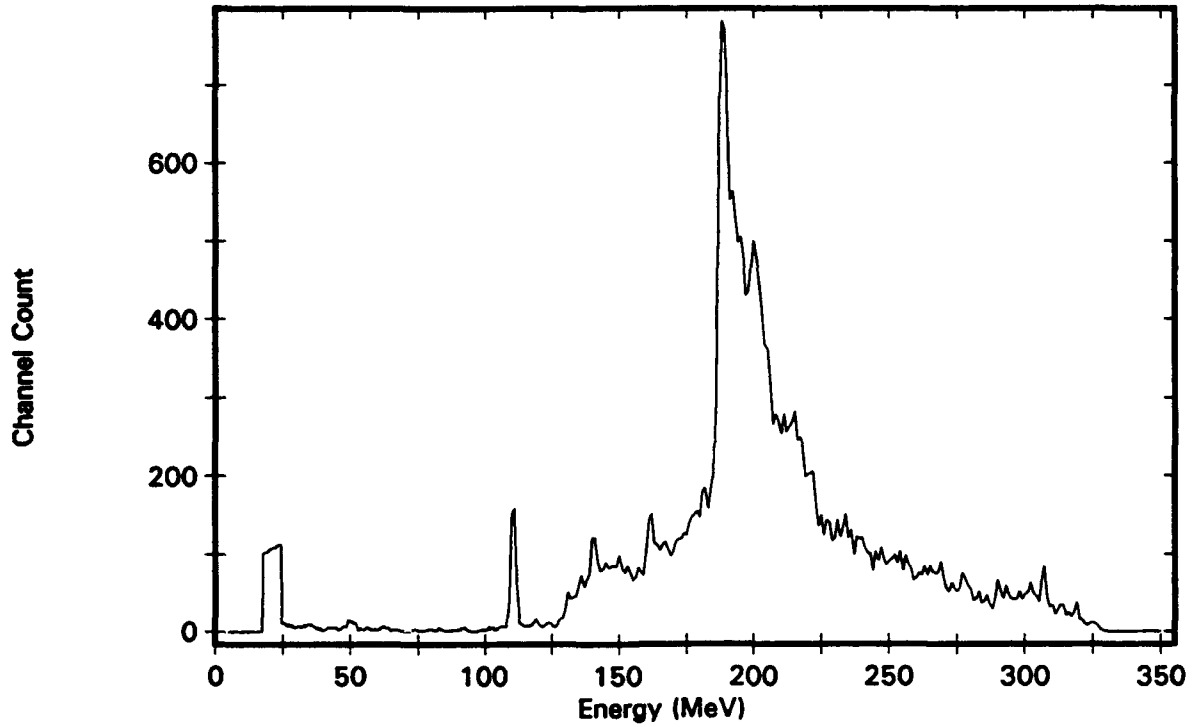
Figure B-8. Isotropic Distribution, Channel 8
