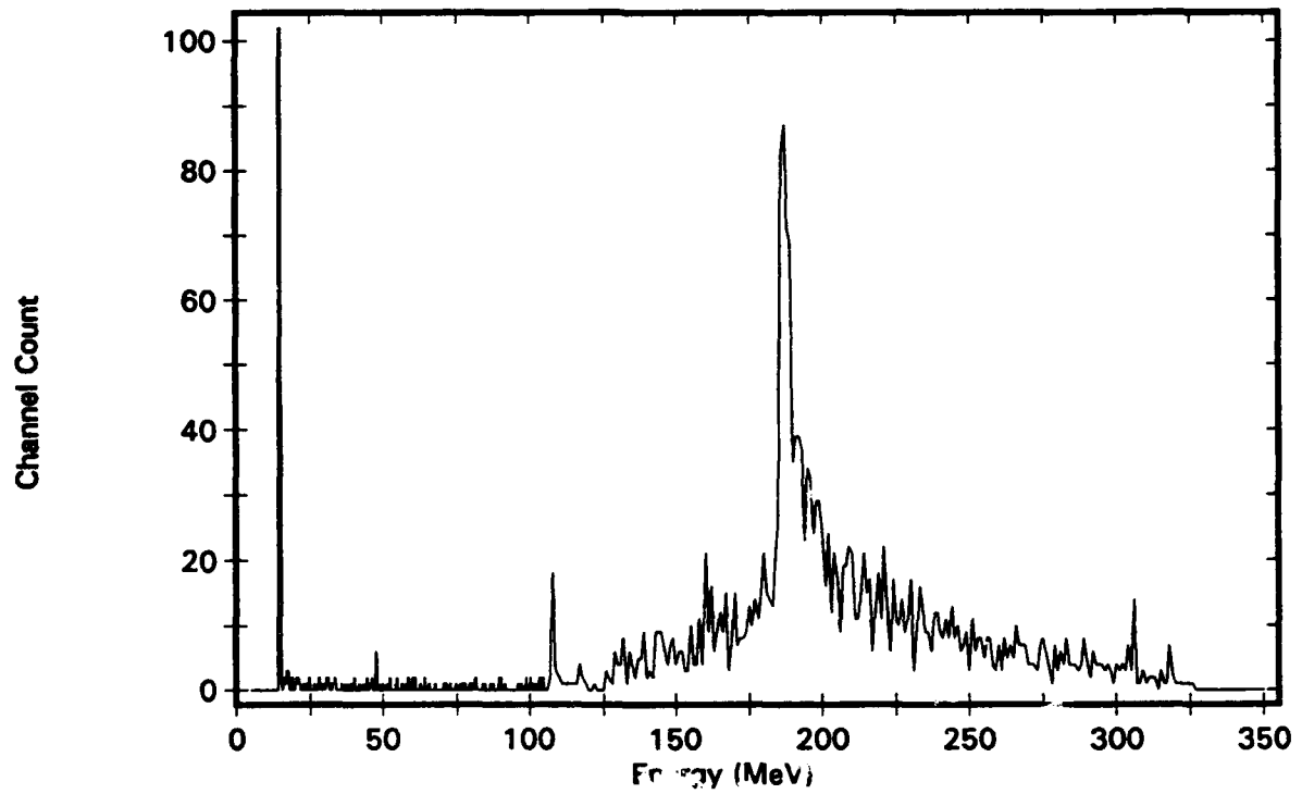
Figure B-6. Isotropic Distribution, Channel 6
