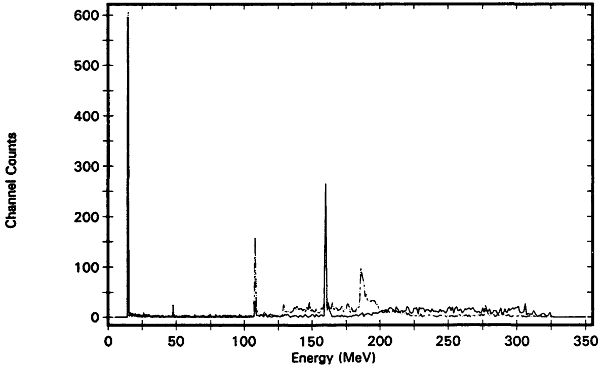
Figure B-22. Mirror Plane Distribution, Channel 6 Solid Line: 0 deg., Dashed: 90 deg. orientation with respect to Magnet
