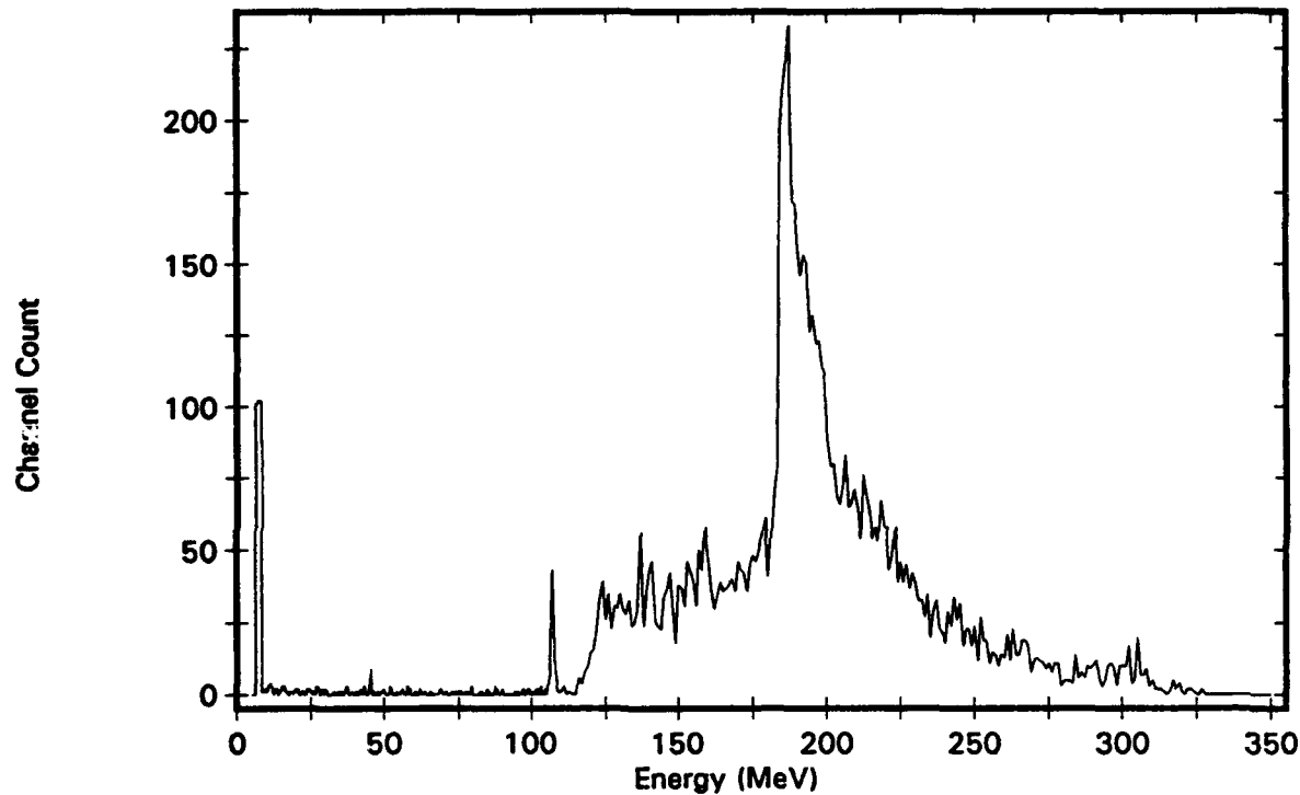
Figure B-2. Isotropic Distribution, Channel 2
