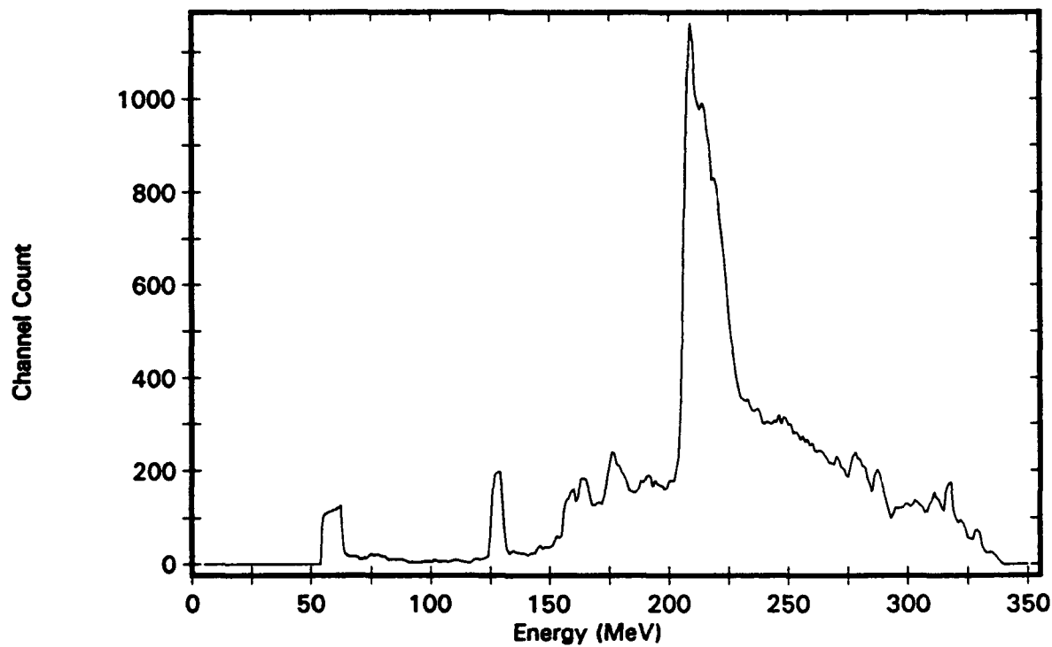
Figure B-14. Isotropic Distribution, Channel 14
