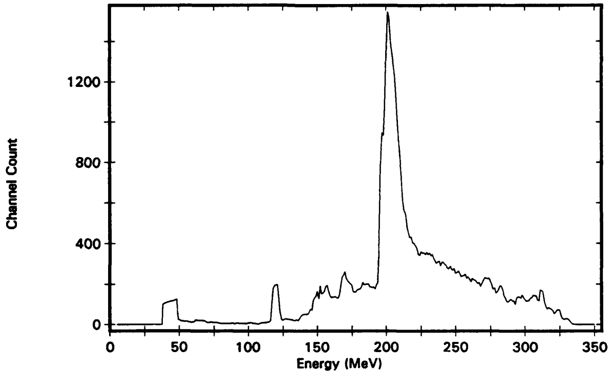
Figure B-12. Isotropic Distribution, Channel 12
