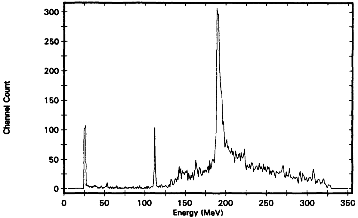
Figure B-9. Isotropic Distribution, Channel 9
