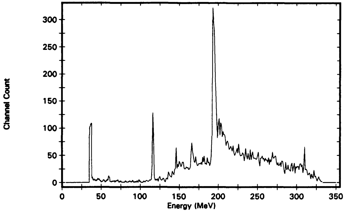
Figure B-11. Isotropic Distribution, Channel 11
