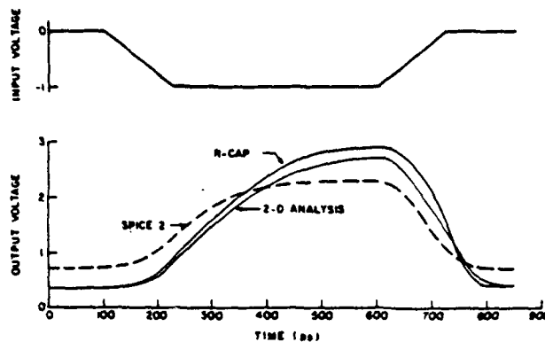
Fig. 12. Comparison of simulation results using R-CAP, SPICE 2 and the two-dimensional analysis for the device of Fig. 11 with V_D=3.5 \text{ V} and for SPICE 2: V_T=2.5 \text{ V} , \beta=71 \mu\text{A}/\text{V}^2 , \lambda=0 , V_{BI}=0.5 \text{ V} , C_{12}(0)=6 \text{ fF} , C_{13}(0)=1 \text{ fF} , for R-CAP: \alpha=1.5/\text{V} , \beta=65 \mu\text{A}/\text{V}^2 , V_T=2.5 \text{ V} , V_{BI}=0.5 \text{ V} , C_{12}(0)=6 \text{ fF} , C_{13}=0.3 \text{ fF} , \tau=10 \text{ ps} . For Both: R_1=R_2=R_3=C_{13}=0 , C_L=6 \text{ fF} , driver width = 10 \mu\text{m} , load width = 5 \mu\text{m} .
