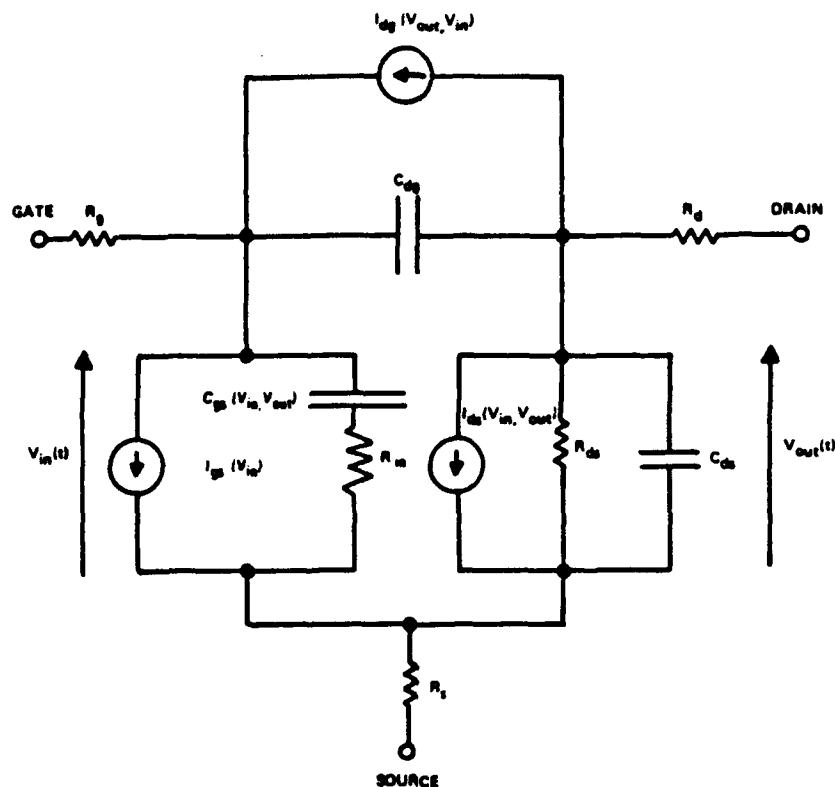
EQUIVALENT CIRCUIT OF GaAs MESFET
