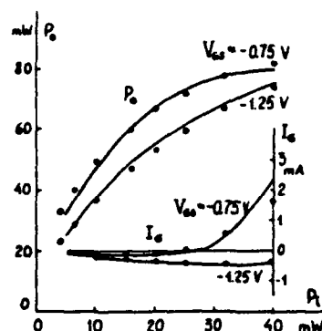
Fig. 5. Output power P_o and dc gate current I_g versus input power P_i . Measurements (OOO), calculations (—), f = 9.5 GHz, and V_{DS} = 4 V.
