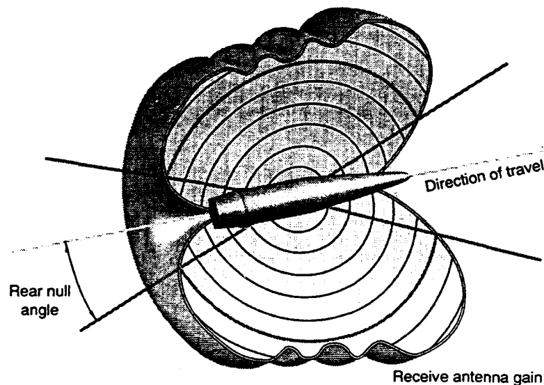
Figure 1. Antenna nulls.
