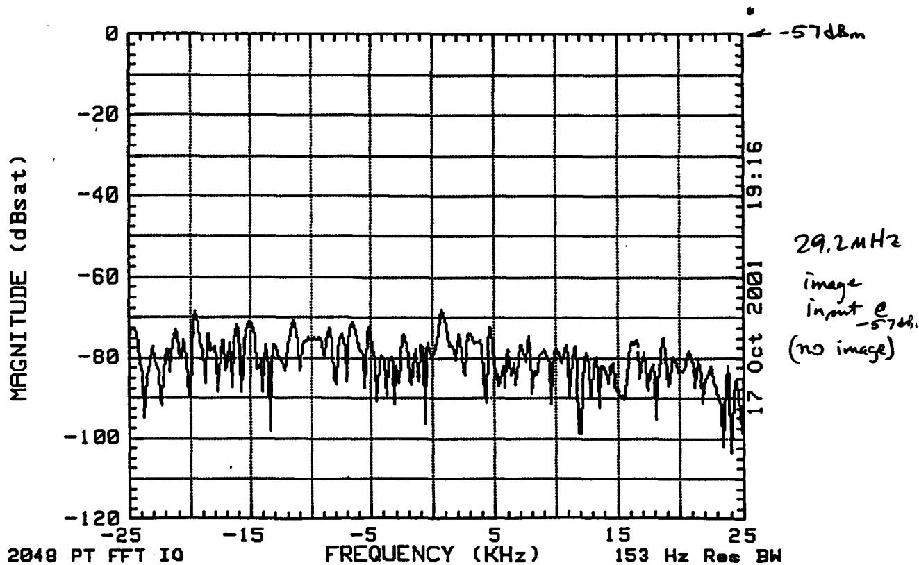
Figure 37 Various Measured Results RF Image Test
