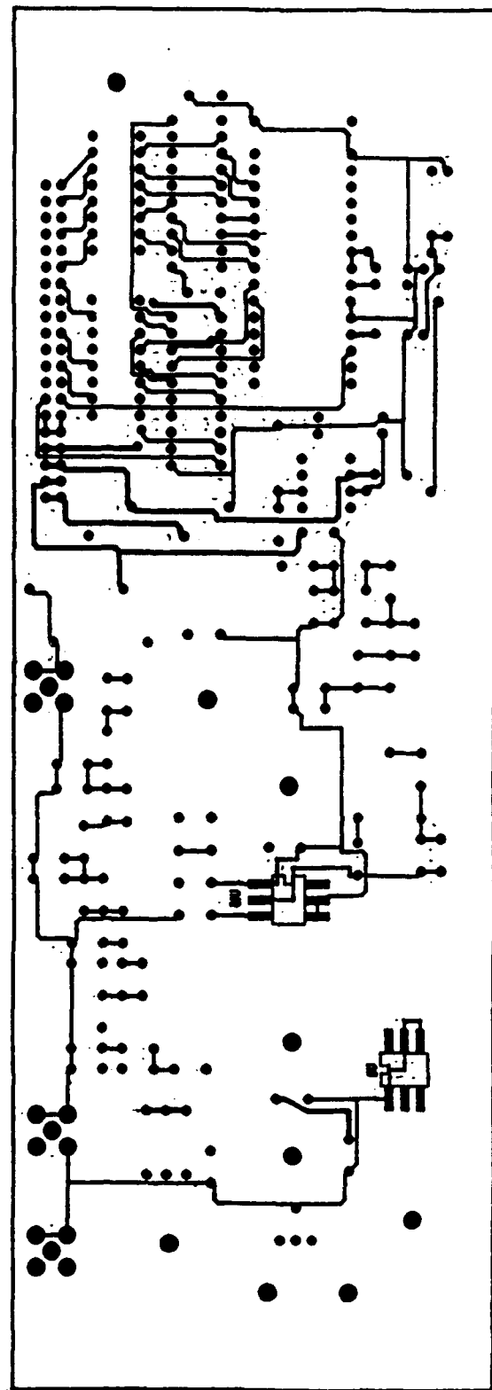
Figure 31 Meteorburst Receiver (Continued)
