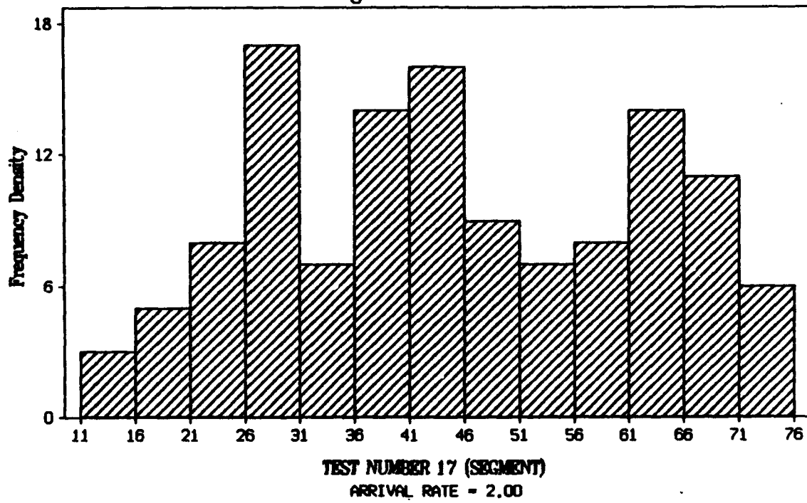
Histogram - EXPERIMENT
