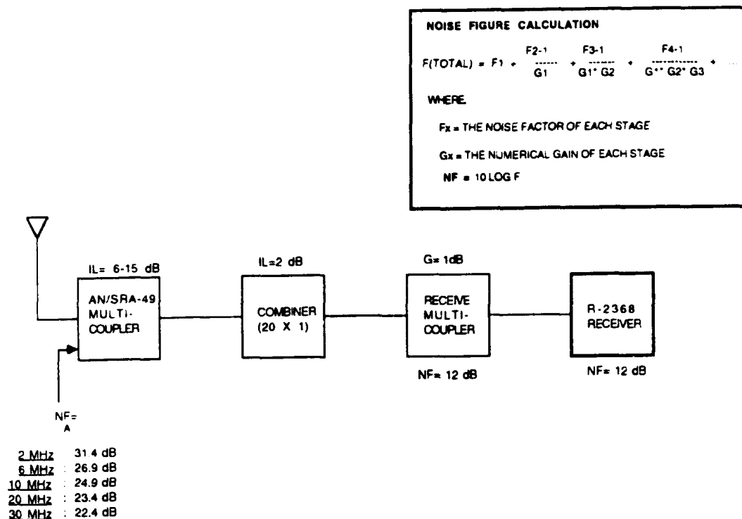
Figure 22. Noise figure calculations for option 3B: Broadband receiving system.
