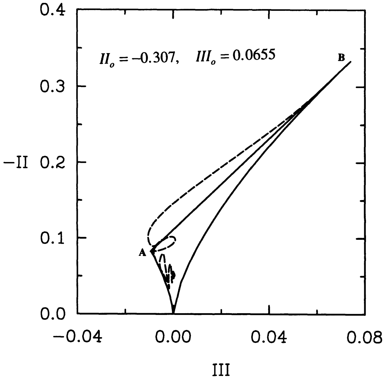
Figure 4. Computed phase space trajectories in homogeneous shear flow for the initial conditions (b_{11})_0 = -0.32 , (b_{22})_0 = -0.32 , SK_0/\epsilon_0 = 50 : (a) Shih-Lumley Model and (b) the IP Model of Launder and co-workers.
