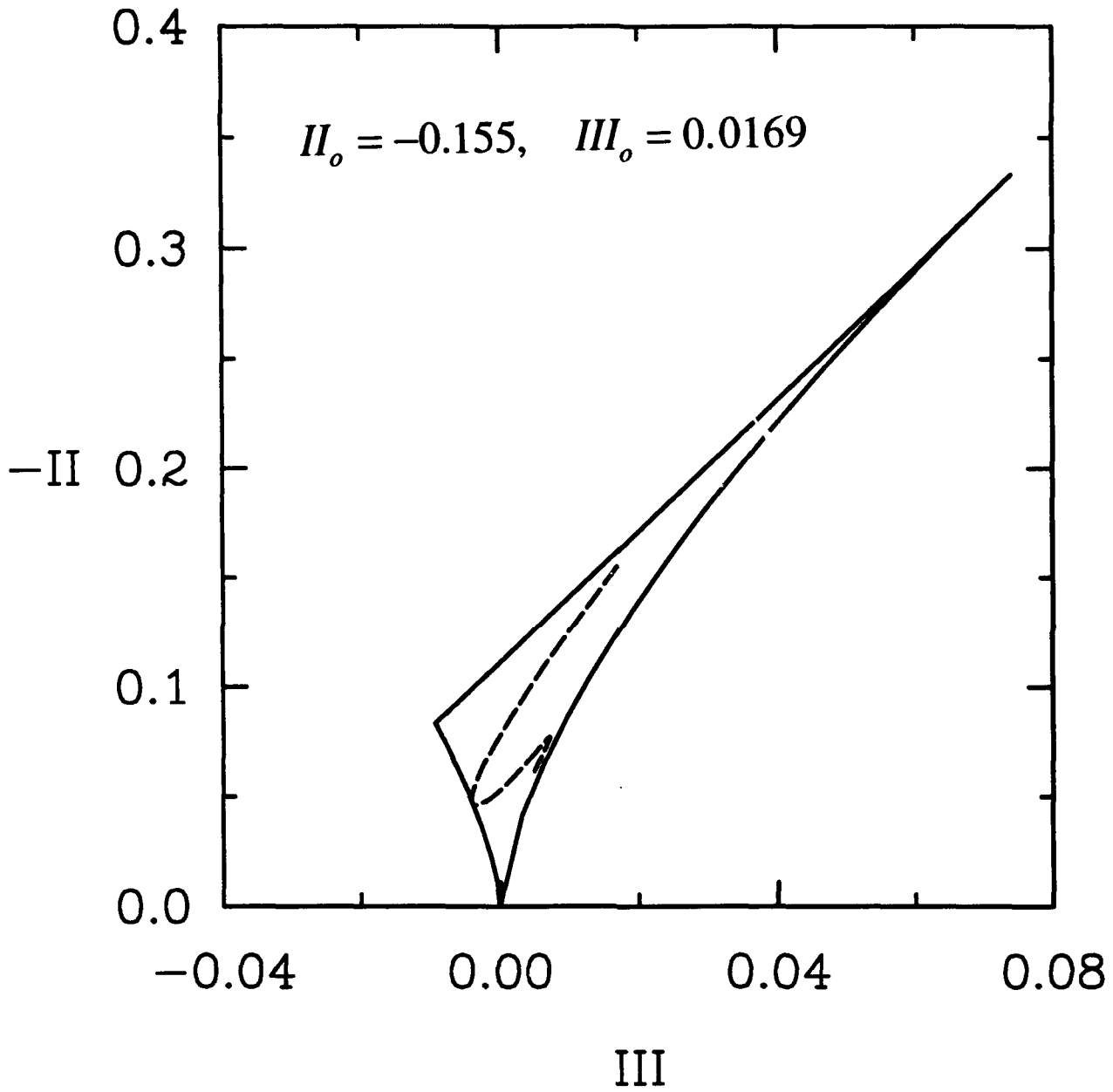
Figure 7. Computed phase space trajectories for homogeneous shear flow corresponding to the initial conditions (b_{11})_0 = -0.32 , (b_{22})_0 = -0.12 , SK_0/\varepsilon_0 = 50 : (a) the Shih-Lumley Model and (b) the IP Model of Launder and co-workers.
