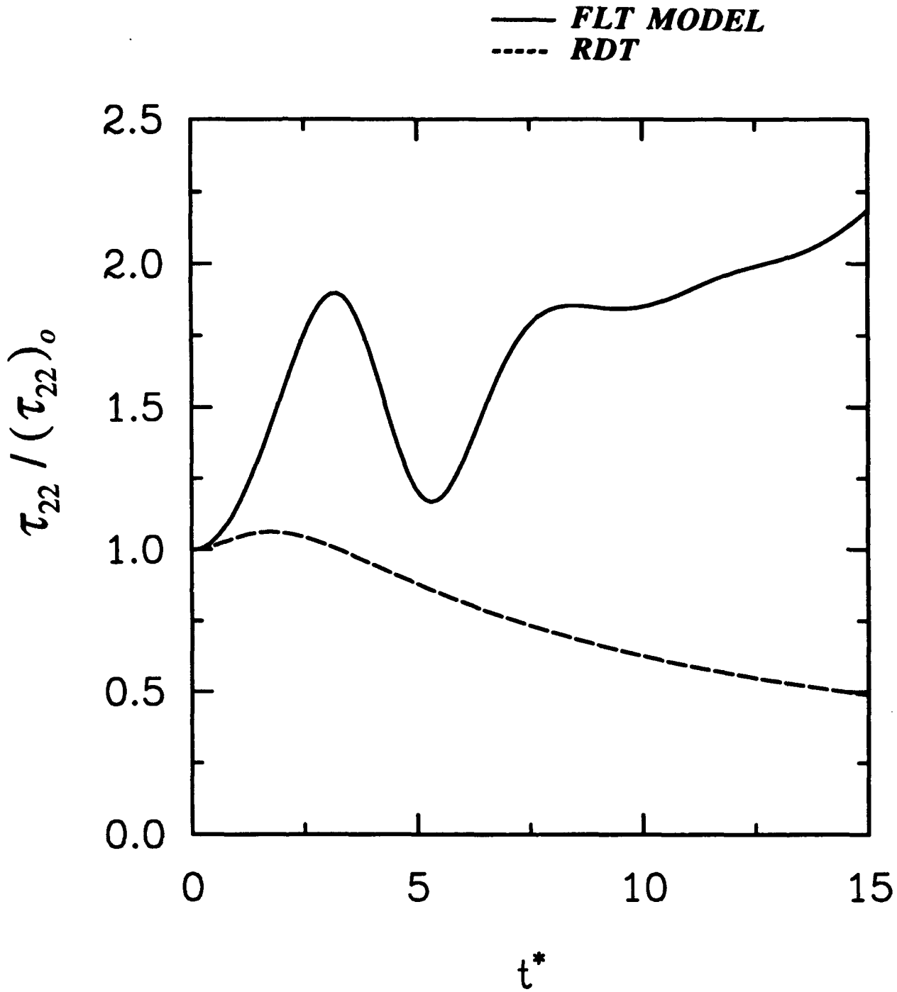
Figure 12. Time evolution of the normal Reynolds stress \tau_{22}/(\tau_{22})_0 in homogeneous shear flow: Comparison of computed results for the FLT Model (corresponding to (b_{11})_0 = (b_{22})_0 = -0.0833 , SK_0/\varepsilon_0 = 50 ) with the Rapid Distortion Theory (RDT) solution.
