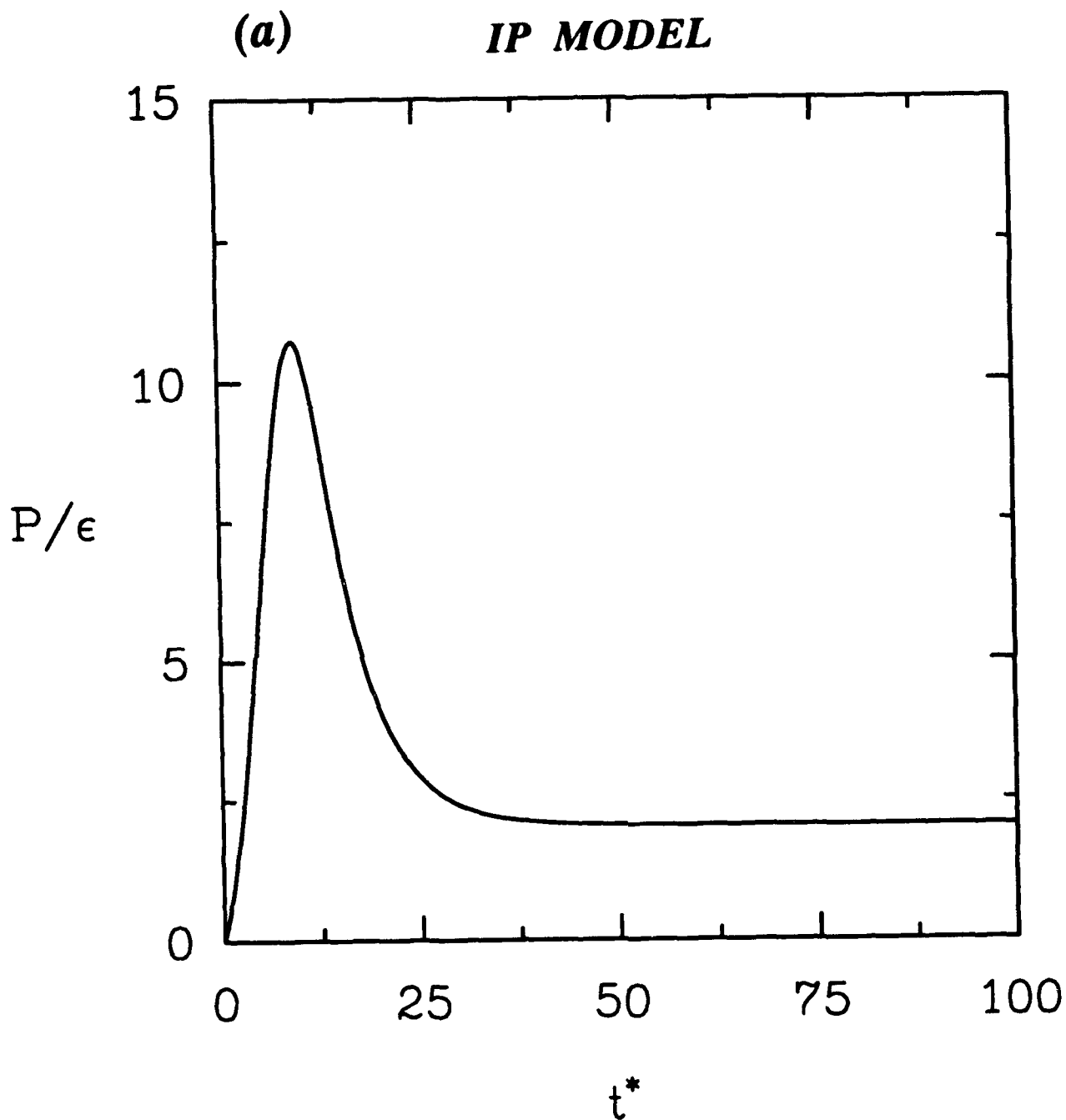
Figure 11. Computed model predictions for the time evolution of the ratio of production to dissipation ( P/\epsilon ) in homogeneous shear flow corresponding to the initial conditions (b_{11})_0 = -0.32 , (b_{22})_0 = -0.32 , SK_0/\epsilon_0 = 50 : (a) IP Model, (b) Shih-Lumley Model and (c) the FLT Model.
