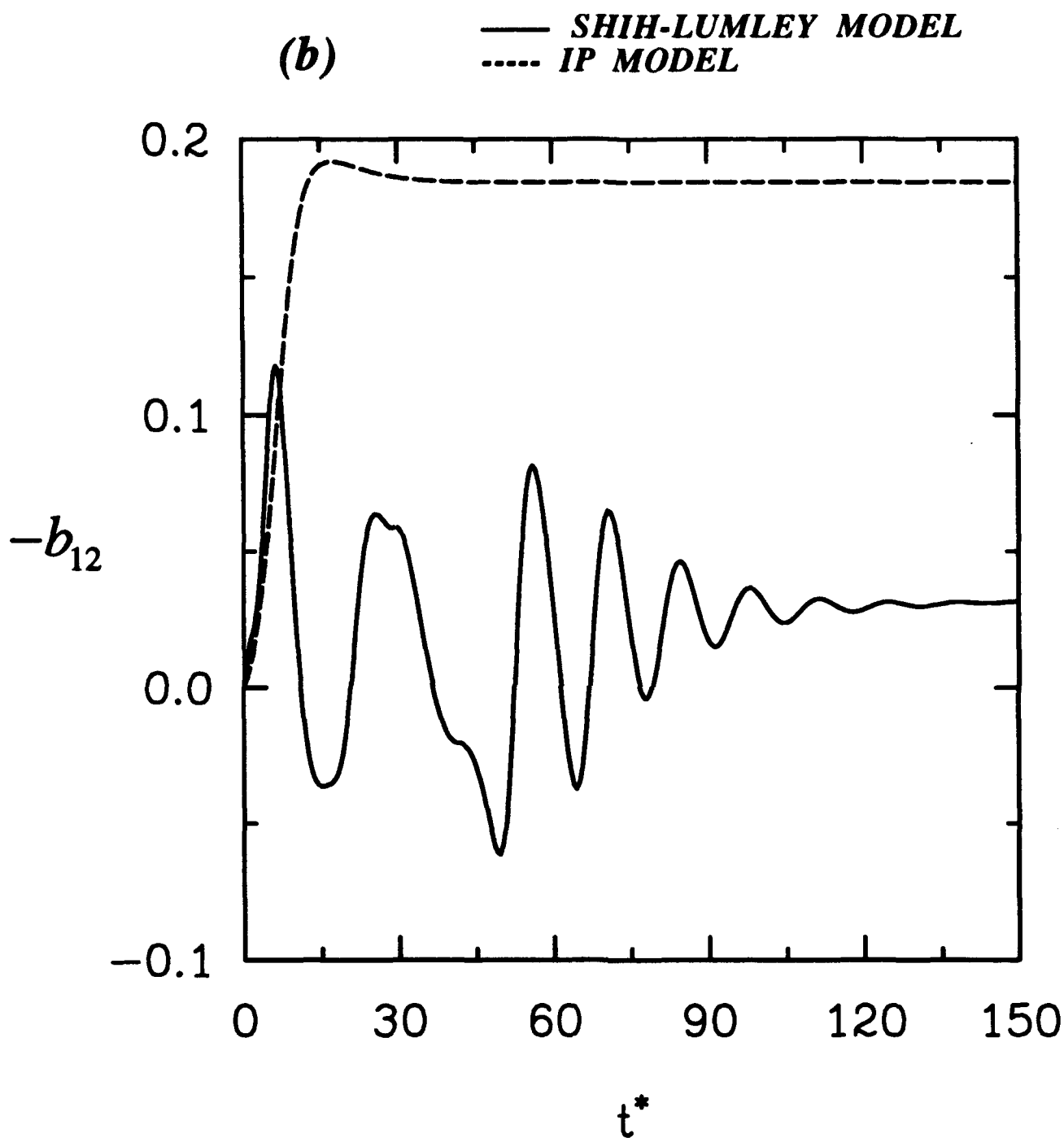
Figure 5. Model predictions for the time evolution of the Reynolds stress anisotropies in homogeneous shear flow corresponding to the initial conditions (b_{11})_0 = -0.32 , (b_{22})_0 = -0.32 , SK_0/\varepsilon_0 = 50 : (a) F and (b) b_{12} .
