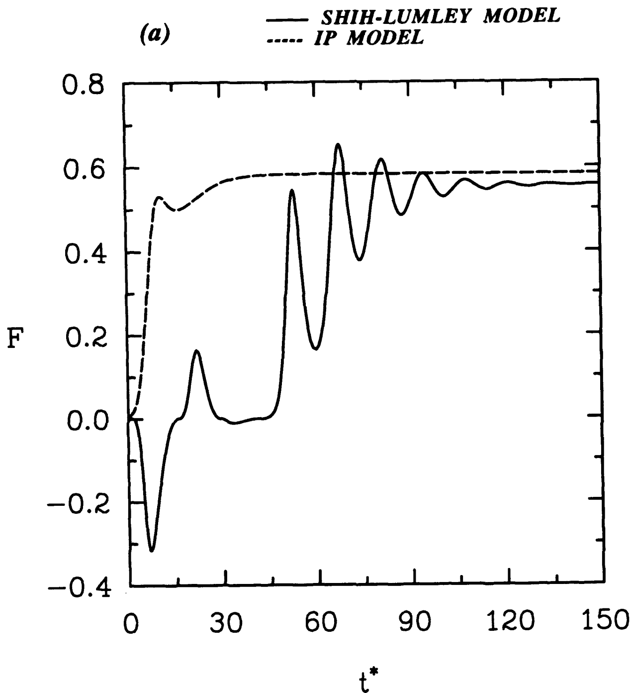
Figure 5. Model predictions for the time evolution of the Reynolds stress anisotropies in homogeneous shear flow corresponding to the initial conditions (b_{11})_0 = -0.32 , (b_{22})_0 = -0.32 , SK_0/\epsilon_0 = 50 : (a) F and (b) b_{12} .
