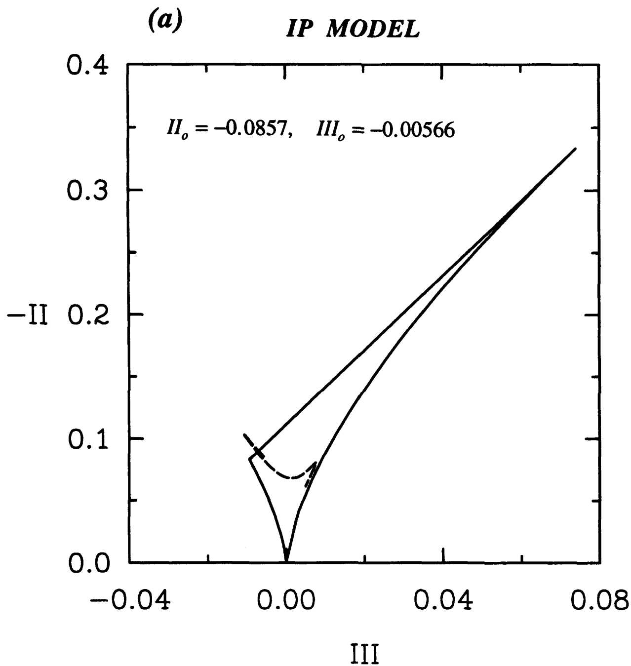
Figure 8. Computed phase space trajectories for homogeneous shear flow corresponding to the initial conditions (b_{11})_0 = -0.24 , (b_{22})_0 = 0.17 , (b_{12})_0 = 0.2 , SK_0/\varepsilon_0 = 50 : (a) the IP Model and (b) the FLT Model of Launder and co-workers.
