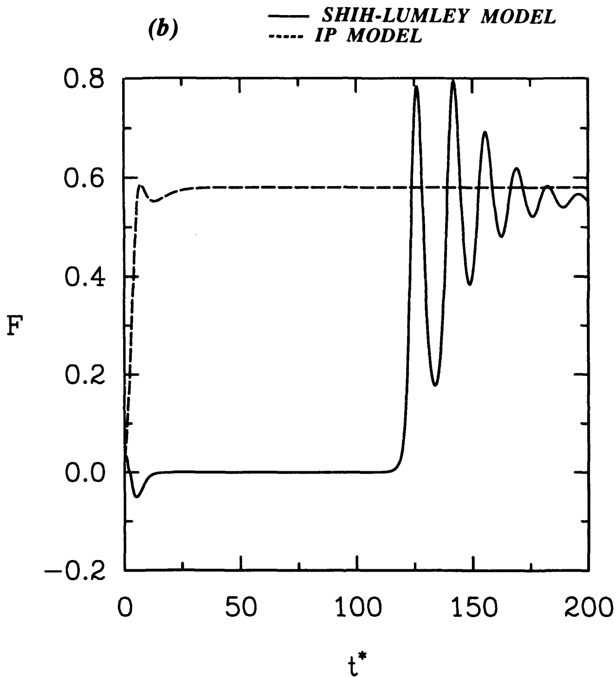
Figure 6. Computed results for homogeneous shear flow corresponding to the initial conditions (b_{11})_0 = -0.3 , (b_{22})_0 = -0.3 , SK_0/\epsilon_0 = 10 : (a) phase space trajectories of the Shih-Lumley Model, (b) time evolution of F and (c) time evolution of b_{12} .
