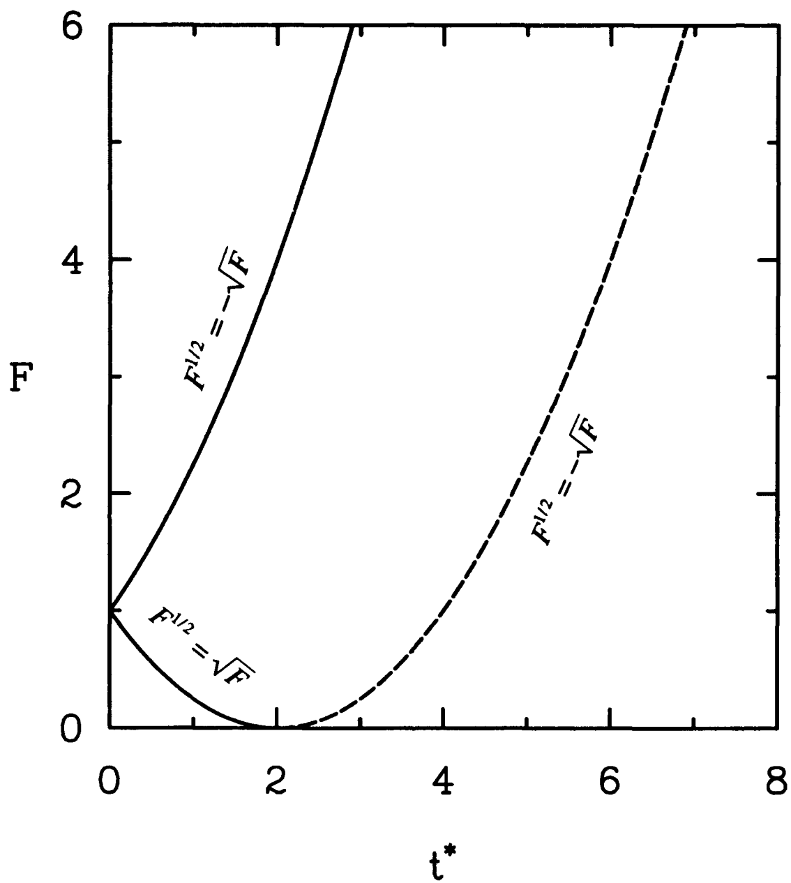
Figure 2. The two principal branches of the solution to the differential equation \dot{F} = -F^{1/2} with the initial condition F_0 = 1 .
