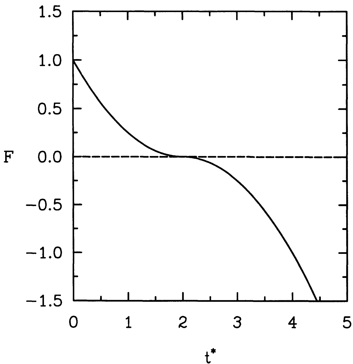
Figure 3. Numerical solution to the differential equation \dot{F} = -\sqrt{|F|} with the initial condition F_0 = 1 .
