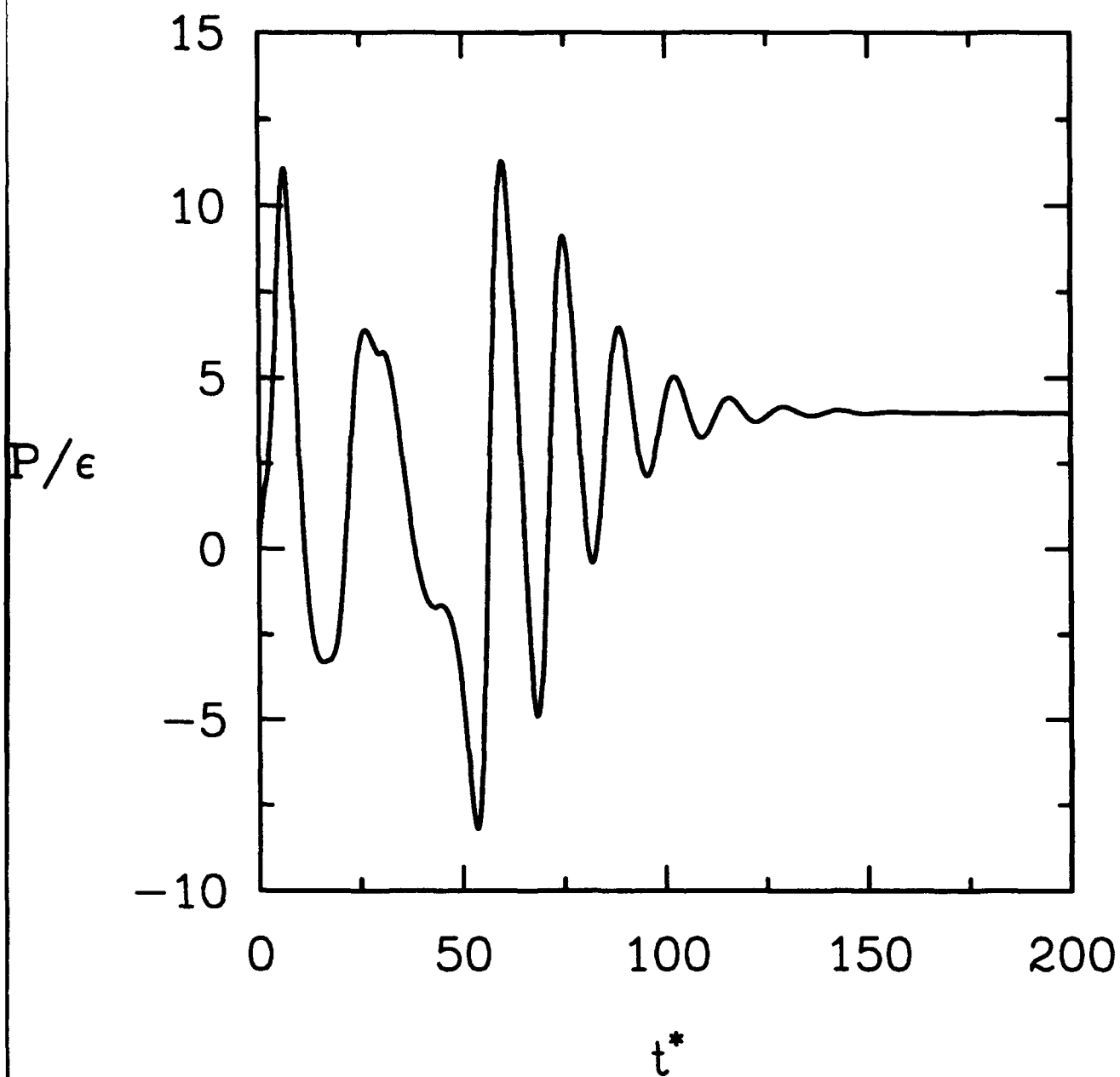
Figure 11. Computed model predictions for the time evolution of the ratio of production to dissipation ( \mathcal{P}/\epsilon ) in homogeneous shear flow corresponding to the initial conditions (b_{11})_0 = -0.32 , (b_{22})_0 = -0.32 , SK_0/\epsilon_0 = 50 : (a) IP Model, (b) Shih-Lumley Model and (c) the FLT Model.
