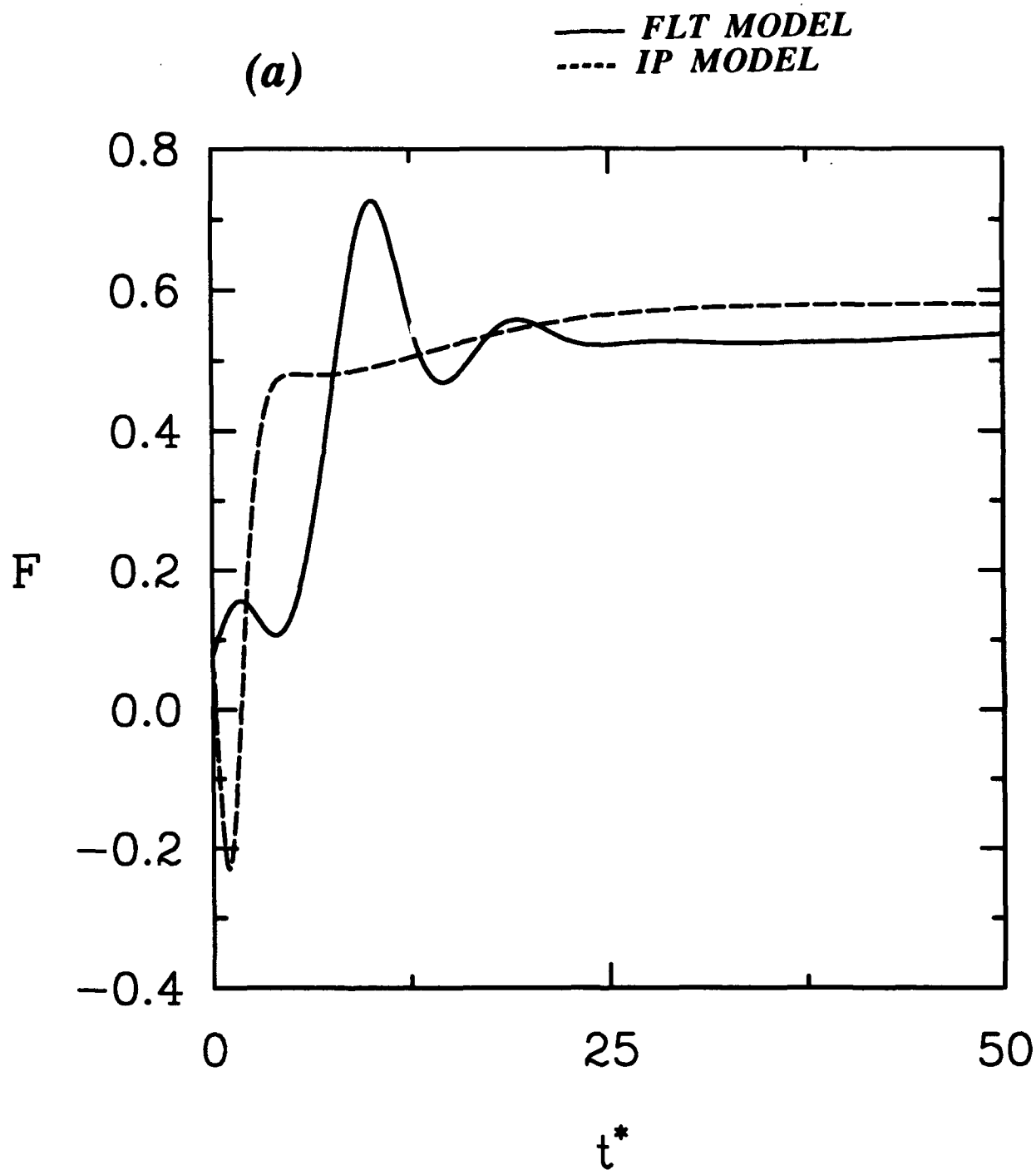
Figure 9. Model predictions for the time evolution of the Reynolds stress anisotropies in homogeneous shear flow corresponding to the initial conditions (b_{11})_0 = -0.24 , (b_{22})_0 = 0.17 , (b_{12})_0 = 0.2 , and SK_0/\epsilon_0 = 50 : (a) F and (b) b_{12} .
