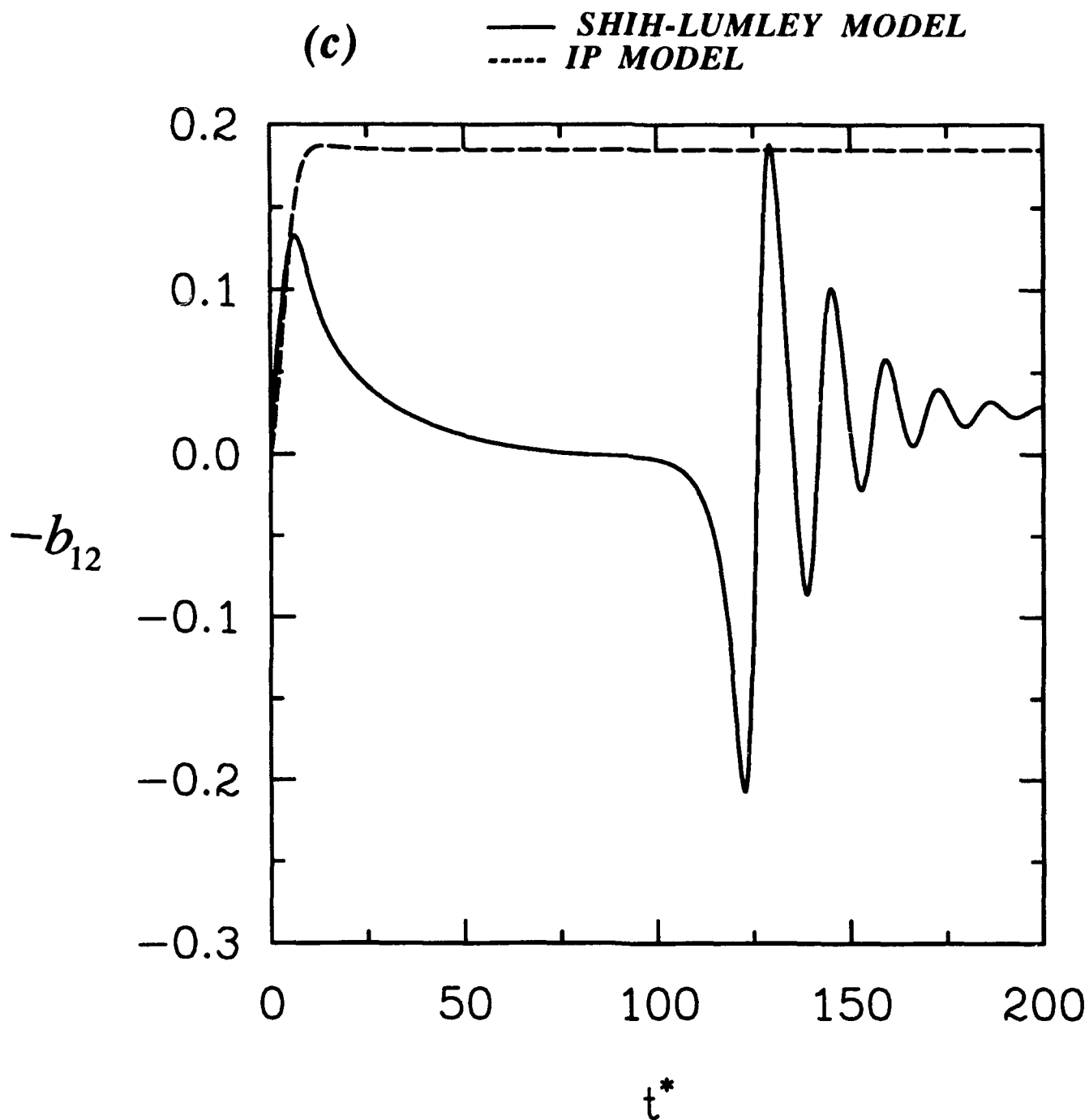
Figure 6. Computed results for homogeneous shear flow corresponding to the initial conditions (b_{11})_0 = -0.3 , (b_{22})_0 = -0.3 , SK_0/\epsilon_0 = 10 : (a) phase space trajectories of the Shih-Lumley Model, (b) time evolution of F and (c) time evolution of b_{12} .
