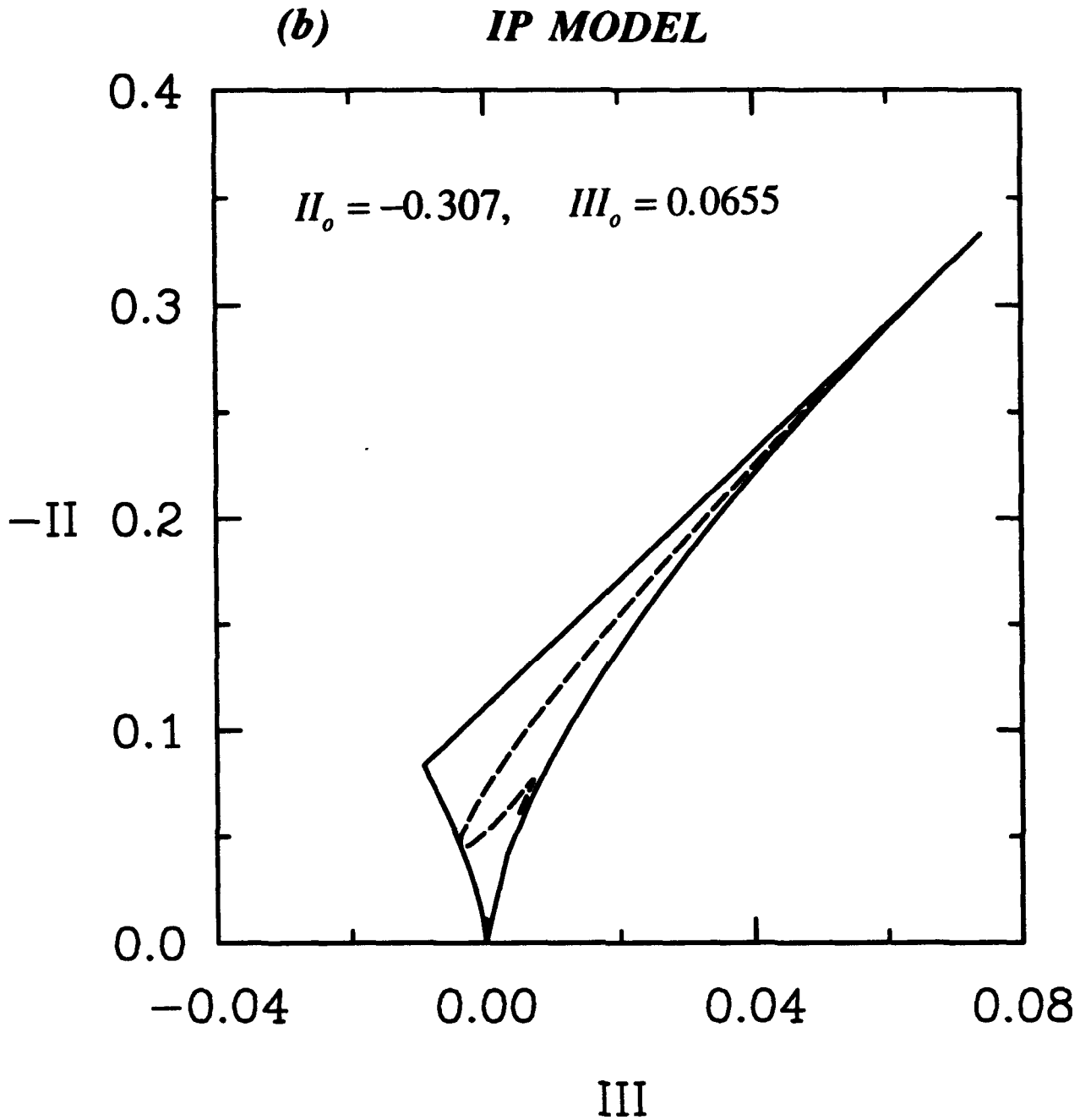
Figure 4. Computed phase space trajectories in homogeneous shear flow for the initial conditions (b_{11})_0 = -0.32 , (b_{22})_0 = -0.32 , SK_0/\epsilon_0 = 50 : (a) Shih-Lumley Model and (b) the IP Model of Launder and co-workers.
