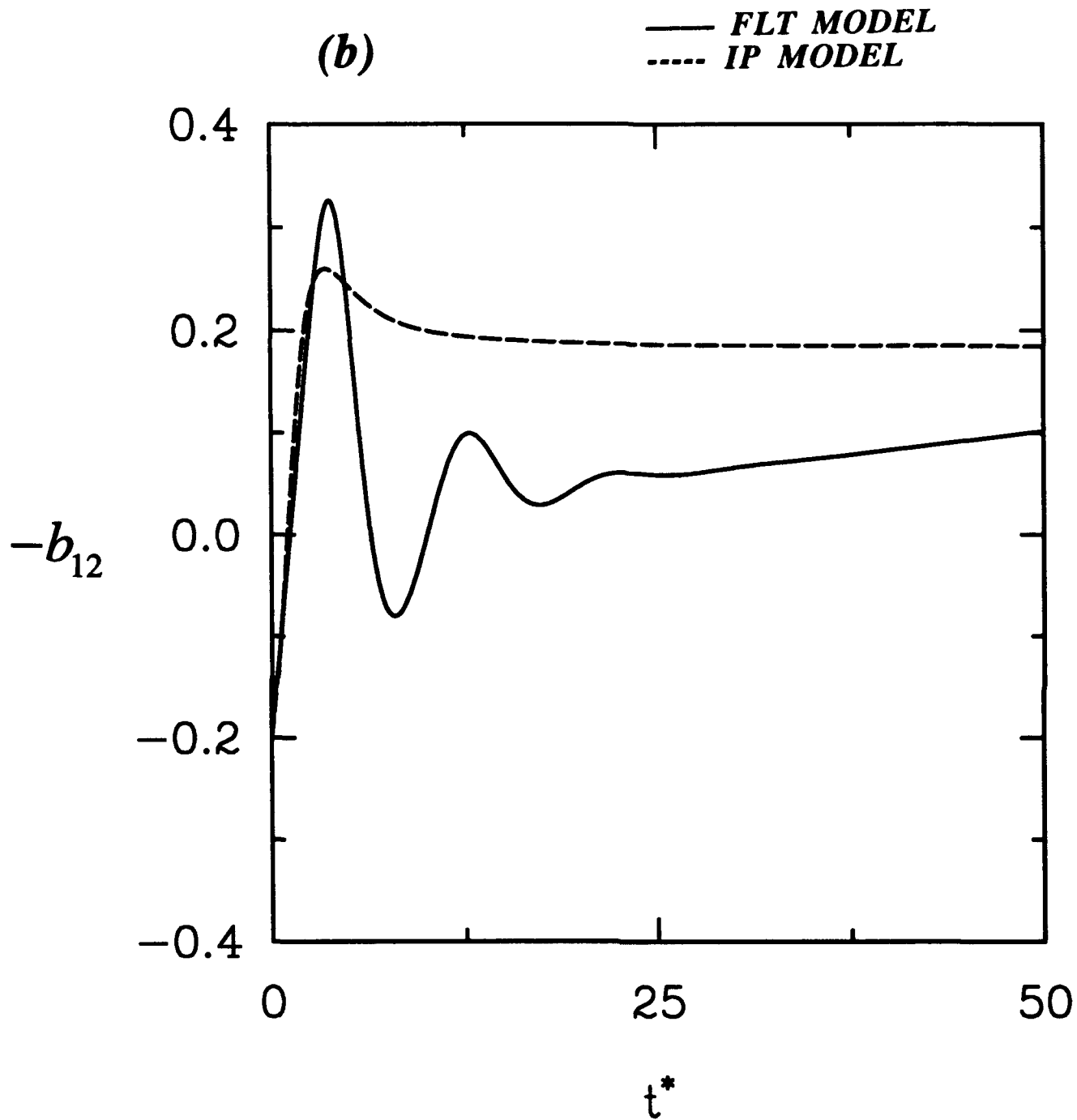
Figure 9. Model predictions for the time evolution of the Reynolds stress anisotropies in homogeneous shear flow corresponding to the initial conditions (b_{11})_0 = -0.24 , (b_{22})_0 = 0.17 , (b_{12})_0 = 0.2 , and SK_0/\varepsilon_0 = 50 : (a) F and (b) b_{12} .
