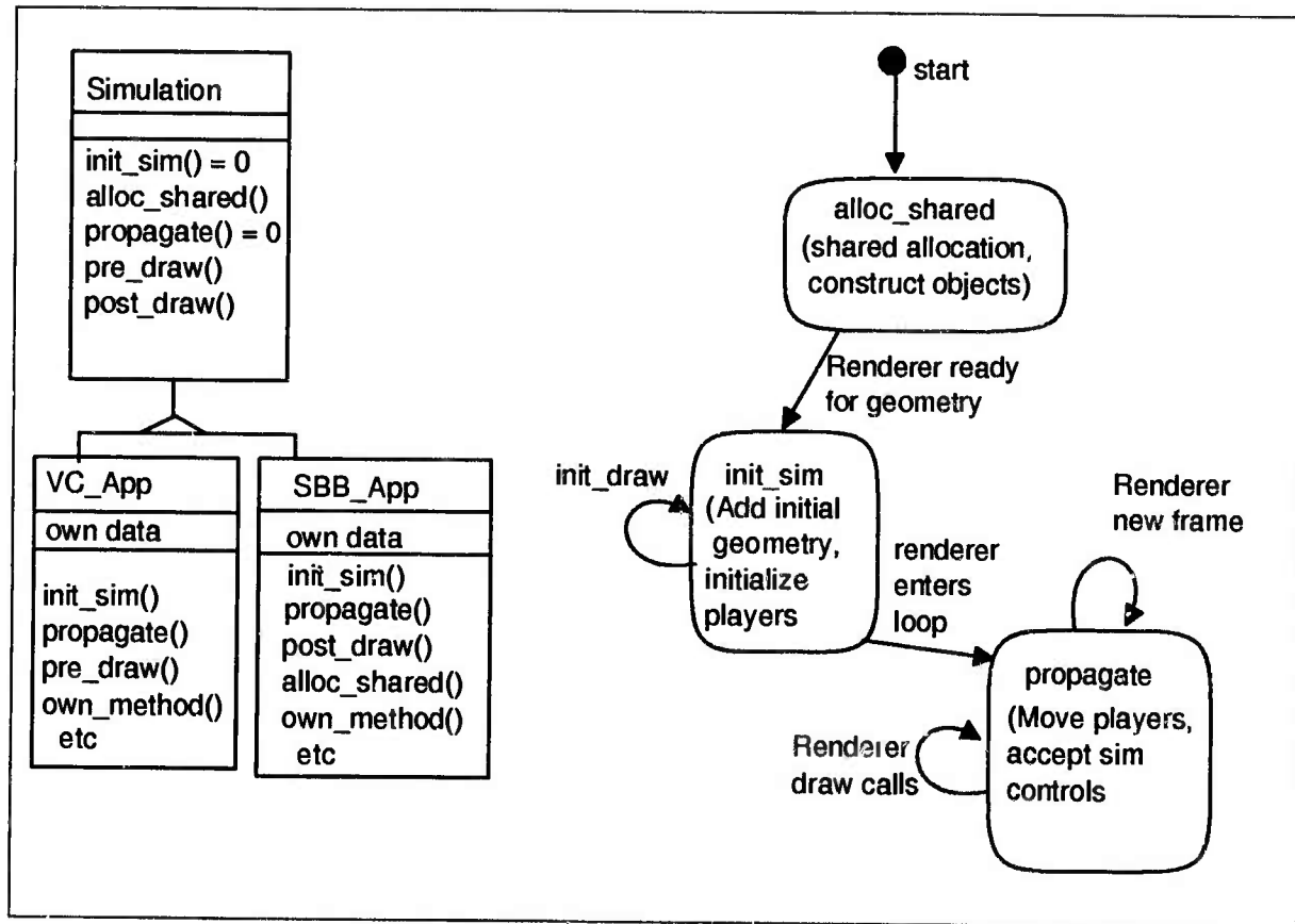
Figure 14 - Simulation Class Diagrams
