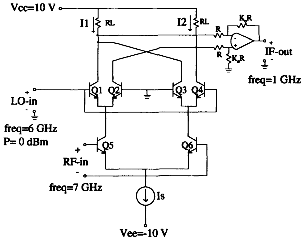
Figure 33. Gilbert multiplier cell.
