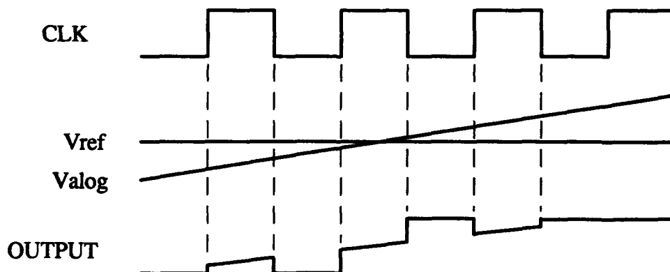
Figure 26. Operational diagram of comparator operation.
