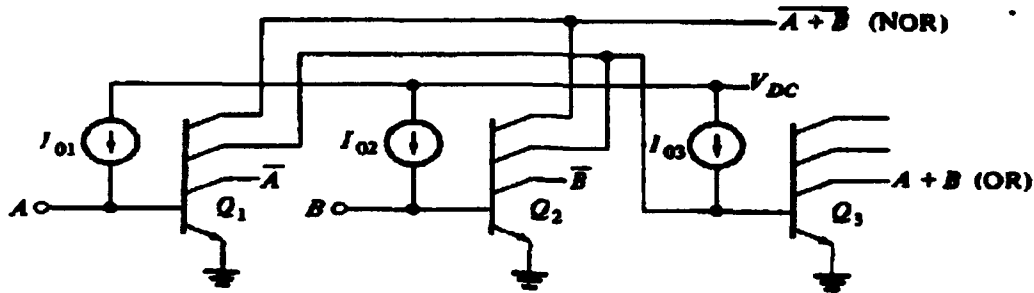
Figure 3. A simple current switch using ECL logic [11].
