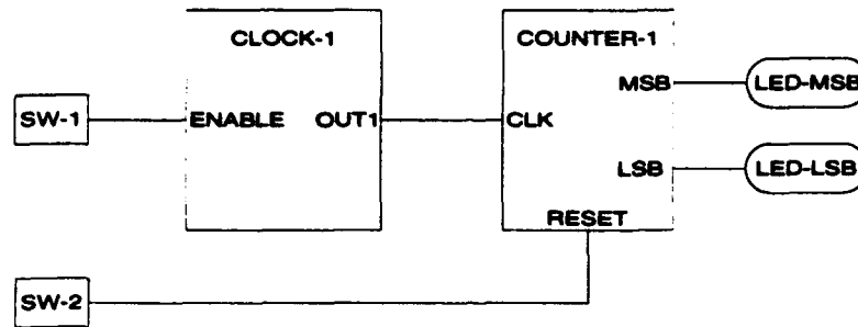
Figure 13. Counter Test
