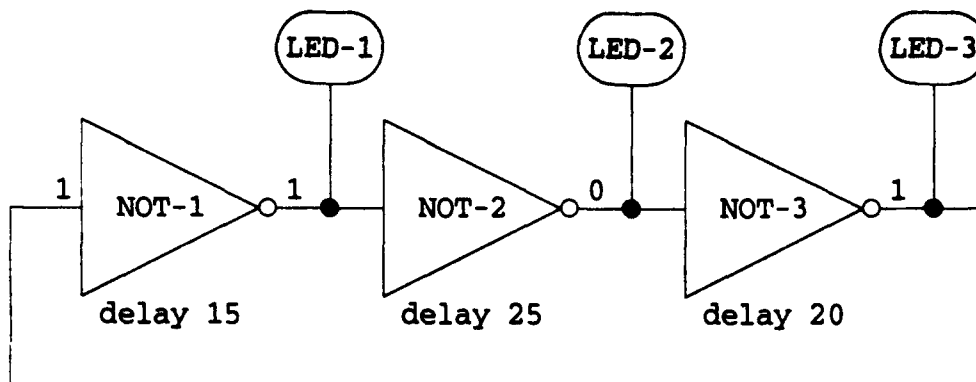
Figure 14. Simple Oscillator
