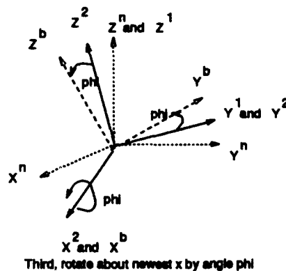
Figure 28. Euler Angle Body Axis Rotations
