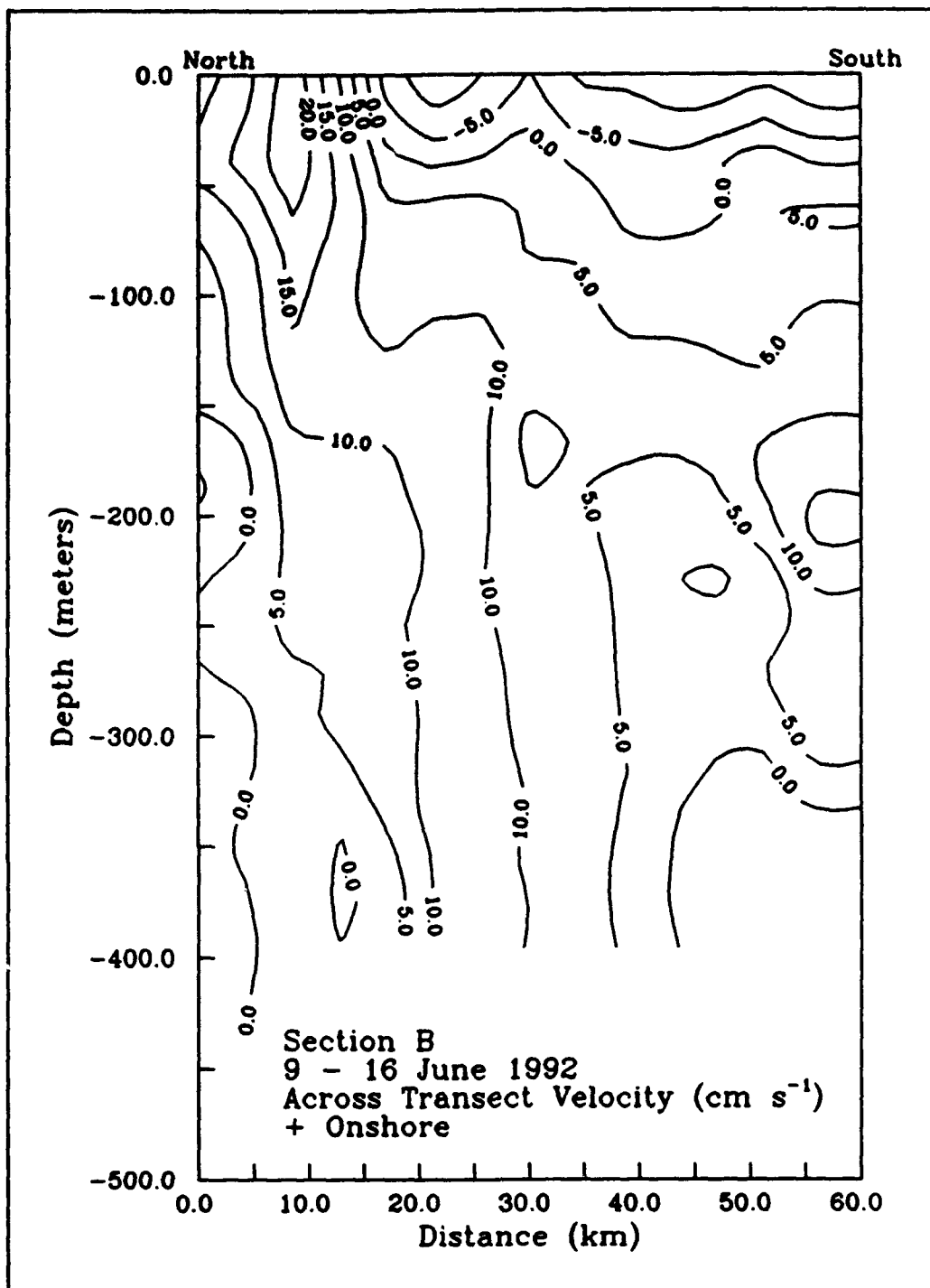
Figure 34. Vertical sections of 5 km averaged a) across-transect and b) along-transect ADCP velocity ( \text{cm s}^{-1} ) for section B of the Eastern Boundary Current Accelerated Research Initiative cruise of June 9-16, 1992 aboard the R/V POINT SUR.
