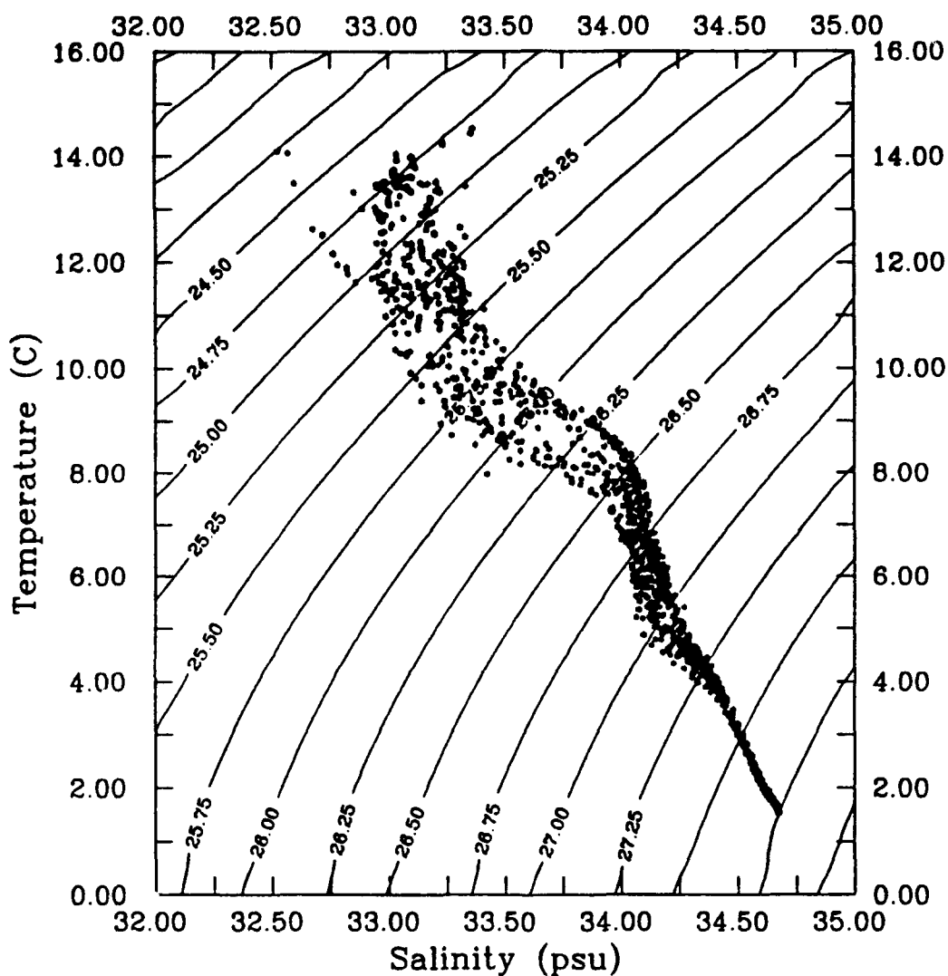
Figure 44. T/S diagram which includes data from all CTD stations completed during the Eastern Boundary Current Accelerated Research Initiative cruise of June 9-16, 1992 aboard the R/V POINT SUR. The data included in this diagram consists of all data listed in Appendix A.
