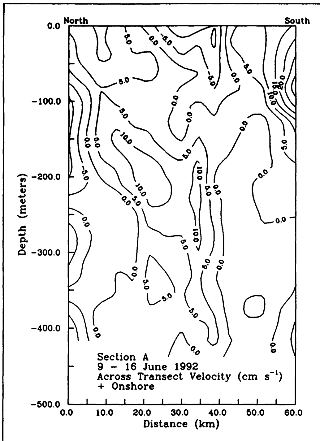
Figure 33. Vertical sections of 5 km averaged a) across-transect and b) along-transect ADCP velocity ( \text{cm s}^{-1} ) for section A of the Eastern Boundary Current Accelerated Research Initiative cruise of June 9-16, 1992 aboard the R/V POINT SUR.
