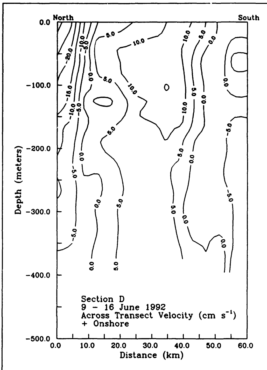
Figure 36. Vertical sections of 5 km averaged a) across-transect and b) along-transect ADCP velocity ( \text{cm s}^{-1} ) for section D of the Eastern Boundary Current Accelerated Research Initiative cruise of June 9-16, 1992 aboard the R/V POINT SUR.
