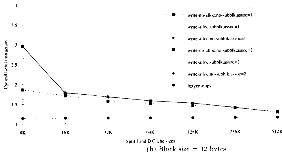
Figure 11: Lexgen summary
