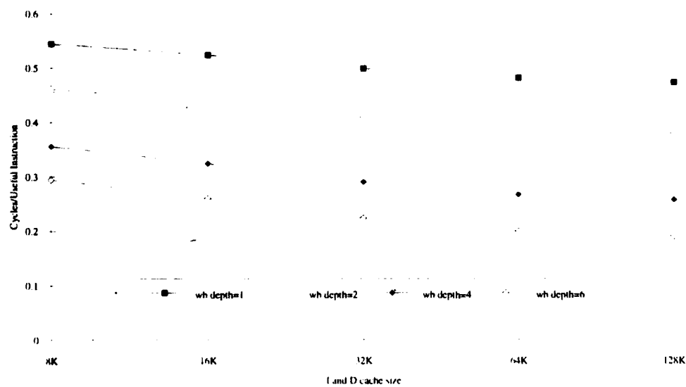
(b) Associativity = 2
