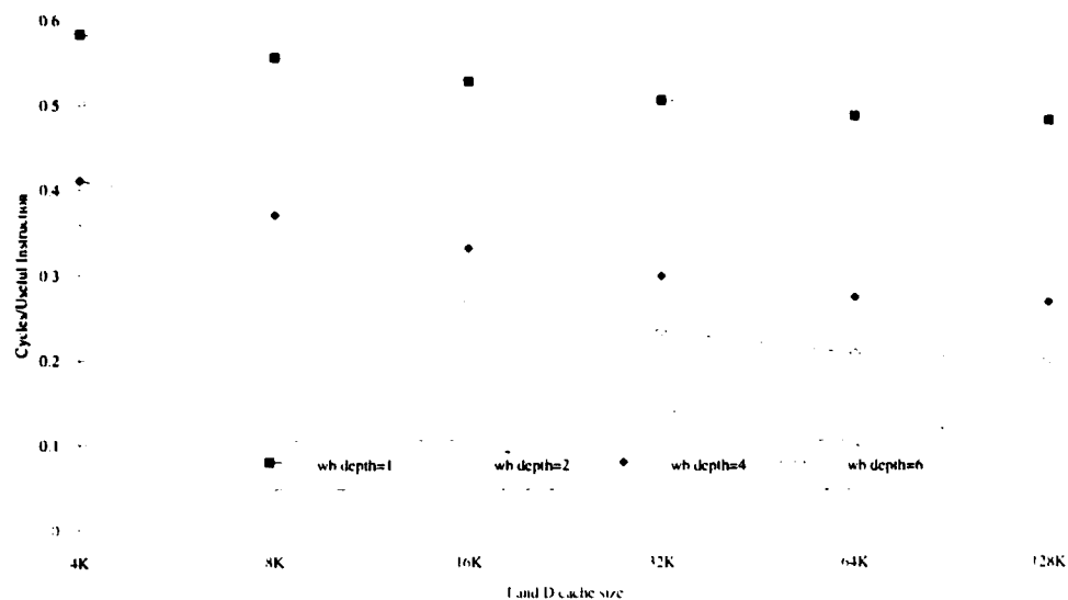
(a) Associativity = 1
