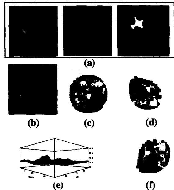
Figure 6 : Matching between a complete model and a partial view: (a) Original images measured from three different views; (b) Image of partial view; (c) Mesh of complete model mapped hue values; (d) Mesh of partial model mapped hue values; (e) Matching using color and curvature; (f) Transformed mesh using the matching result;
