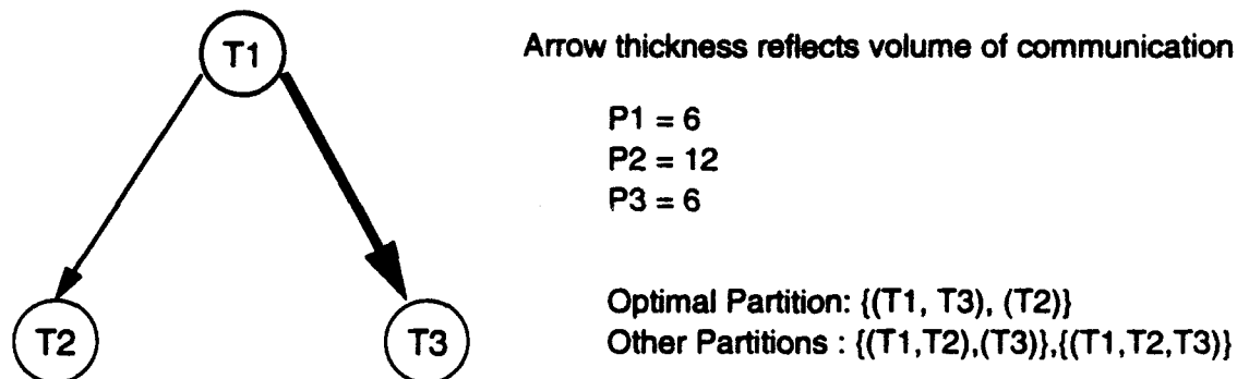
Figure 4: Partitioning a task graph into modules
