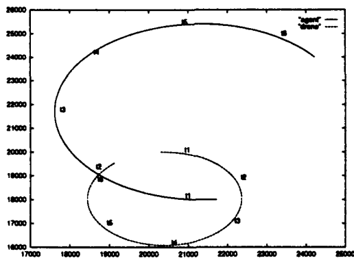
Figure 5.14 Scenario #2, standard agent. Two- and three-dimensional behavior of standard agent at close range.
