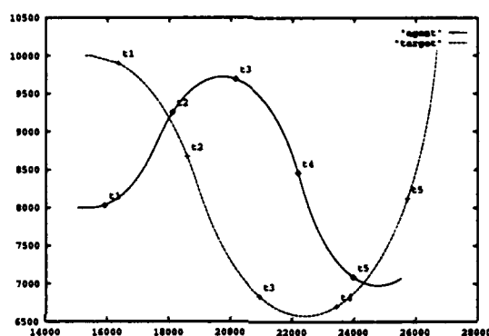
Figure 1.1 An example of inappropriate MAXIM behavior. In this scenario the agent overshoots the target and loses the opportunity to achieve a positional advantage.
