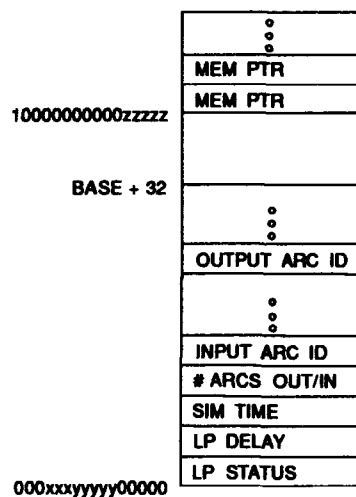
Figure 23. SRAM Memory Map for DES Coprocessor
