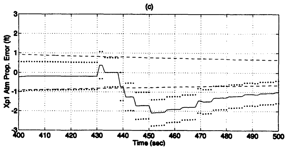
Plot I-8: RRS Range bias/Velocity bias/Atmospheric propagation delay Errors
