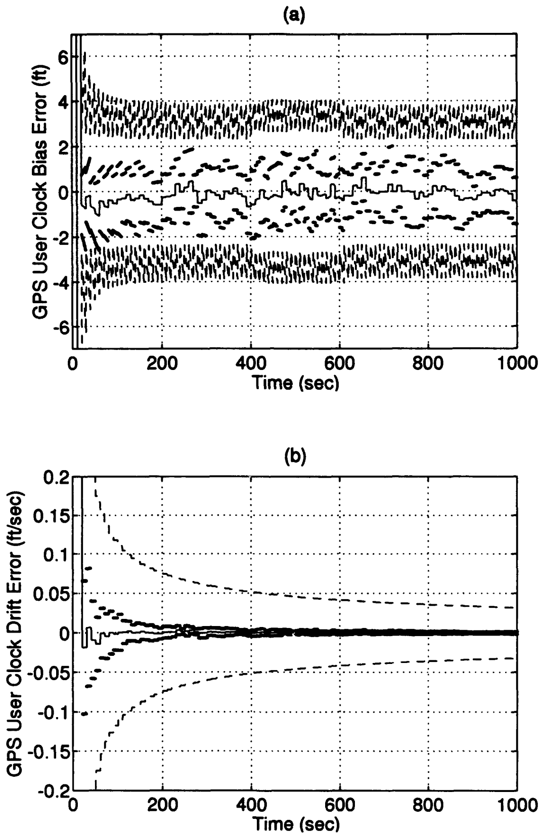
Plot G-8: GPS User Clock Bias/Drift Errors
