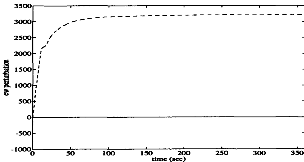
Figure 5.15 C-130A: Nonlinear Simulation, Response To A 100 ft Step Altitude Change: Energy Conserving Implementation (solid line) and Energy Excursion Minimizing Implementation (dashed line)
