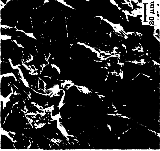
Torsion With Axial Compression
