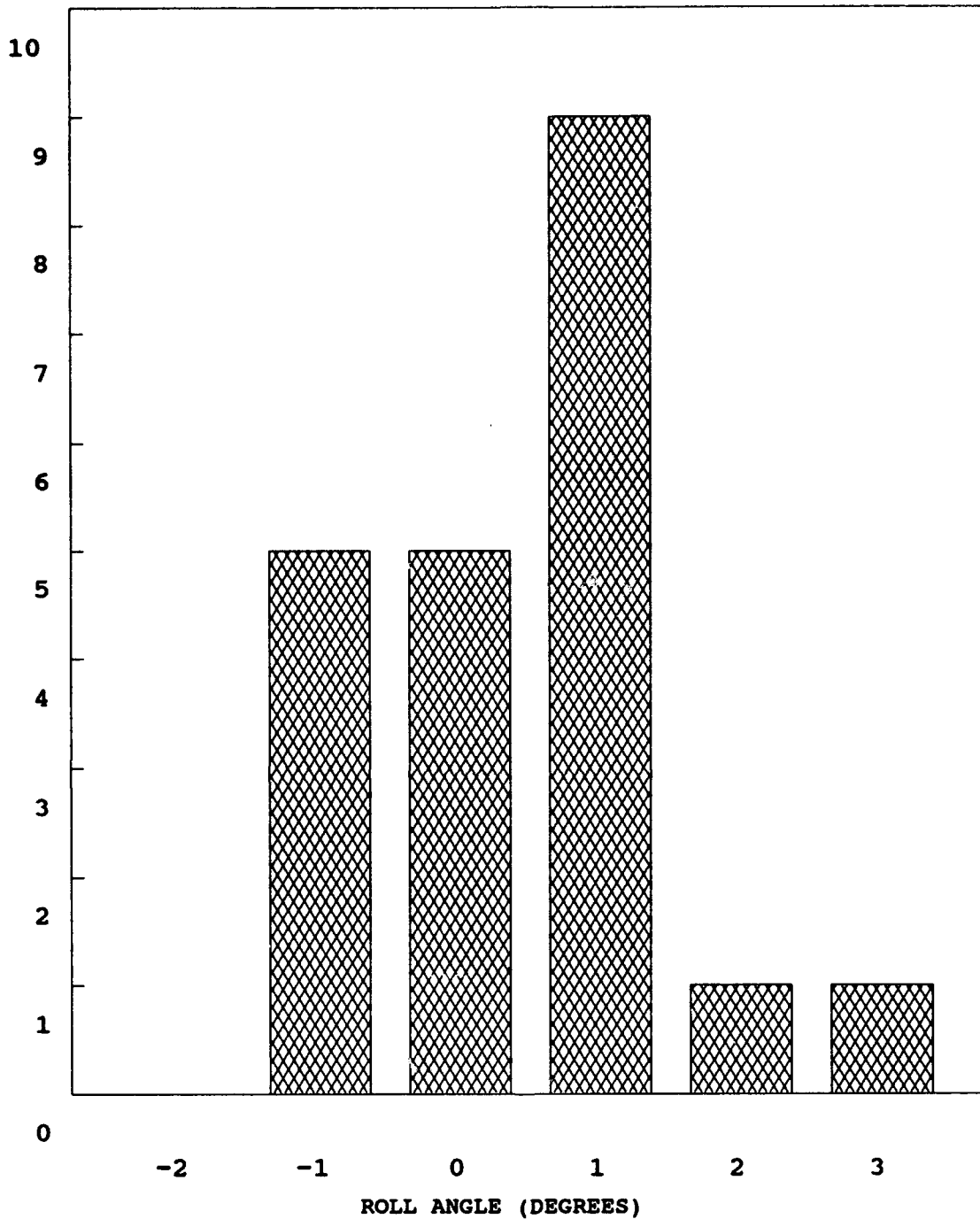
FIGURE 9. LANDING LOADS DATA COLLECTION PROGRAM FAA TECHNICAL CENTER B-727-100 LANDINGS NUMBER OF LANDINGS VERSUS ROLL ANGLE
