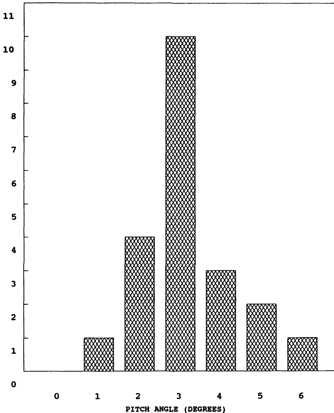
FIGURE 8. LANDING LOADS DATA COLLECTION PROGRAM FAA TECHNICAL CENTER B-727-100 LANDINGS NUMBER OF LANDINGS VERSUS PITCH ATTITUDE
