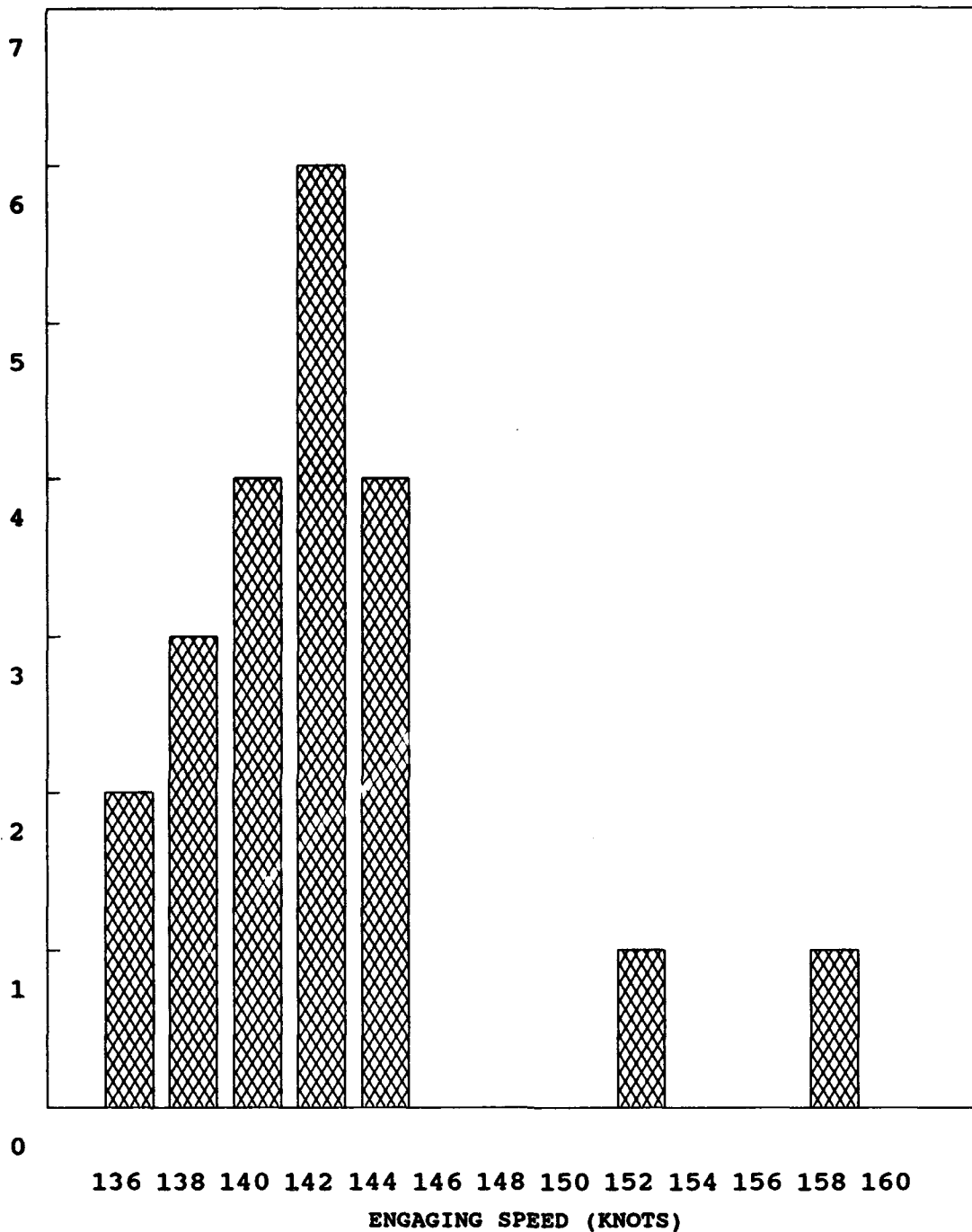
FIGURE 7. LANDING LOADS DATA COLLECTION PROGRAM FAA TECHNICAL CENTER B-727-100 LANDINGS NUMBER OF LANDINGS VERSUS ENGAGING SPEED
