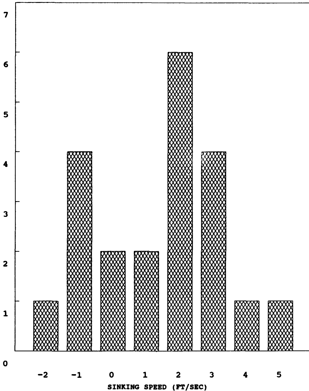
FIGURE 6. LANDING LOADS DATA COLLECTION PROGRAM FAA TECHNICAL CENTER B-727-100 LANDINGS NUMBER OF LANDINGS VERSUS SINK SPEED
