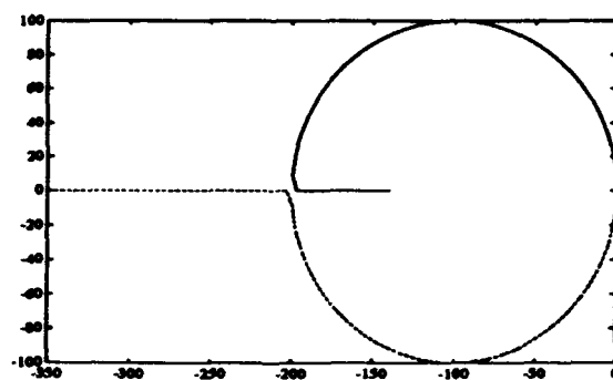
Figure 4. Open Loop Poles and Zeros for SKM Beam.
