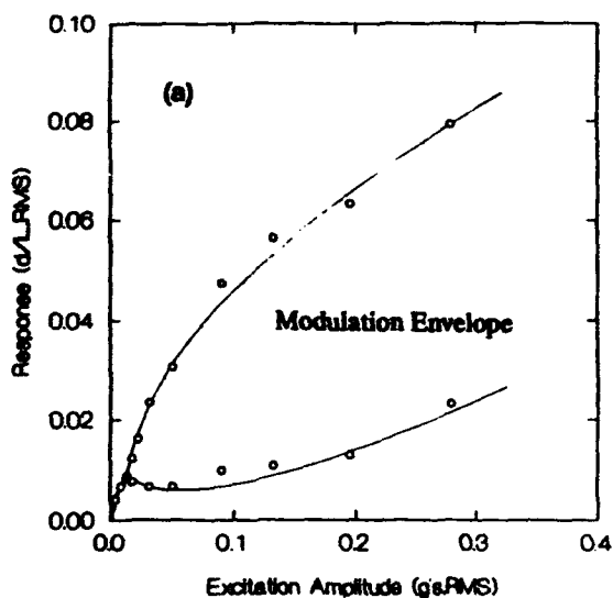
Figure 12. First mode amplitude response of the 2DOF structure with +0.20% detuning and no damping treatment for a direct excitation to the first mode at a frequency of 1.004. This frequency corresponds to the modulation region in Figure 10. The curves approximate the bounds on the modulation. The second mode amplitude is qualitatively similar.
