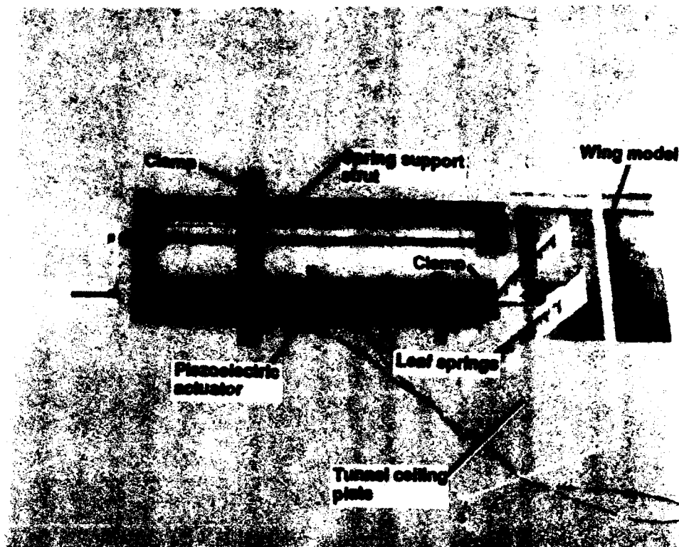
Figure 3. - Wind-tunnel model and support system.
