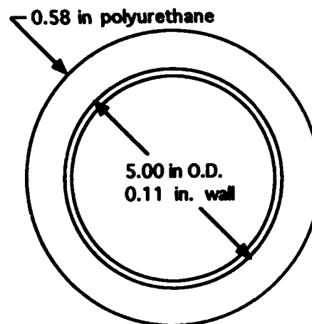
Fig. 9 — Unconstrained layer damping ring test specimen.
