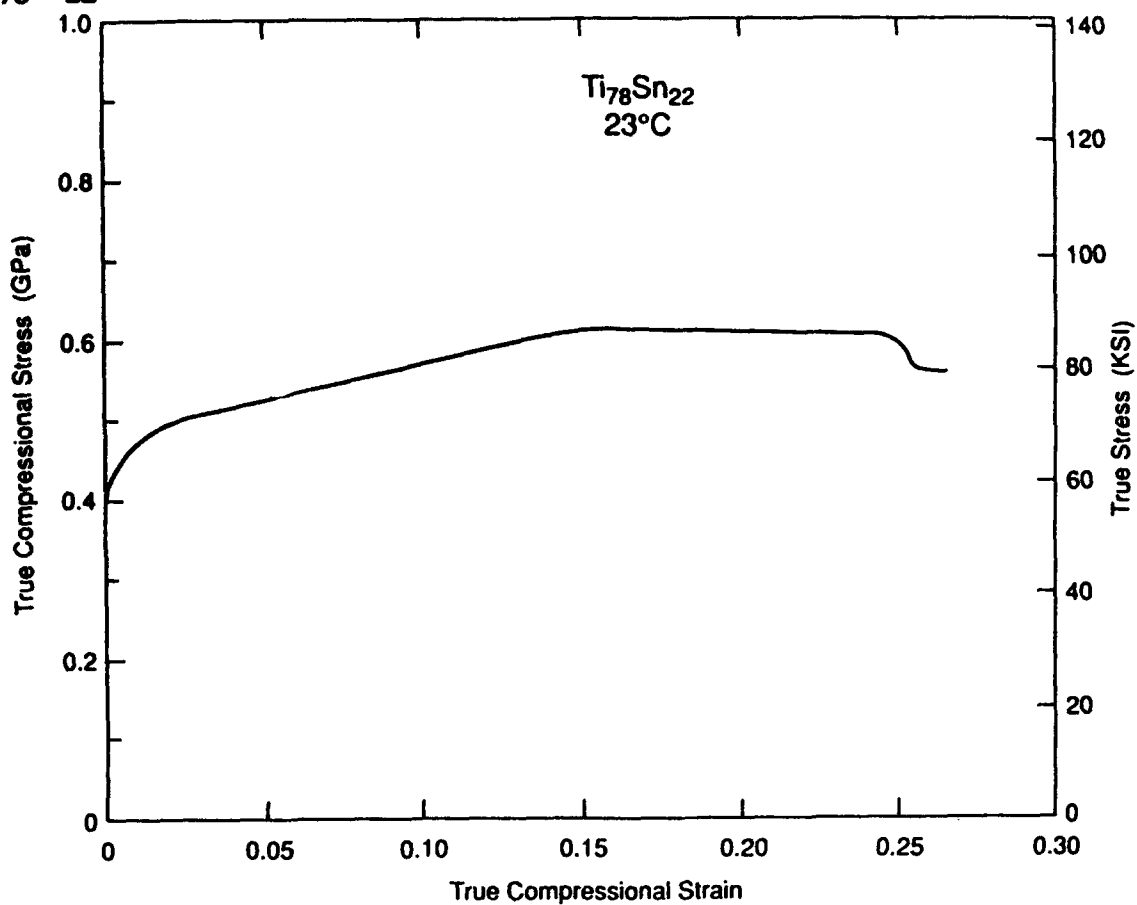
FIG. 6 Stress-Strain Curve For Compressional Room-Temperature Deformation of \text{Ti}_{78}\text{Sn}_{22}
