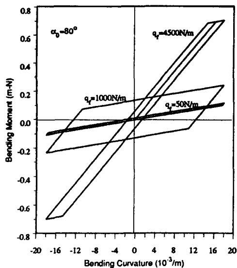
Figure 12 Moment-curvature relationship in bent cables with various friction forces.
