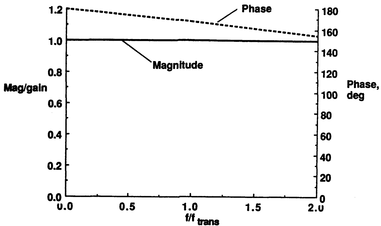
Figure 9.- Transfer function.
