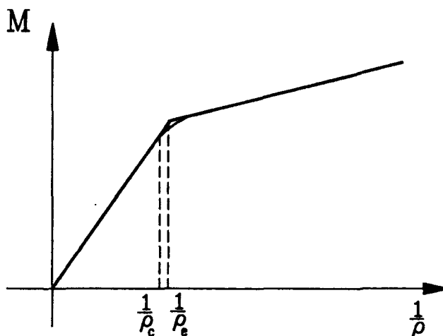
Figure 9 Approximation of the bending-curvature relation as a piece-wise linear function.
