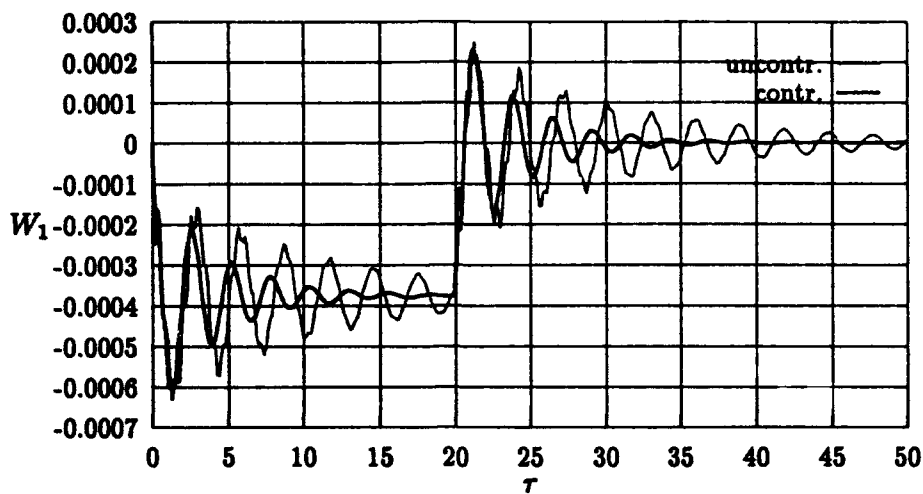
Figure 8: Tip torsional rotation response to a rectangular gust with and without control.
