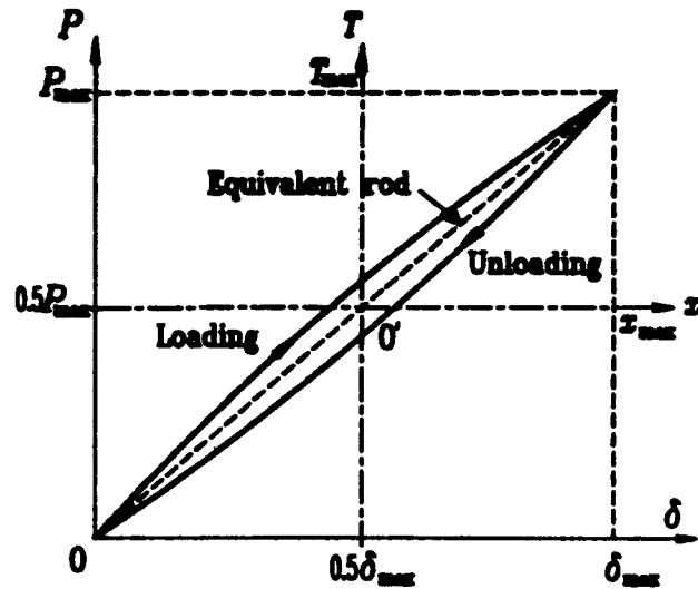
Figure 5 Hysteretic loop from the cable.
