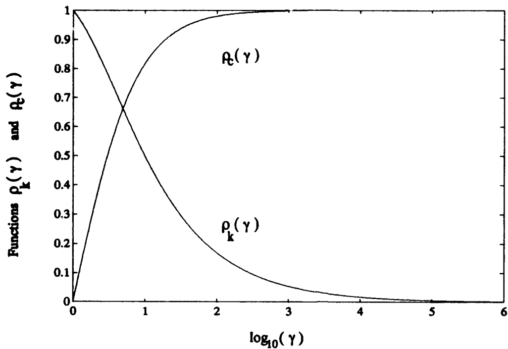
Figure 6. Functions \rho_k(\gamma) and \rho_c(\gamma) (harmonic linearization).
