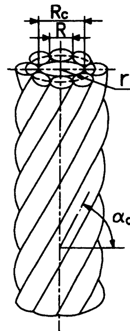
Figure 1 A six-wire cable.
