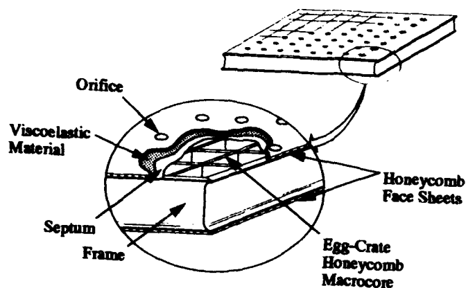
Figure 12. 1.8 m by 1.8 m Panel Fabricated and Tested in 1990
