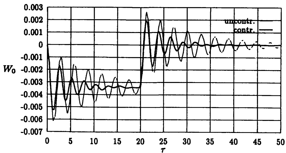
Figure 7: Tip displacement response to a rectangular gust with and without control.
