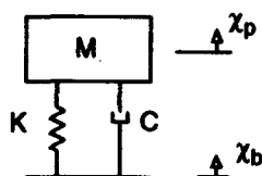
Fig. 2 Passive Second-order Isolator Schematic
