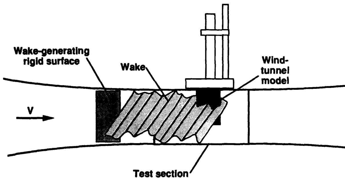
Figure 7. - Wake generator.
