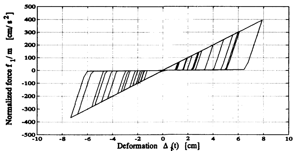
Figure 9. Comparison of the response of a 2DOF nonlinear structure and its linearization.
