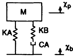
Fig. 5 Third-order Isolator Schematic
