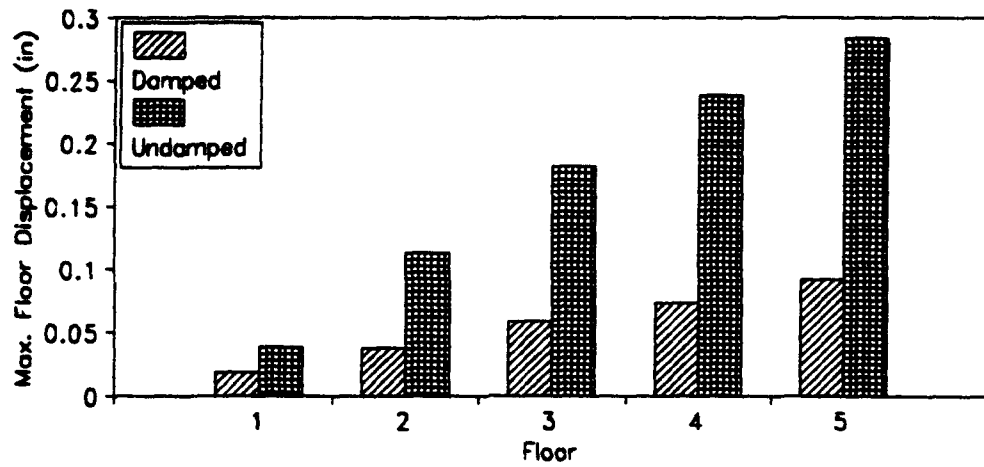
Fig. 8 Max Floor Disp. (0.06 El Centro)
