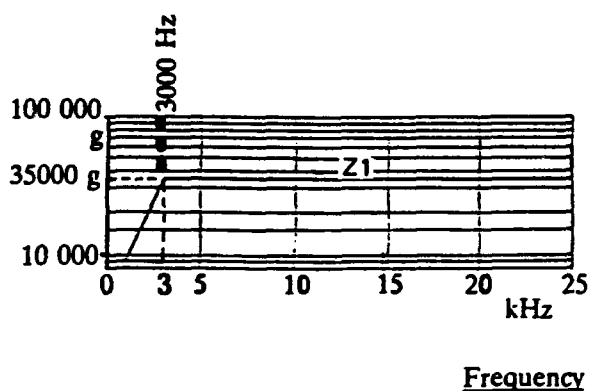
Fig. 5: ARIANE 5, specified shock response spectrum for Zone "Z1"
