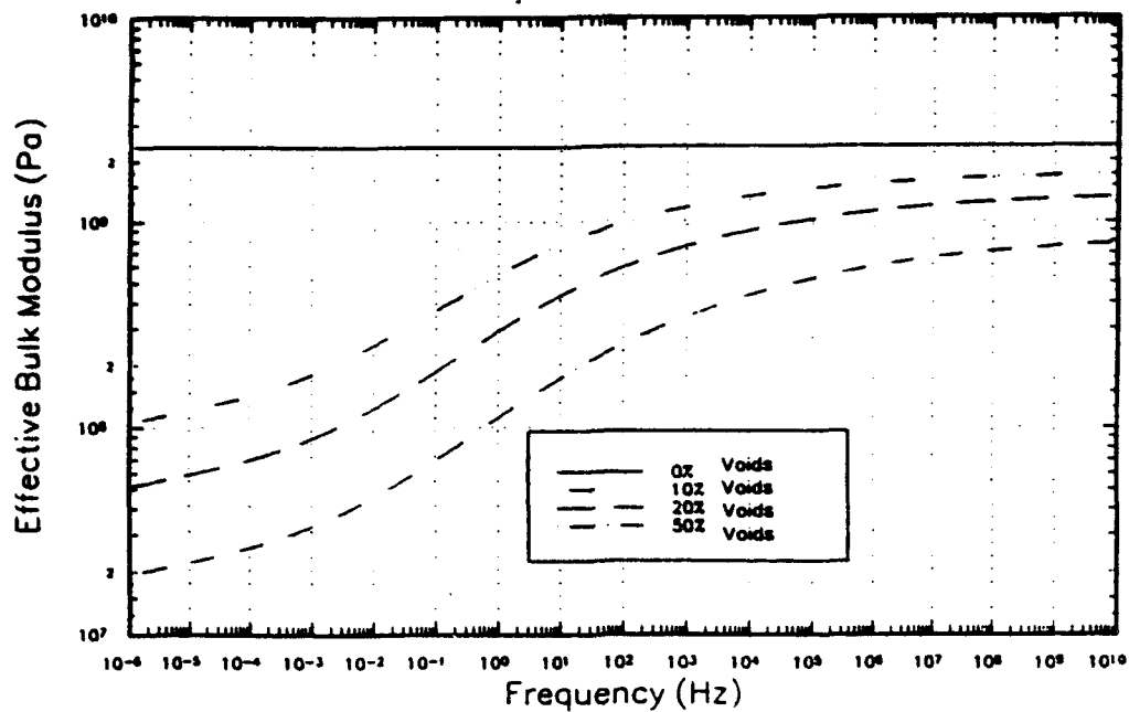
Figure 11. Effective bulk modulus of a voided urethane
