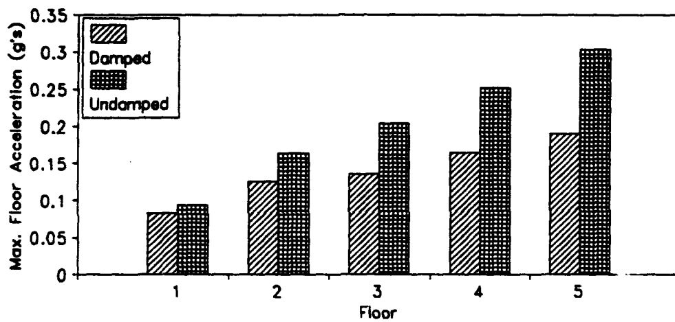
Fig. 9 Max Acceleration (0.06 El Centro)
