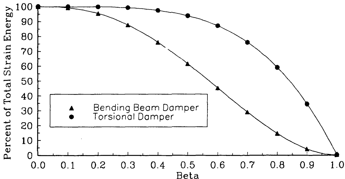
Fig. 4 Percent Strain Energy vs Strain Range \beta
