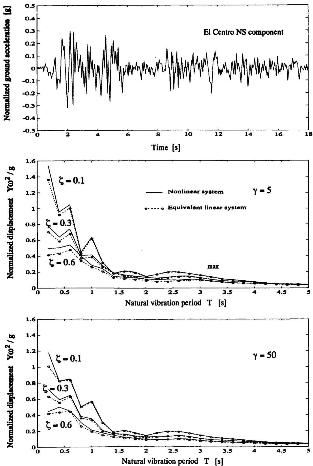
Figure 8. Ground motion signal and deformation response spectra for \gamma = 5 and \gamma = 50
