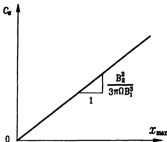
Figure 8 Damping-elongation relation.
