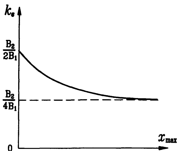
Figure 7 Stiffness-elongation relation.
