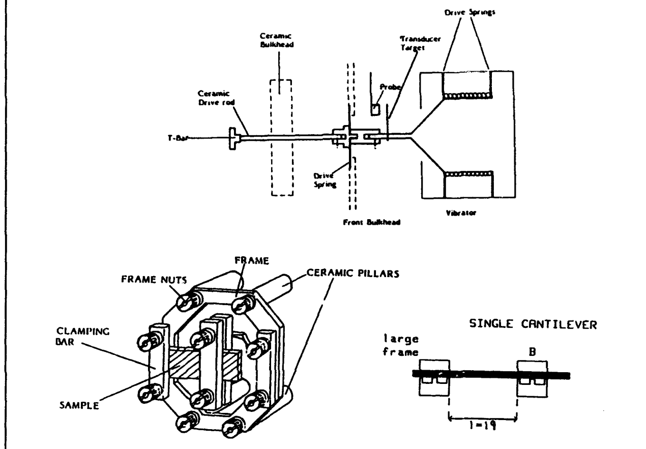
FIG. 1. Dynamic Mechanical Thermal Analyzer: grip setup.
