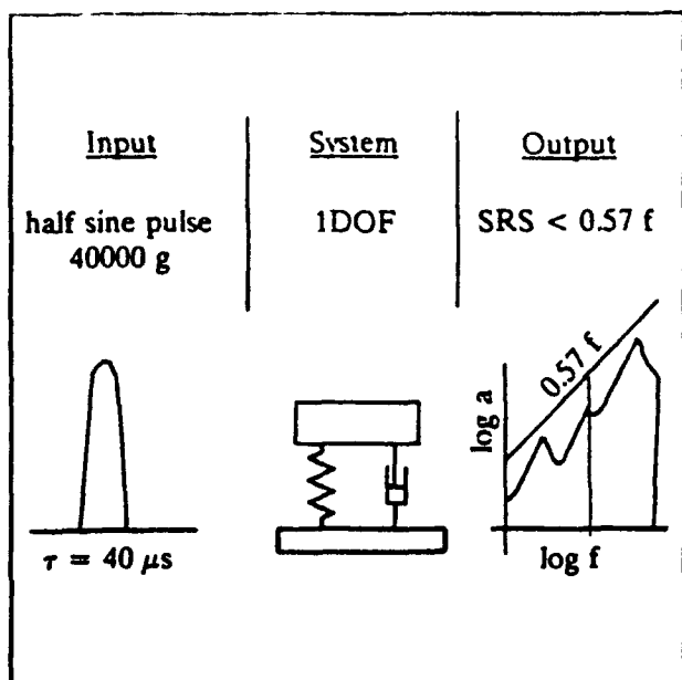
Fig. 7: Input/Output requirement
