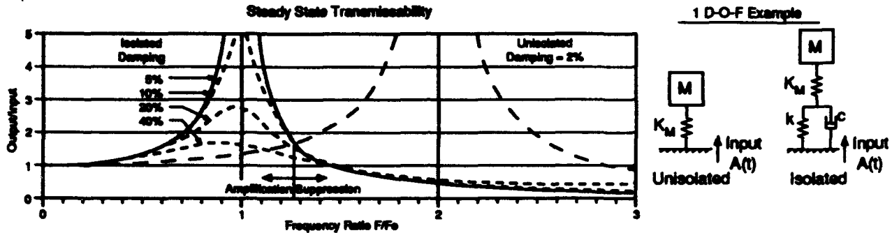
Fig. 4. Steady-state Transmissibility
