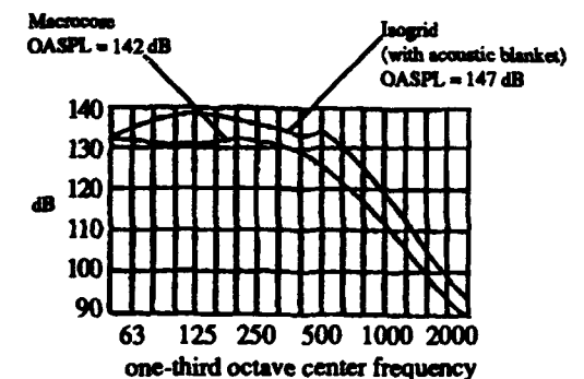
SEA noise prediction performed by Cambridge Collaborative Inc., Figure 14. Predicted Shroud Interior Noise Levels
