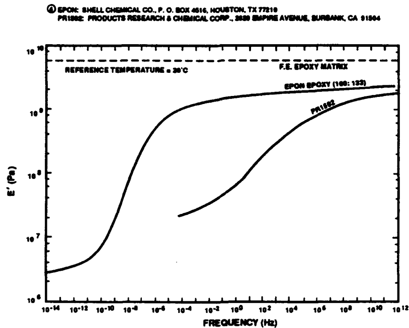
Figure 7. Moduli of EPON ® epoxy and PR 1592 polyurethane 4
