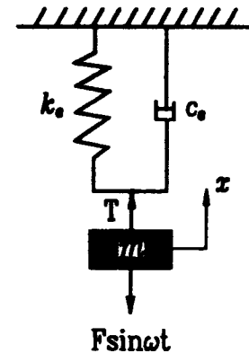
Figure 6 SDOF model.
