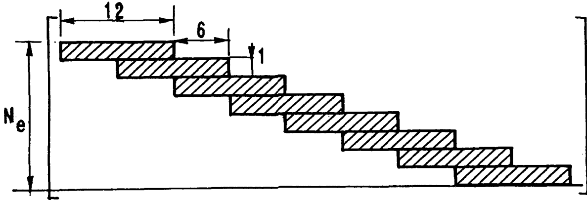
Figure 2: Block structure of the transpose of the matrices P and B .
