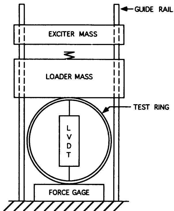
Fig. 14 — Principle of operation of the dynamic tester.
