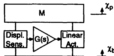
Fig. 9 Active Fourth-order Isolator Schematic
