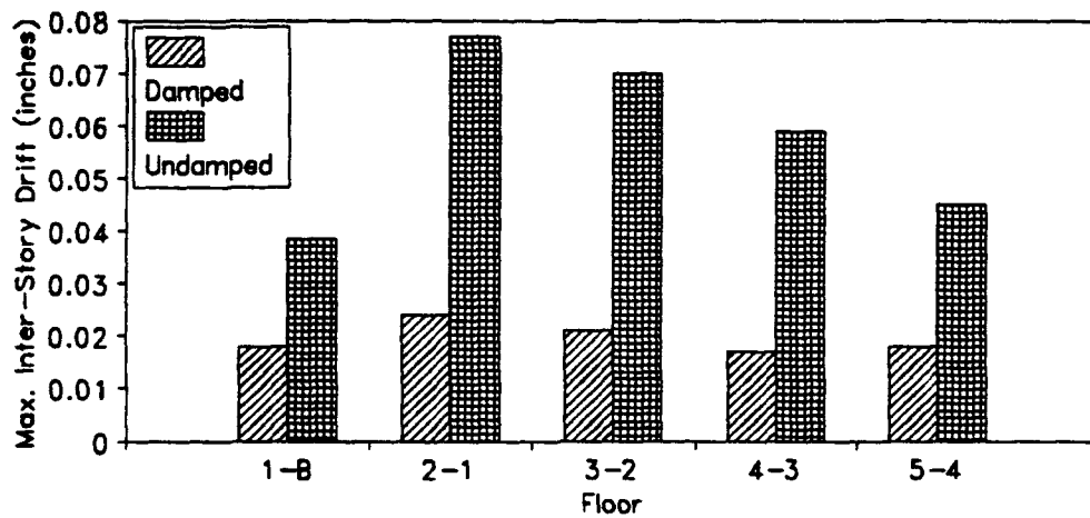
Fig. 10 Max Inter-Story Drift (0.06 El Centro)
