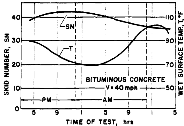
Figure 14. Influence of Hourly Changes in Wet Surface Temperatures on Steady-State Skid Number (Kummer and Meyer [12])
