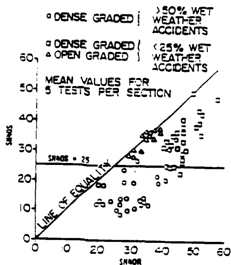
Figure 10. Skid Numbers SN40R (ribbed tire) and SN40S (smooth tire) Measured at Accident Sites in Florida: Mean Values for Five Tests per Section (Henry and Wambold [2])
