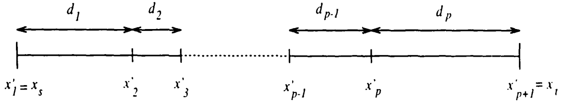
Figure 1: Illustration of reformulation 1. Each segment i defines a cut between nodes on the left of the segment and the nodes on the right. The value of this cut is t_i .
