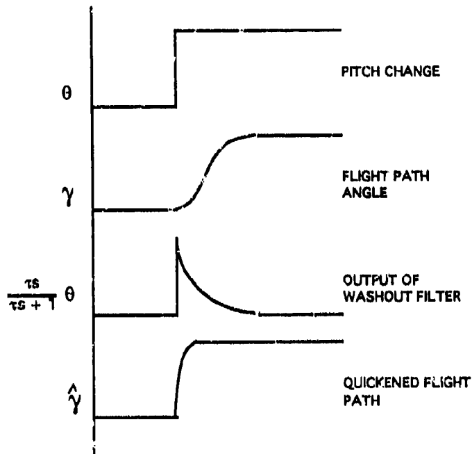
Figure B- 4. Effect of washout filter on flight path. The pitch change is the input to the filter. The output from the filter is added to the actual flight path to produce the quickened flight path. These curves are idealized responses to a step change in pitch.
