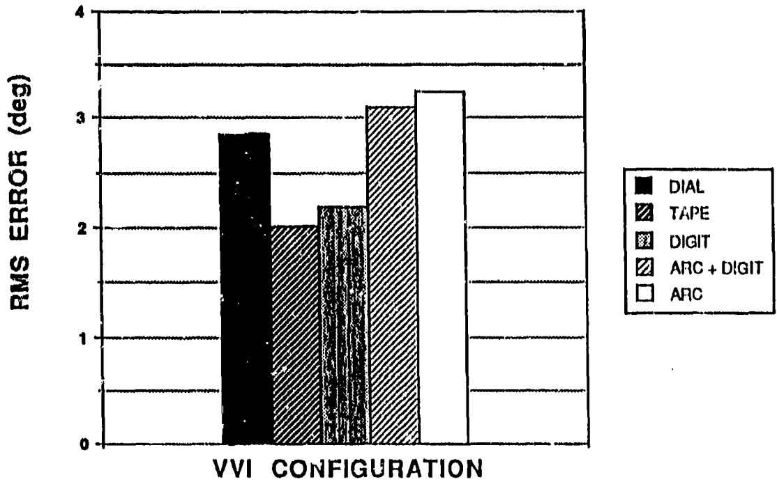
Figure 16. The RMSE in bank as a function of VVI configuration.
