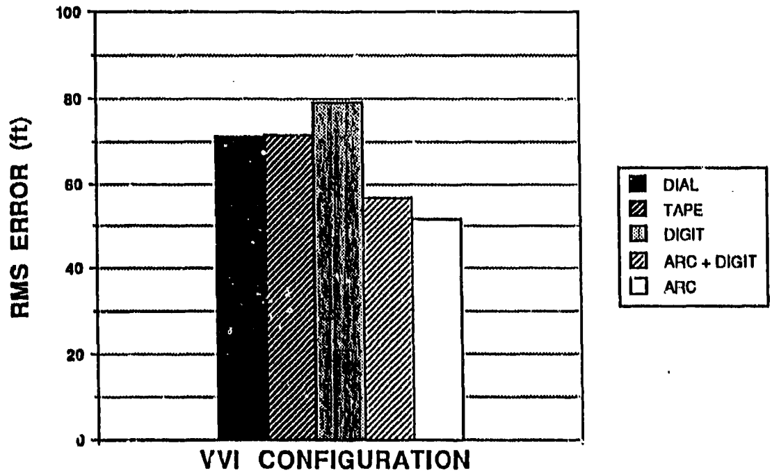
Figure 15. The RMSE altitude for the five VVI configurations during the straight and level task with perturbations.
