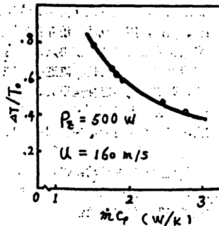
Figure 1: Relationship between temperature rise \Delta T and mass flow m
