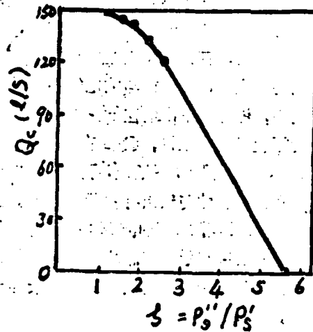
Figure 4: Effect of pressure ratio \zeta on fan speed Q_c .
