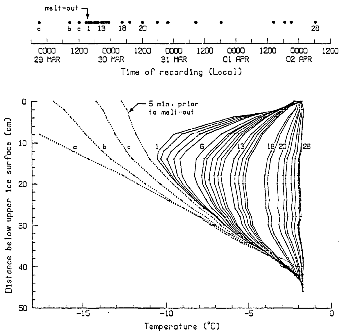
Figure 56. Temperature profiles in the submerged ice block during the 3 days it took for the block to warm to the temperature of the water. The four profiles taken prior to melt-out are shown as dotted lines in Figure 36. As in Figure 36, several profiles are labeled by run number after submergence. The graph at the top of the figure associates run number with local time.
