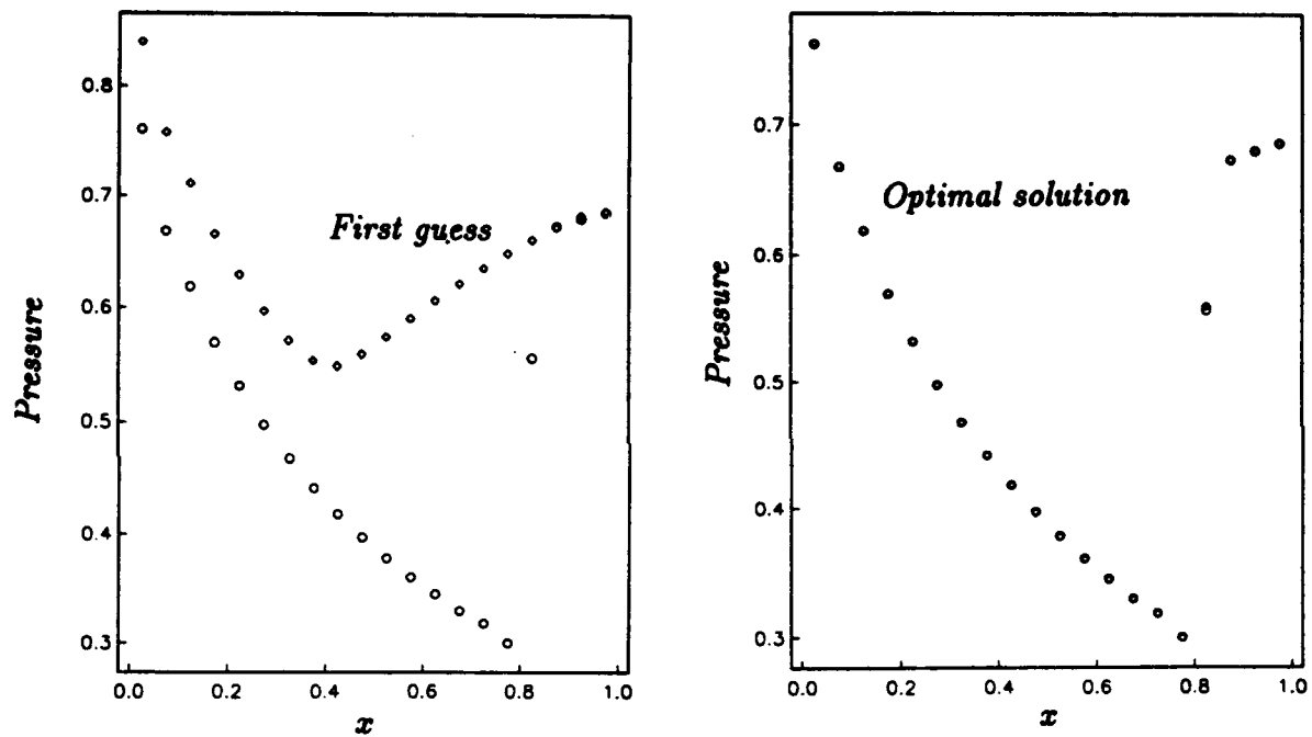
Figure 5: Target solution is h(x) = 2.5X + 0.3/X + 5 . First guess is h(x) = 2X + 0.52/X + 5 . Shape function for which minimum is sought is h(x) = \alpha_1 X + \alpha_2/X + 5 , and optimization algorithm used is BFGS. Starting value of the functional is of order 10^{-3} . At minimum it is of order 10^{-9} . Gradient components are of order 10^{-12} at minimum.
