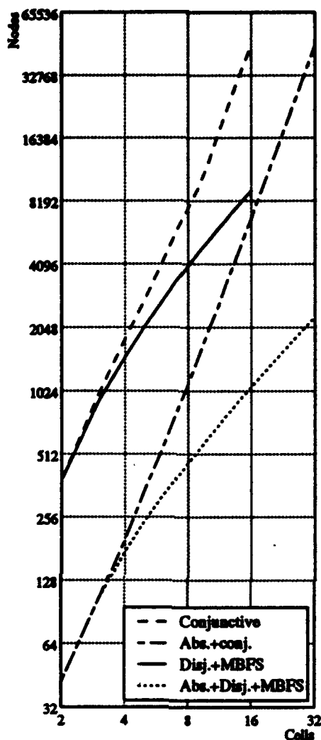
Figure 14: State set BDD sizes for DME circuit
