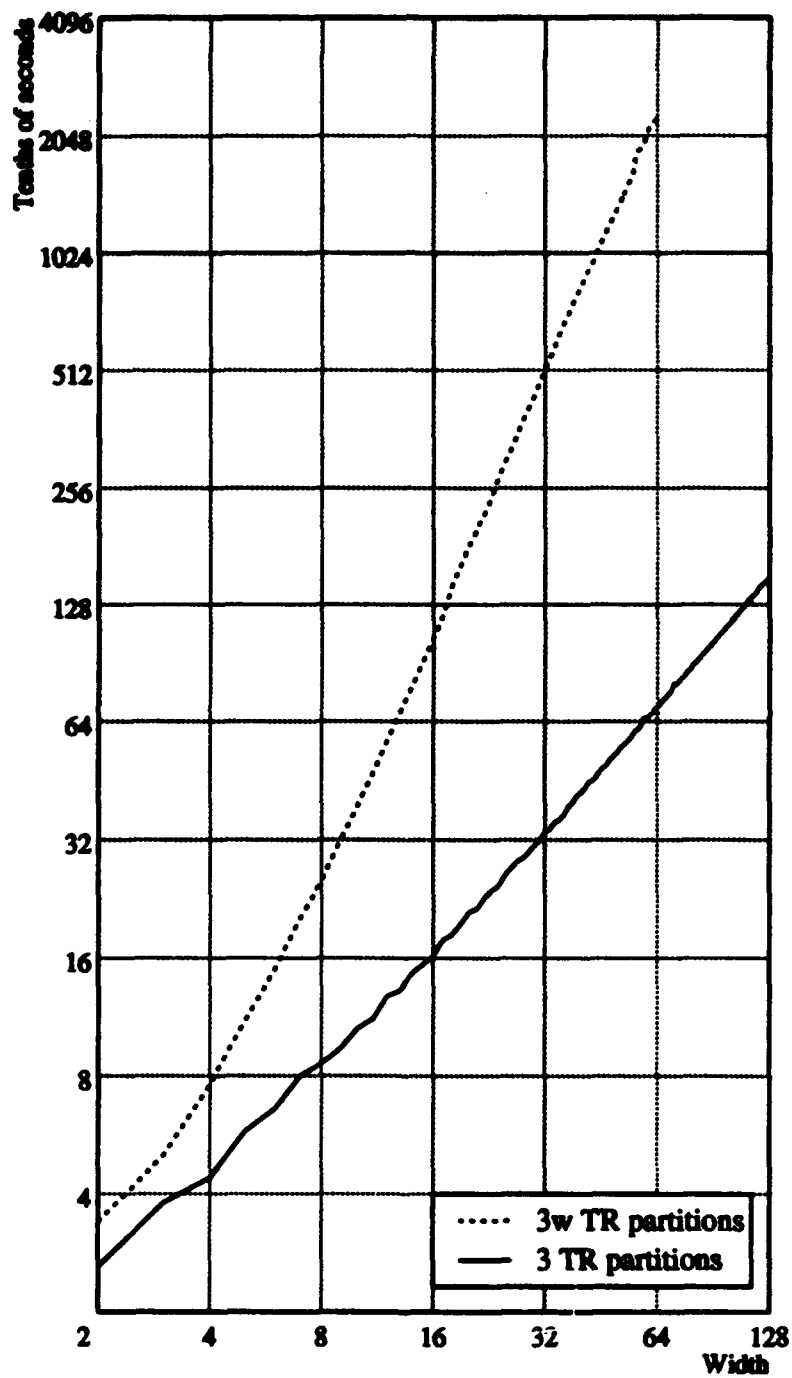
Figure 6: Verification times for MINMAX circuit
