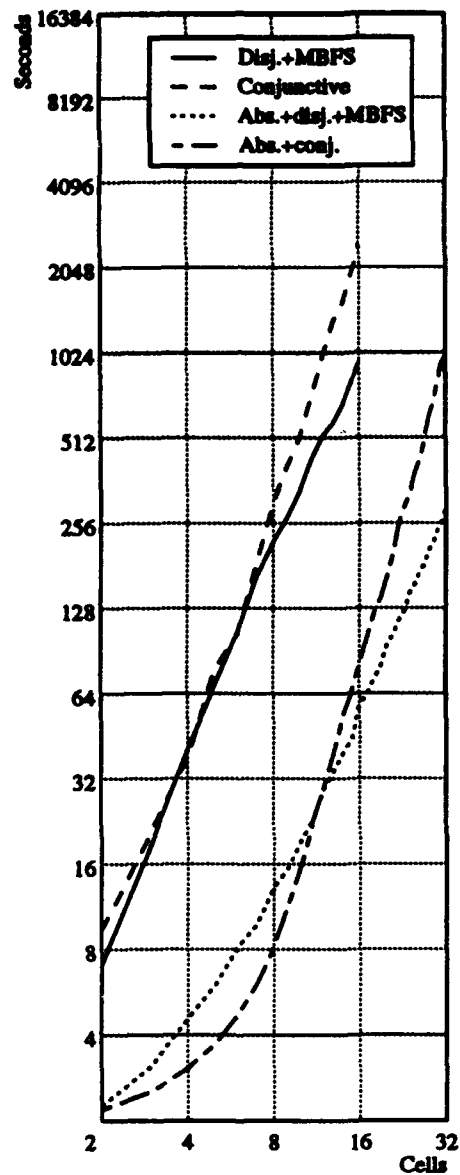
Figure 13: DME circuit verification times
