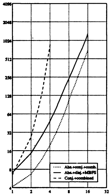
Figure 10: Search times in seconds for stacks of various depths, with w = 1
