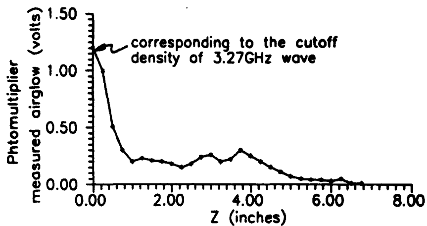
Fig. 18 (a) Spatial distribution of the peak airglow intensity emitting from an 1\mu\text{s} 3.27 GHz microwave pulse induced plasma
