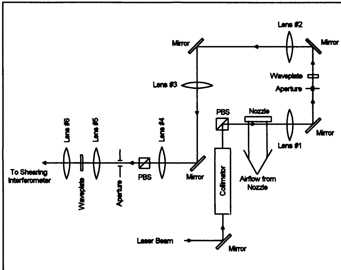
Figure 10. Experimental setup.
