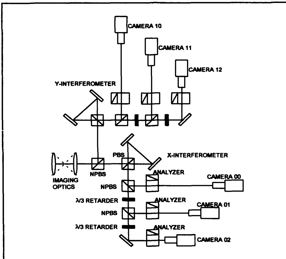
Figure 3. Shearing interferometer (SI).
