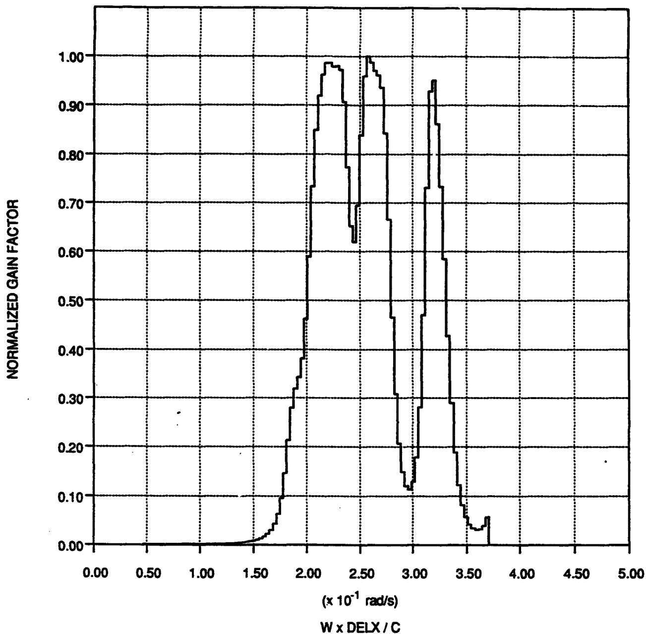
BEAM BREAKUP GAIN CURVE Peak gain = 0.17824 \cdot [\text{kA}] / \gamma
