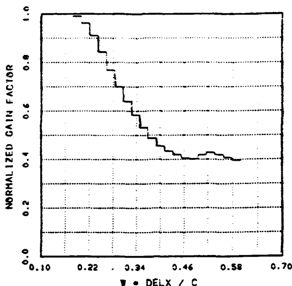
Figure 4. Normalized gain curve for highly-damped cavity.
