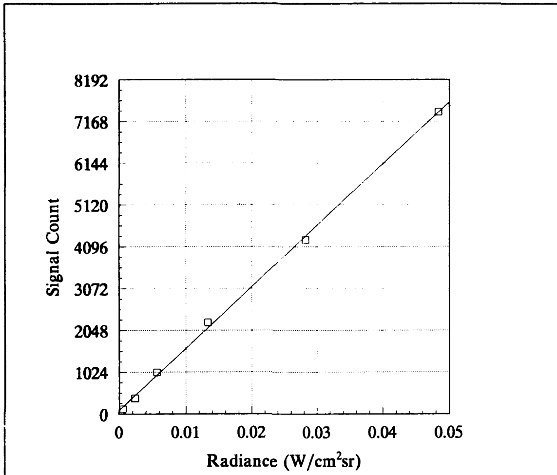
FIGURE B-15. RESPONSIVITY OF THE 880+ WITH THE 7° LENS, NO FILTERS, AND APERTURE 1.
