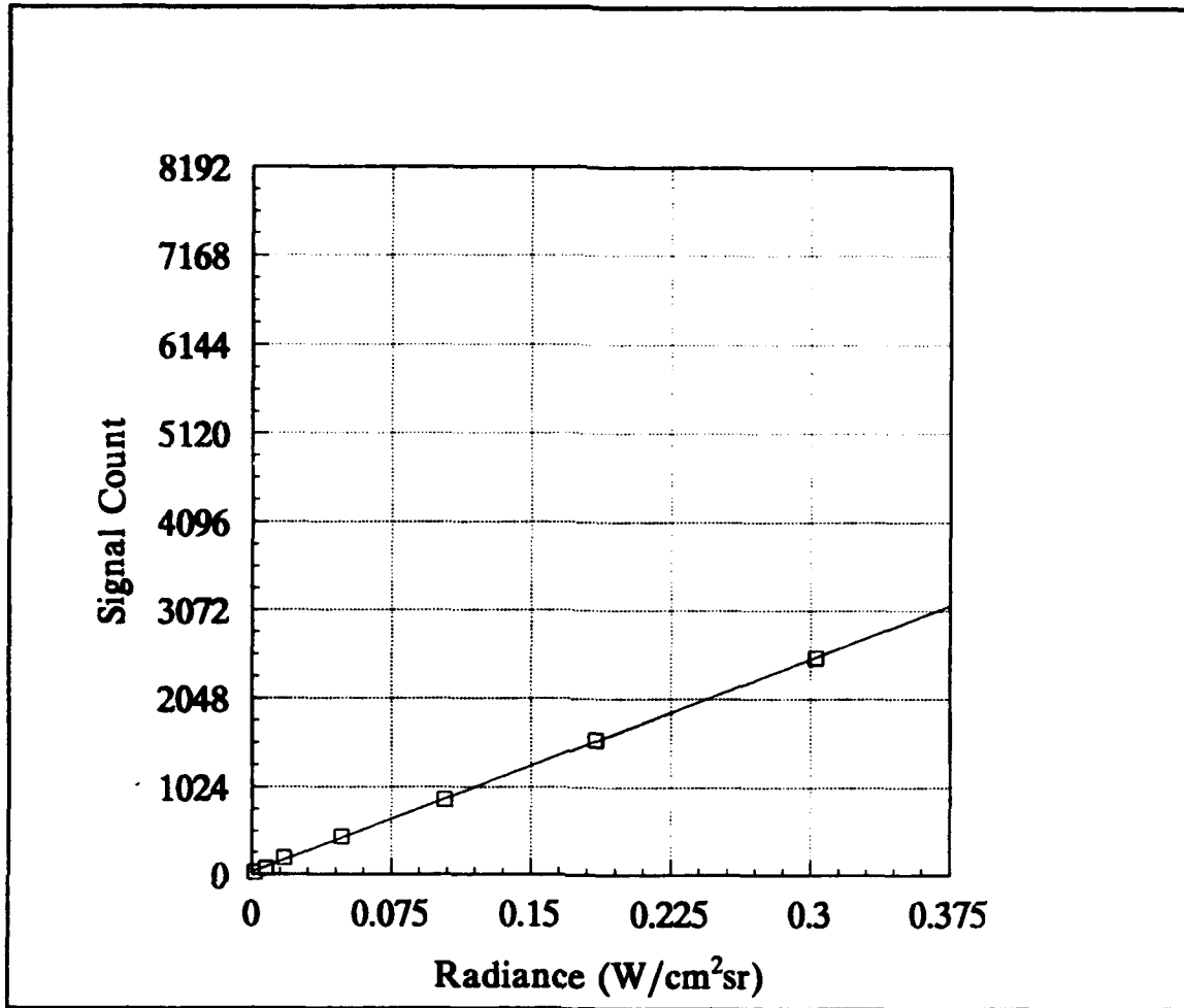
FIGURE B-21. RESPONSIVITY OF THE 880+ WITH THE 7° LENS, BLUE FILTER, AND APERTURE 1.
