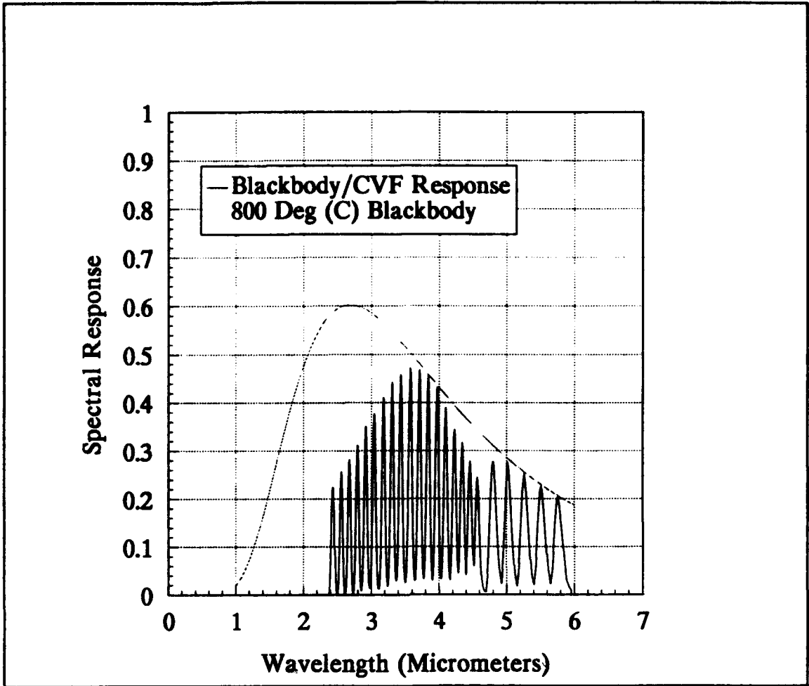
FIGURE B-4. CALCULATED IN-BAND RADIANCE FOR A 800 BLACKBODY (SOLID LINE). THEORETICAL PLANCK CURVE (DOTTED LINE) IS MULTIPLIED BY THE FILTER CVF1 TO GET THE IN-BAND RADIANCE.
