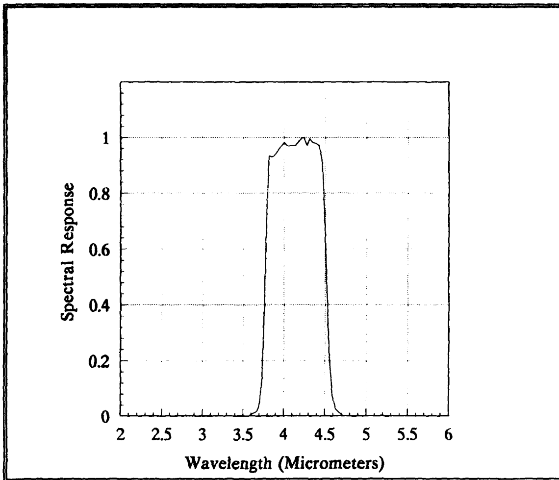
FIGURE A-1. NORMALIZED SPECTRAL TRANSMISSION OF THE 880+ YELLOW FILTER.
