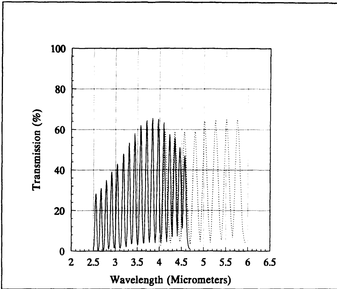
FIGURE B-1. TWO SEGMENTS OF THE OCLI CVF. SOLID LINE IS SEGMENT 1. DOTTED LINE IS SEGMENT 2.
