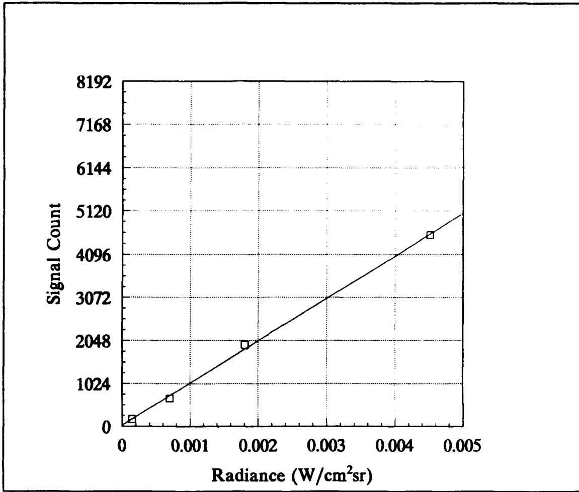
FIGURE B-17. RESPONSIVITY OF THE 880+ WITH THE 7° LENS, YELLOW FILTER, AND APERTURE 0.
