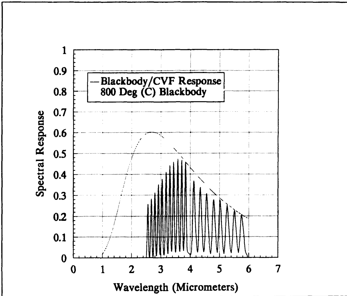
FIGURE B-5. CALCULATED IN-BAND RADIANCE FOR A 800 BLACKBODY (SOLID LINE). THEORETICAL PLANCK CURVE (DOTTED LINE) IS MULTIPLIED BY THE FILTER CVF2 TO GET THE IN-BAND RADIANCE.
