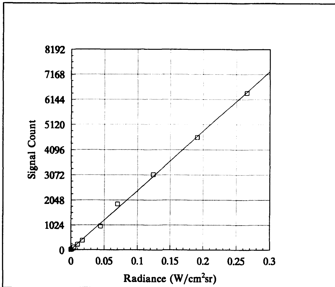
FIGURE B-19. RESPONSIVITY OF THE 880+ WITH THE 7° LENS, YELLOW FILTER, AND APERTURE 2.
