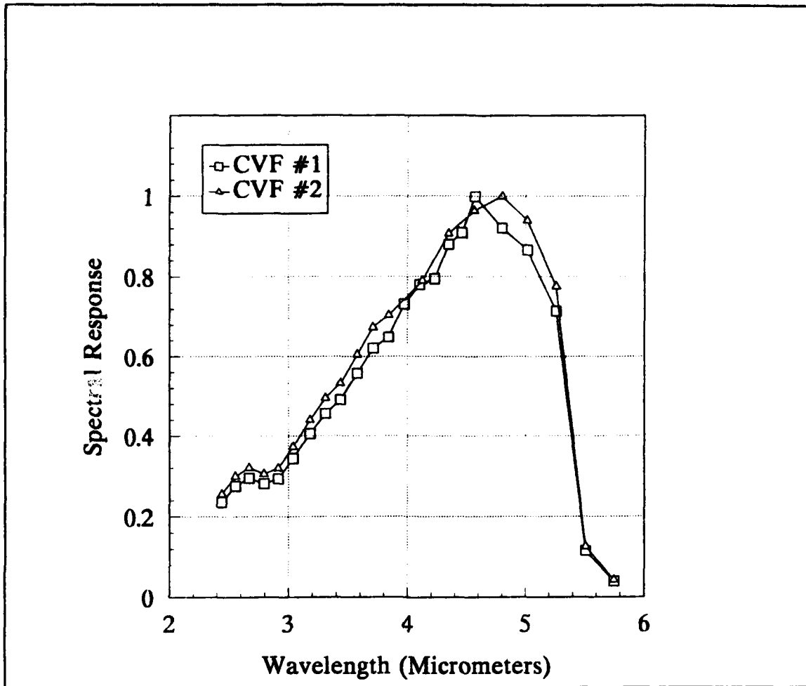
FIGURE B-7. SPECTRAL RESPONSE OF THE 880+ SYSTEM. AN 801°C BLACKBODY IS VIEWED AT EACH CVF ANGULAR POSITION AND THE MEASURED SIGNAL IS DIVIDED BY THE IN-BAND RADIANCE CALCULATED WITH FILTERS CVF1 AND CVF2.
