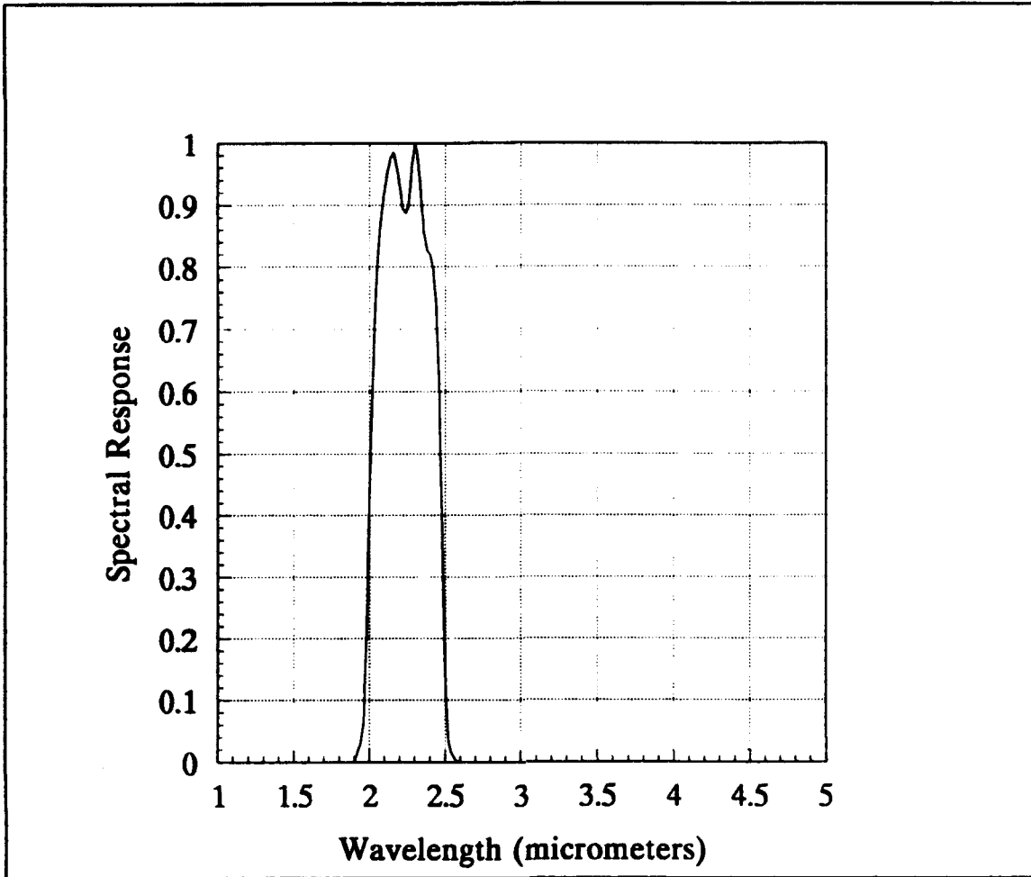
FIGURE B-13. NORMALIZED SPECTRAL TRANSMISSION OF THE BLUE FILTER.
