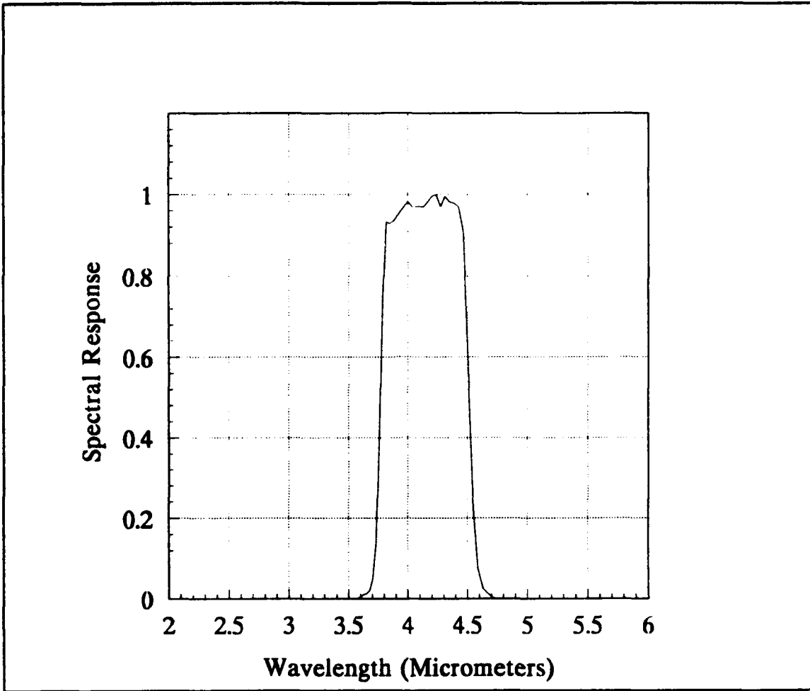
FIGURE B-11. NORMALIZED SPECTRAL TRANSMISSION OF THE YELLOW FILTER.
