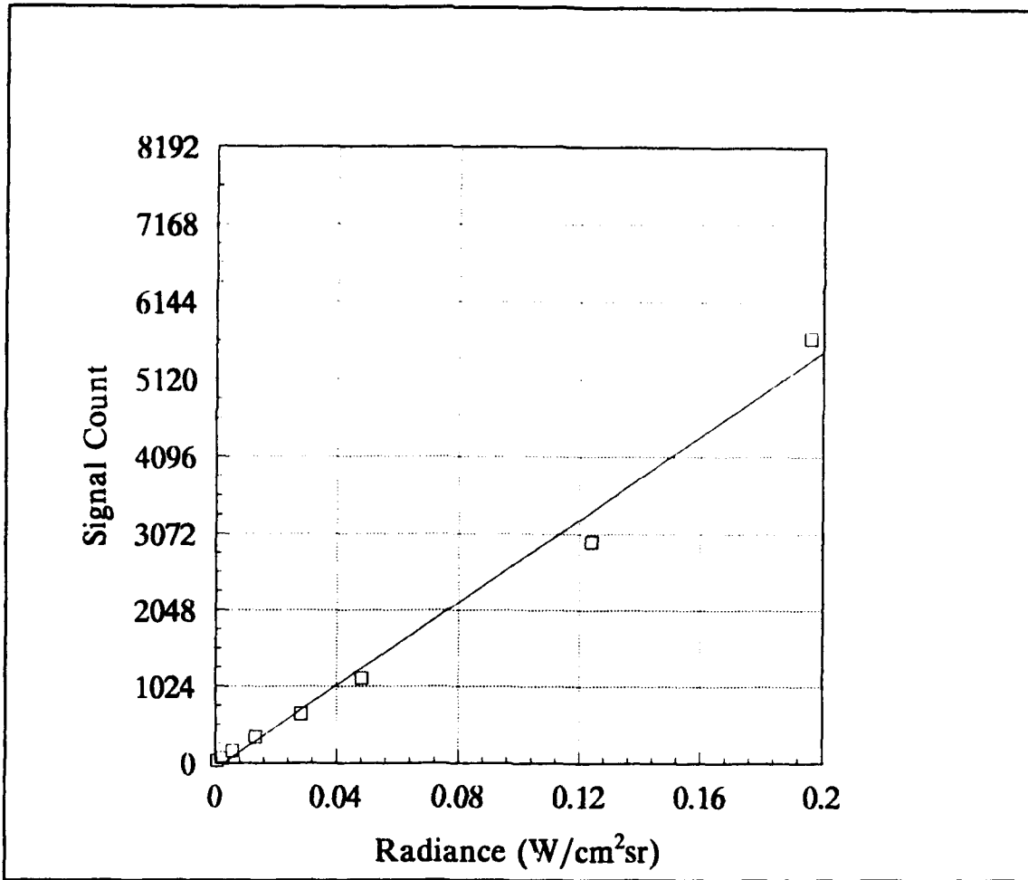
FIGURE B-16. RESPONSIVITY OF THE 880+ WITH THE 7° LENS, NO FILTERS, AND APERTURE 2.
