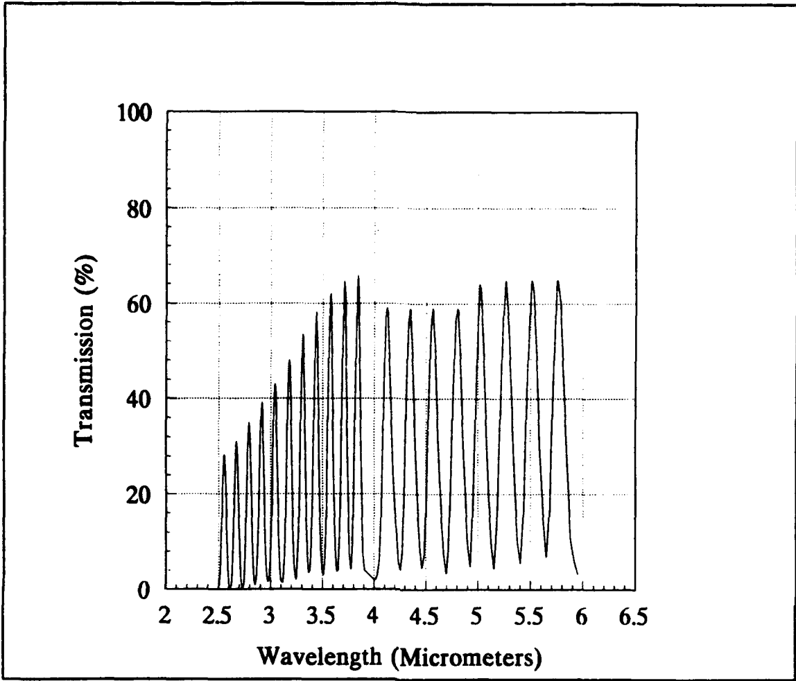
FIGURE B-3. COMBINATION OF COMPLETE CVF SEGMENT 2 AND THE PORTION OF CVF SEGMENT 1 FROM 2.380 TO 4.000 \mu\text{m} .
