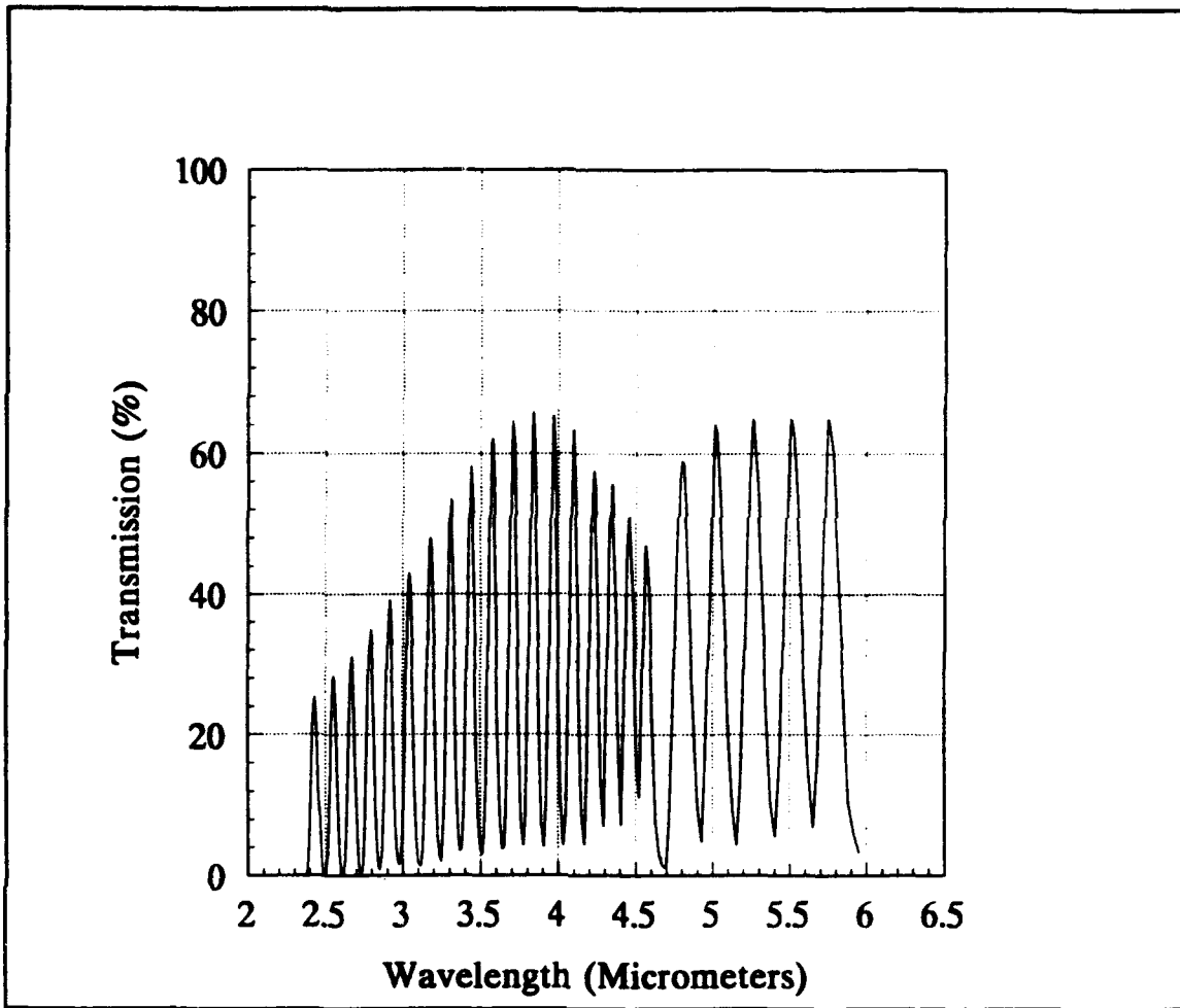
FIGURE B-2. COMBINATION OF COMPLETE CVF SEGMENT 1 AND THE PORTION OF CVF SEGMENT 2 FROM 4.717 TO 5.950 \mu\text{m} .
