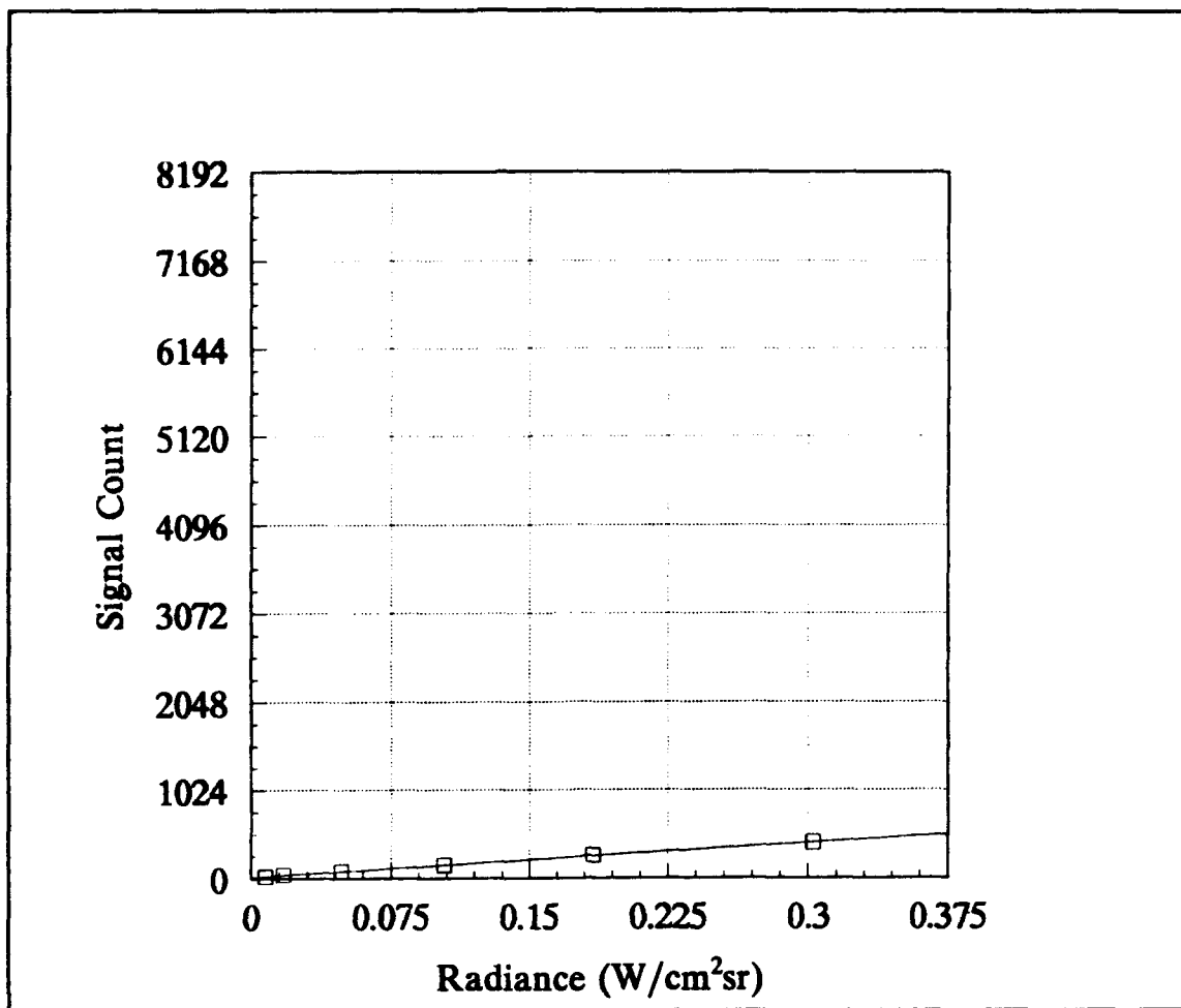
FIGURE B-22. RESPONSIVITY OF THE 880+ WITH THE 7° LENS, BLUE FILTER, AND APERTURE 2.
