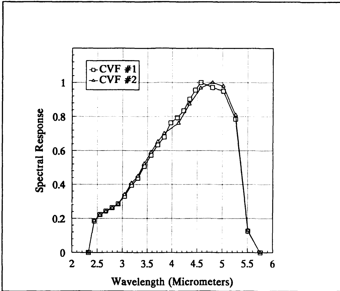
FIGURE B-6. SPECTRAL RESPONSE OF THE 880+ SYSTEM. AN 805°C BLACKBODY IS VIEWED AT EACH CVF ANGULAR POSITION AND THE MEASURED SIGNAL IS DIVIDED BY THE IN-BAND RADIANCE CALCULATED WITH FILTERS CVF1 AND CVF2.
