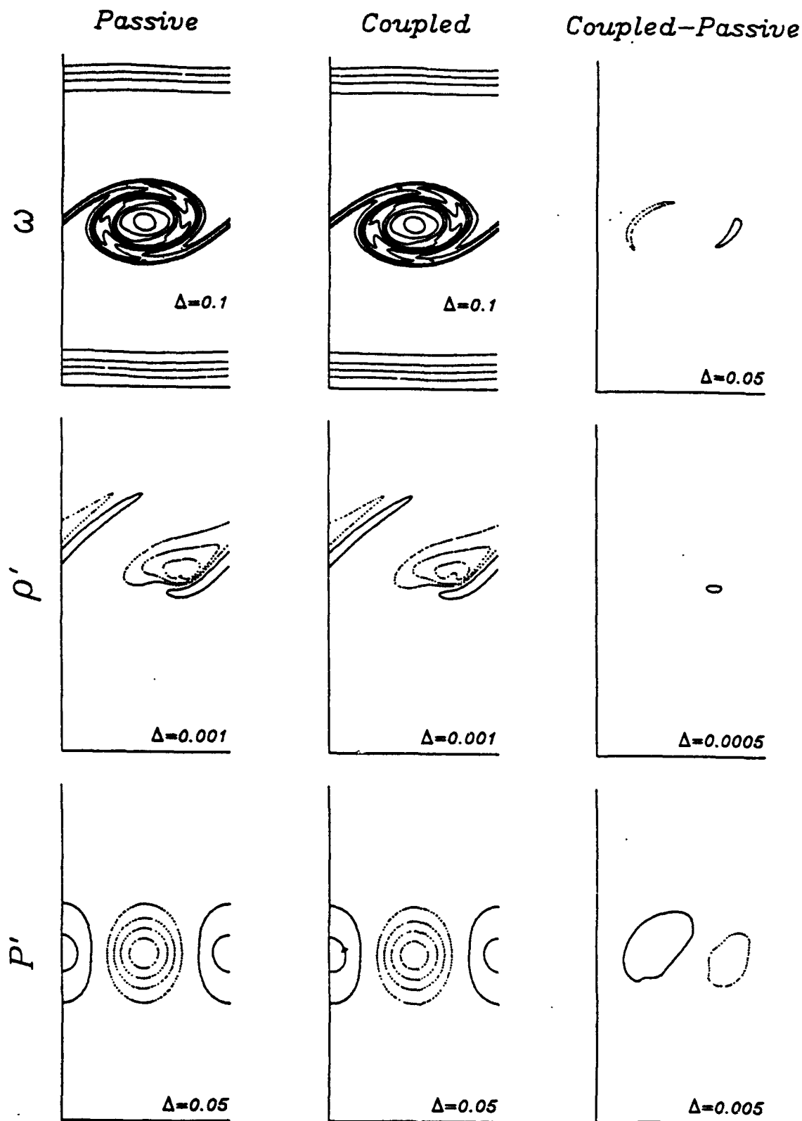
Figure 11: Vorticity, density and pressure fields for the coupled and passive cases, along with their differences, for \mathcal{A} = 5.8 and \mathcal{F} = 0.707 at (a) t = 30 , (b) t = 40 , (c) t = 50 . Although we see the accumulation of bubbles similar to previous cases at t = 30 , at later times the pressure gradient is not large enough to entrap bubbles, and as a result we observe streaks of bubbles which are produced from a least unstable point replacing the equilibrium point.
