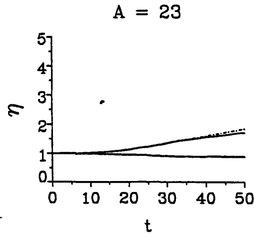
Figure 12: Time series of maximum and minimum number density for: \mathcal{A} = 5.8 (top), 10.3 (center), and 23 (bottom). All cases have \mathcal{F} = 0.707 . The solid lines represent two-way coupled and dashed lines passive simulations. The larger gravitational effects result in smaller accumulations, most noticeable in the \mathcal{A} = 5.8 case where there is no equilibrium point for the bubbles at later times.
