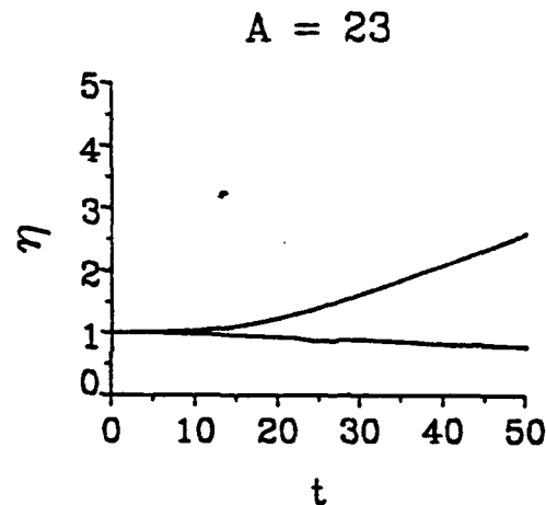
Figure 7: Time series of maximum and minimum number density for: A = 5.8 (top), 10.3 (center), and 23 (bottom). All cases have \mathcal{F} = 2 . The solid lines represent two-way coupled and dashed lines passive simulations. The reduced gravitational effects result in much larger accumulations for both passive and coupled cases than for the \mathcal{F} = 1 cases.
