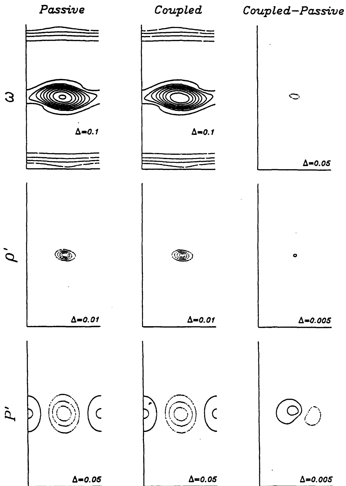
Figure 9: Vorticity, density and pressure fields for the coupled and passive cases, along with their differences, at t = 50 for \mathcal{F} = 2 and \mathcal{A} = 10.3 . Although the accumulation is greater than for the same sized bubbles with \mathcal{F} = 1 , due to the \mathcal{F}^{-2} coefficient the coupling effects are smaller.
