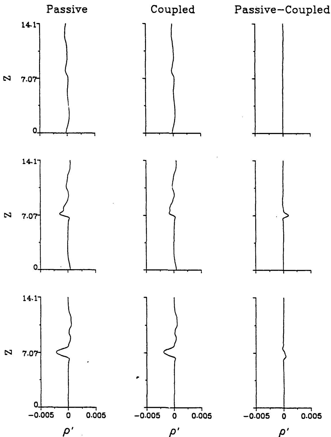
Figure 13: Vertical density profiles averaged over horizontal slices at t = 50 for: \mathcal{A} = 5.8 (top), 10.3 (center), and 23 (bottom). All cases have \mathcal{F} = .707 . This suggests that there is an optimum bubble size in terms of bubble accumulation for cases with small \mathcal{F} . For the smallest bubbles (bottom) the accumulation rate is small, but for large bubbles (top) rise velocity is so large that equilibrium points do not exist.
