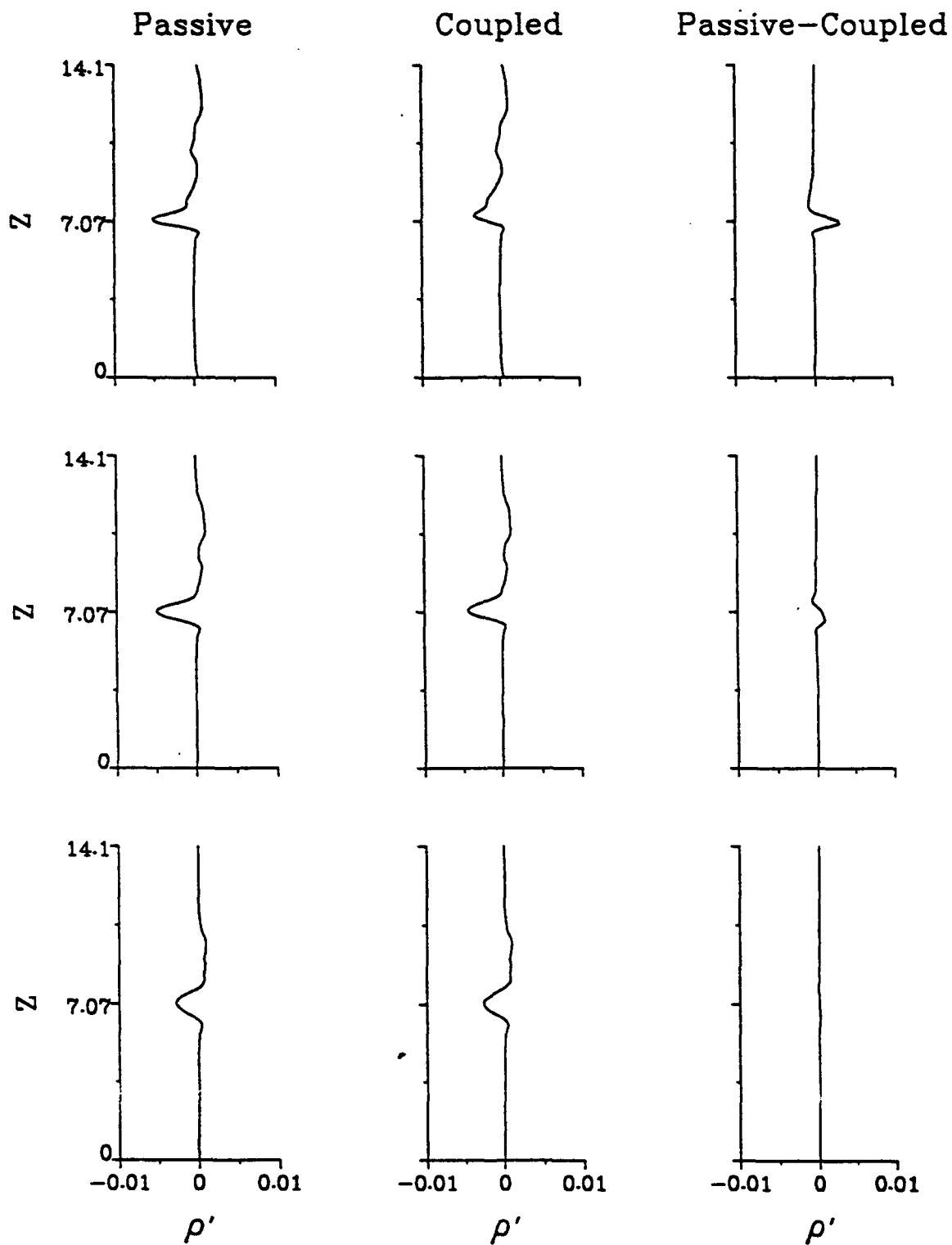
Figure 6: Vertical density profiles averaged over horizontal slices at t = 50 for: \mathcal{A} = 5.8 (top), 10.3 (center), and 23 (bottom). All cases have \mathcal{F} = 1 . Here we observe how the accumulation and difference between coupled and passive cases decrease with bubble size.
