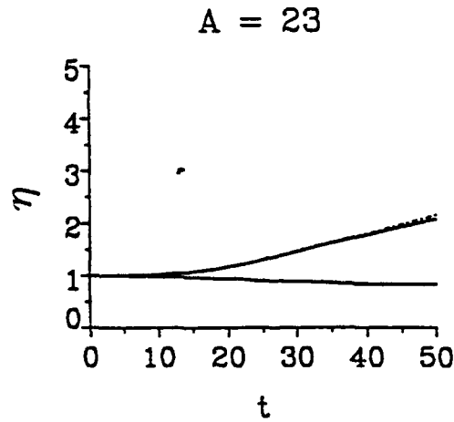
Figure 5: Time series of maximum and minimum number density, \eta , for: A = 5.8 (top), 10.3 (center), and 23 (bottom). All cases have \mathcal{F} = 1 . The solid lines represent two-way coupled and dashed lines passive simulations. These times series show that the accumulation of bubbles decreases with bubble size (larger A ). Note that for A = 5.8 the maximum accumulation for the coupled case becomes smaller as bubbles are released from the equilibrium points.
