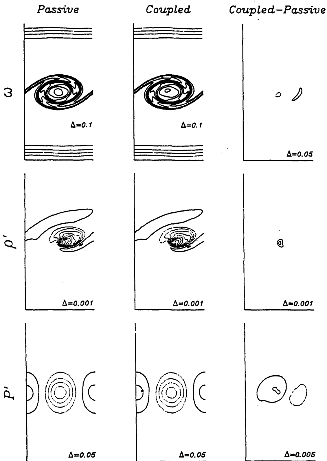
Figure 2: Vorticity, density and pressure fields for the coupled and passive cases, along with their differences, at a) t = 30 and b) t = 50 for \mathcal{F} = 1 and \mathcal{A} = 5.8 . The solid lines indicate positive values and the dashed line negative values. The increment between countour levels is given in each figure. At t = 30 , the accumulation is not large enough to produce substantial changes from the coupling, however at t = 50 we observe differences in all fields, most notably the reduction in vorticity, pressure gradient, and bubble accumulation near the vortex center.
