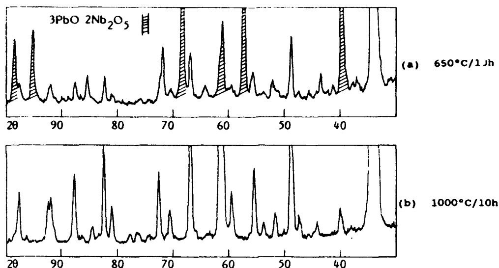
FIGURE 2 X-Ray powder diffraction pattern at various temperatures
