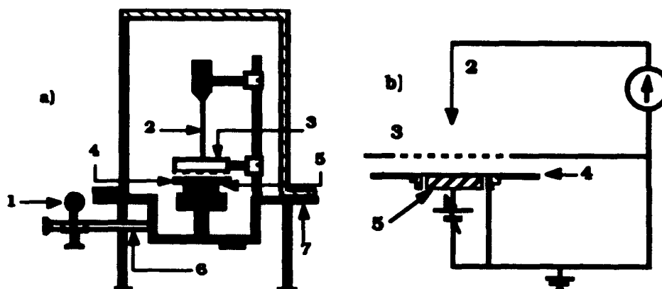
FIGURE 1 a) - The Corona Chamber: 1-manometer; 2-Corona tip (sewing needle); 3-Metallic Grid; 4- Electret; 5-Metallic sample holder (Back electrode); 6- to vacuum pump and gas inlet; 7- Horizontal flange. b) - The Corona Triode.
