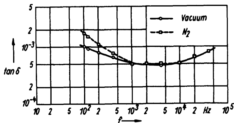
FIGURE 6 Dielectric loss vs. frequency of samples of TGS:L-A+Cr 3+ measured in \text{N}_2 and high vacuum
