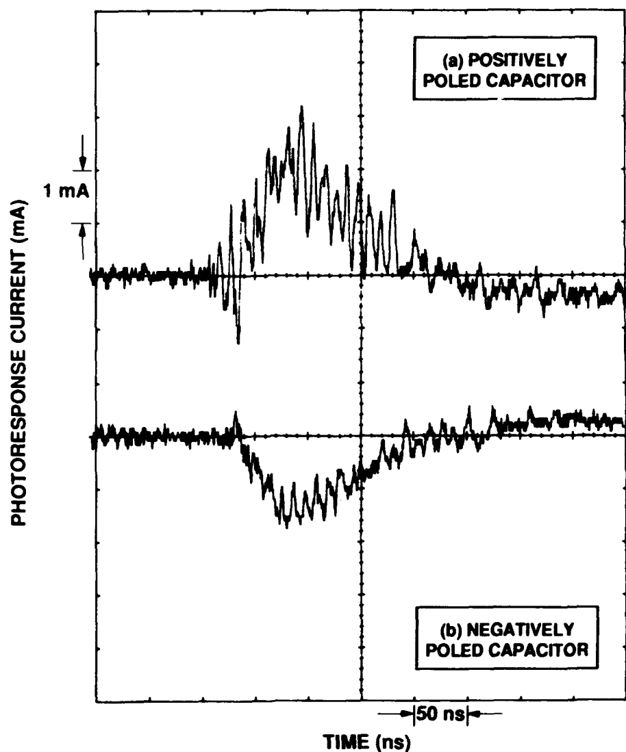
FIGURE 1 First readout of photoresponse current from thin film ferroelectric capacitor (TFFC) with semitransparent top electrode (a) positively polarized state (b) negatively polarized state
