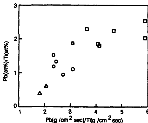
FIGURE 5 Plots of Pb/Ti atomic ratio of deposited films vs. Pb/Ti evaporation rate. o; perovskite \text{PbTiO}_3 , □; Pb rich, Δ; Ti rich.
