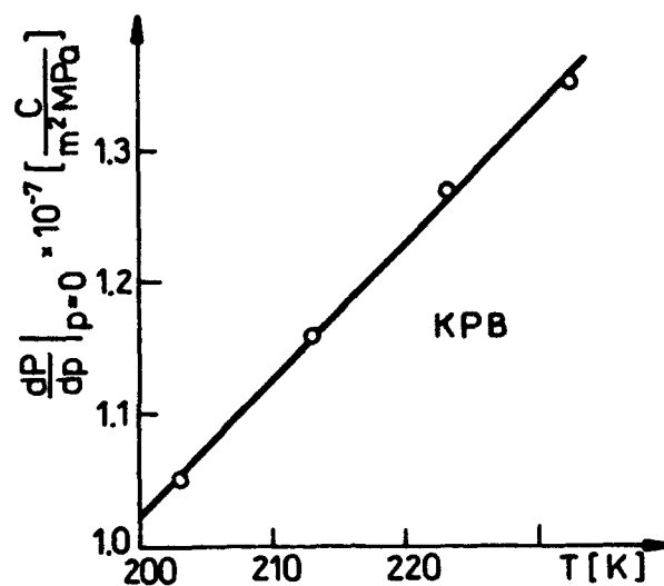
Fig.2. Temperature dependence of the pressureelectric coefficient for potassium pentaborate crystals (at p = 0 ).
