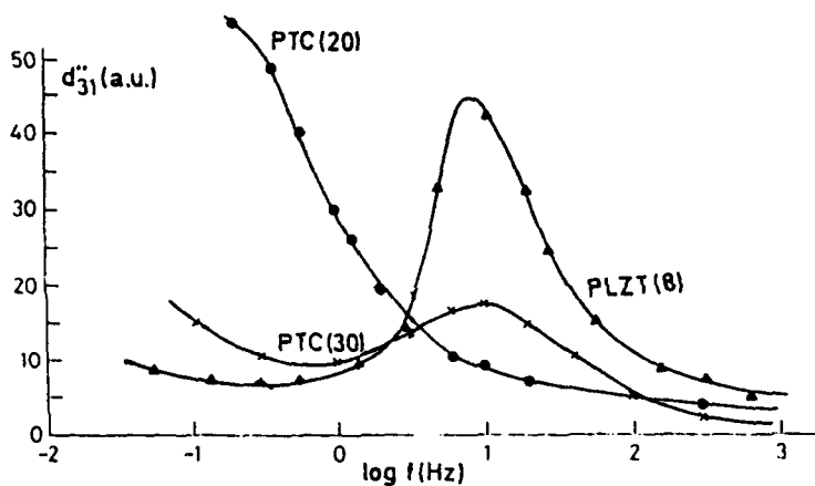
Fig. 3.- Imaginary part of d_{31} vs. frequency. ( 1 \text{ a.u.} \sim 3 \cdot 10^{-13} \text{C} )
