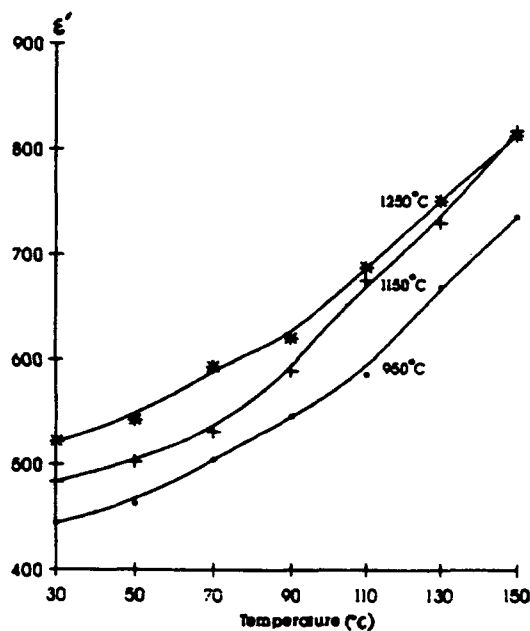
FIG 6. Dielectric constant vs Temperature for PGZT samples subjected to 950°C, 1150°C and 1250°C sintering temperatures at a fixed frequency of 1 kHz.
