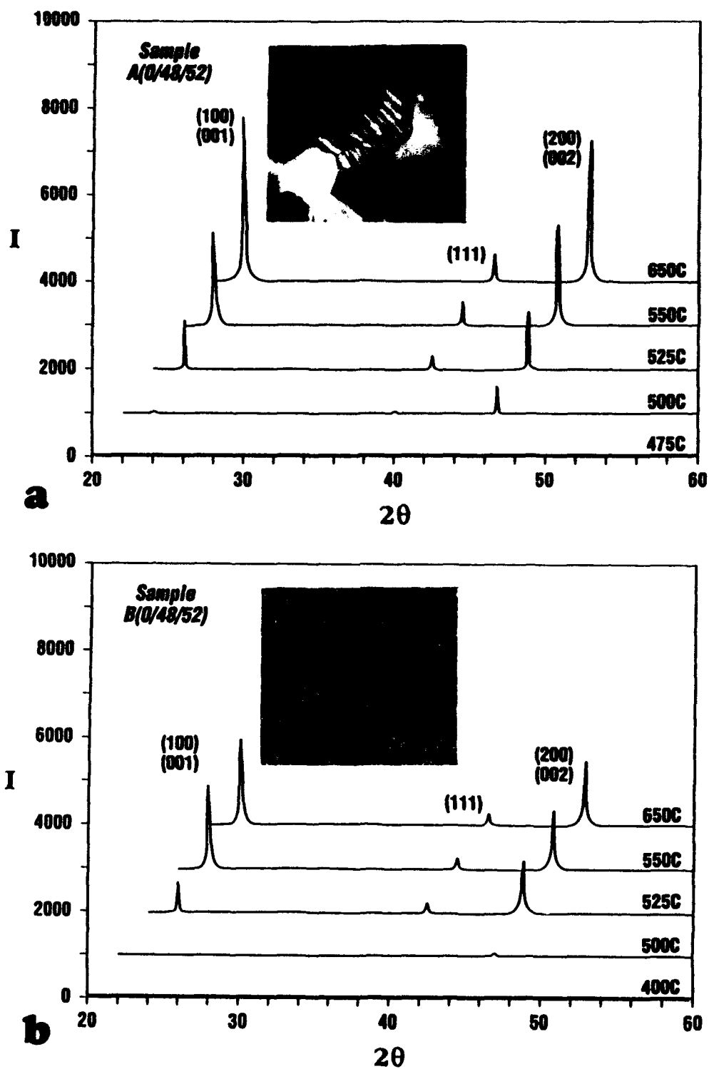
FIGURE 1 XRD spectra and corresponding TEM micrographs of samples analyzed (a,b,c,d). See text for details.
