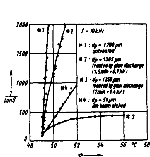
FIGURE 4 Dielectric loss vs. temperature of samples with various ways of surface treatment
