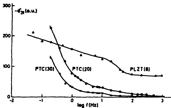
Fig. 2.- Real part of d_{31} vs. frequency. ( 1 \text{ a.u.} \sim 3 \cdot 10^{-13} \text{C} )
