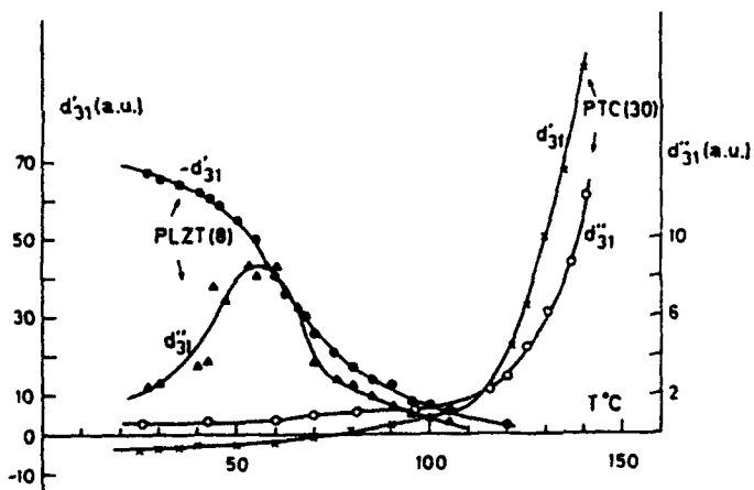
Fig. 4.- Real and imaginary parts of d_{31} vs. temperature. ( 1 \text{ a.u.} \sim 3 \cdot 10^{-13} \text{C} )
