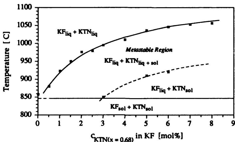
FIGURE 1 Partial phase diagram of KF/KTN( x = 0.68 ).
