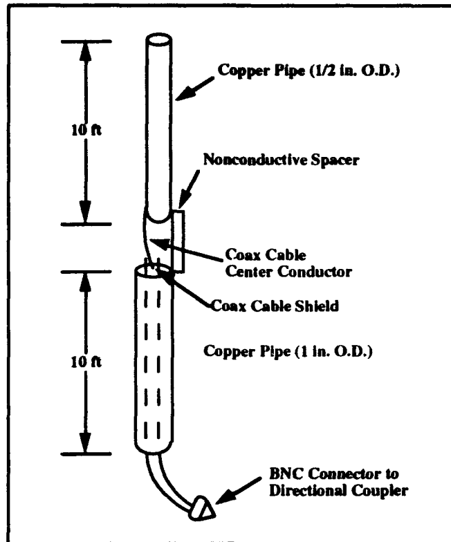
Figure 6-1. Bazooka Dipole
