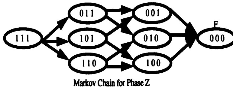
Figure 3: The Markov chains for three phases
