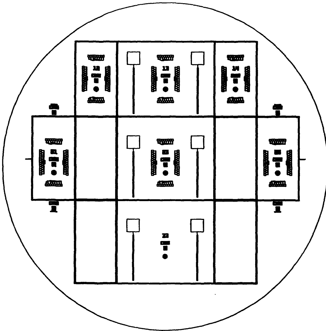
Figure 3. Diagram of layout of thin-film load structures (three chips in center column), test pieces for measurement of surface resistance after processing (four blank rectangular chips), and test patterns for measuring dc properties of YBCO and the thin-film Mo/Ti resistors (remaining four chips) on a two-inch wafer.
