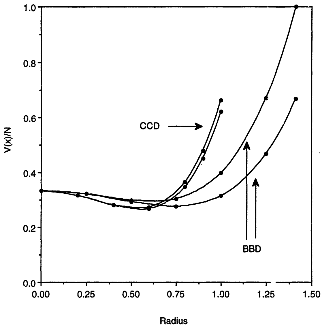
Figure 2. V(\mathbf{x}) / N for the Three-Factor Central Composite and Box-Behnken Designs.
