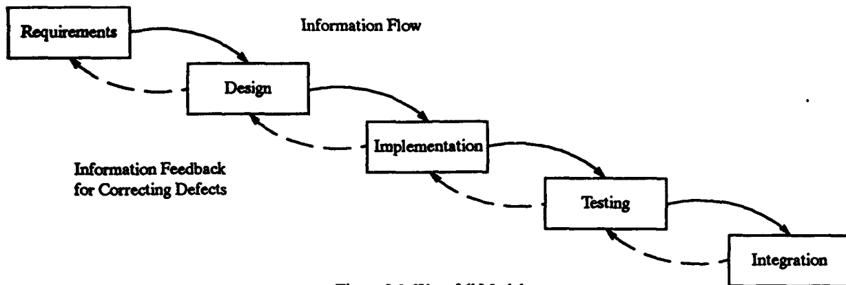
Figure 2-3. Waterfall Model
