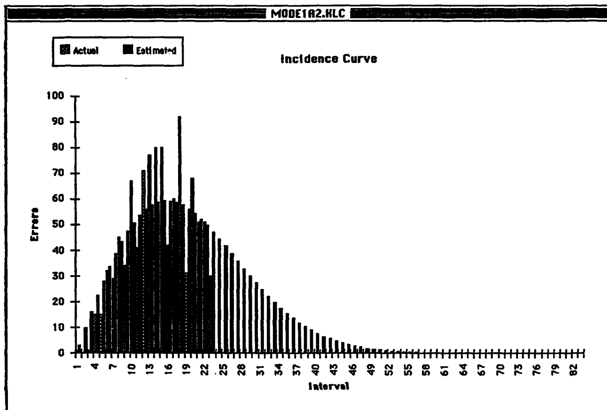
Figure 5-5. Error Incidence for 23 Months
