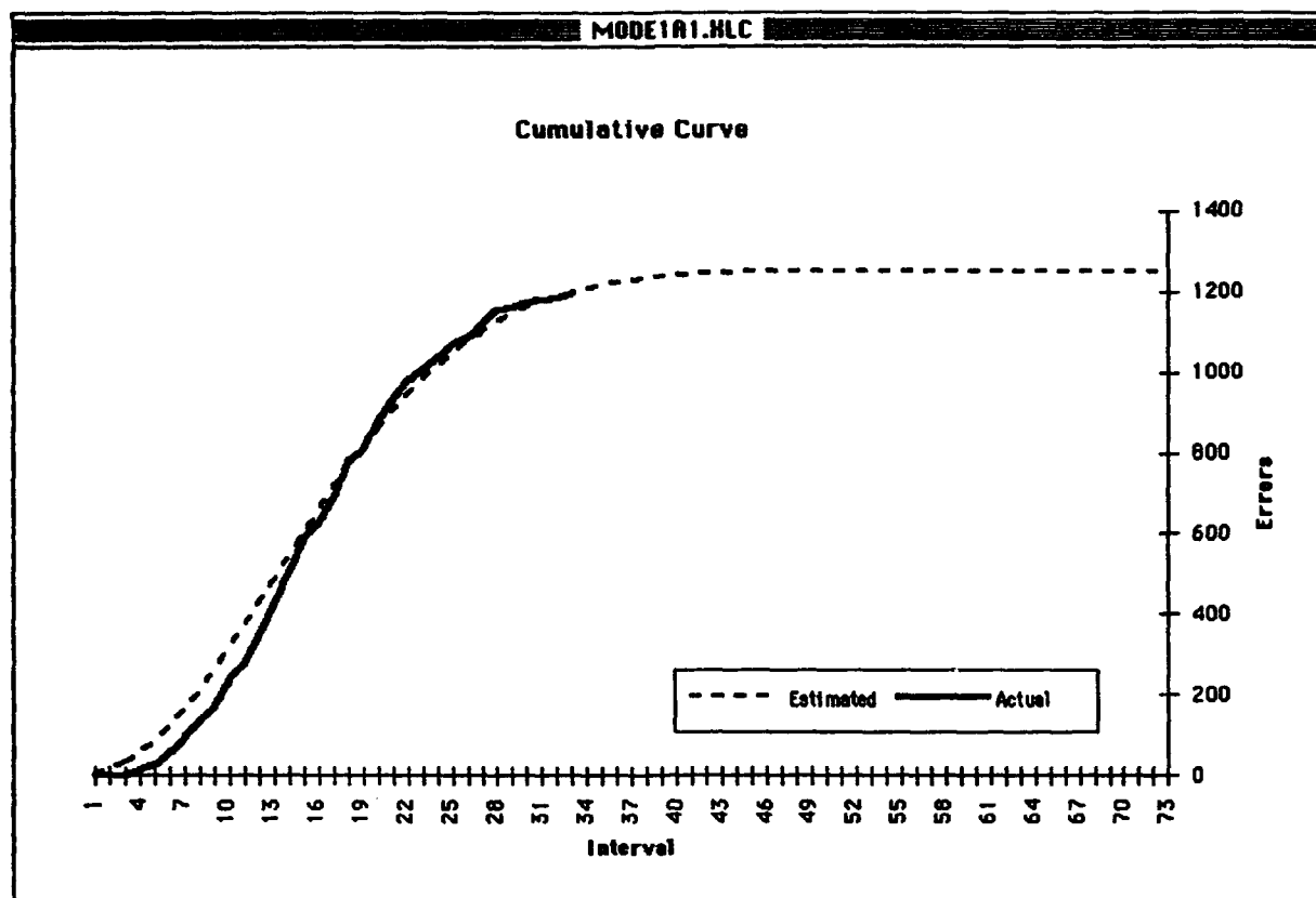
Figure 5-2. Cumulative Number of Errors for 33 Months
