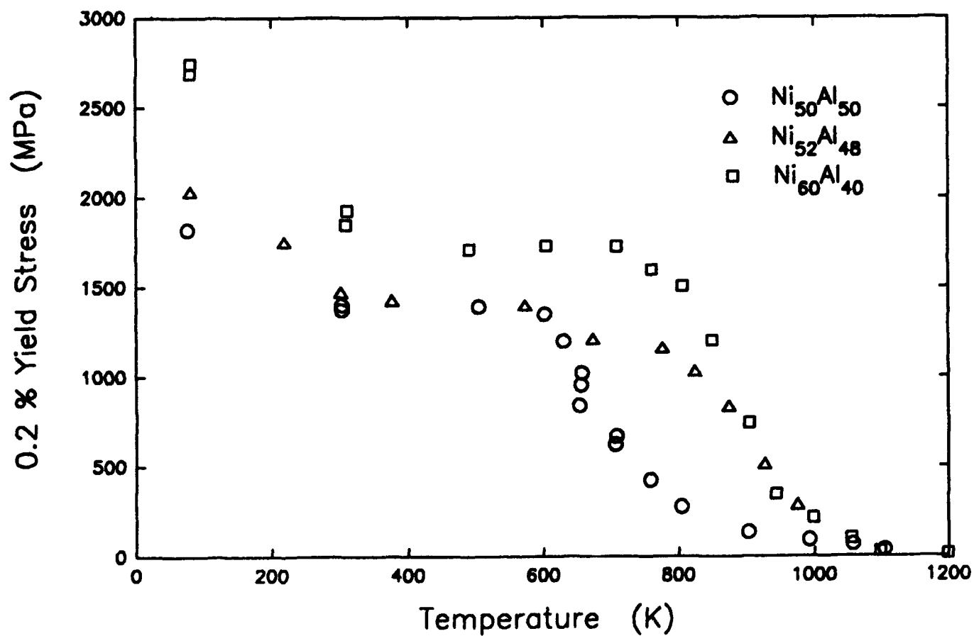
Figure 26.—The effect of alloy stoichiometry on the temperature dependent yield strength of [001] single crystal NiAl (ref. 149).
