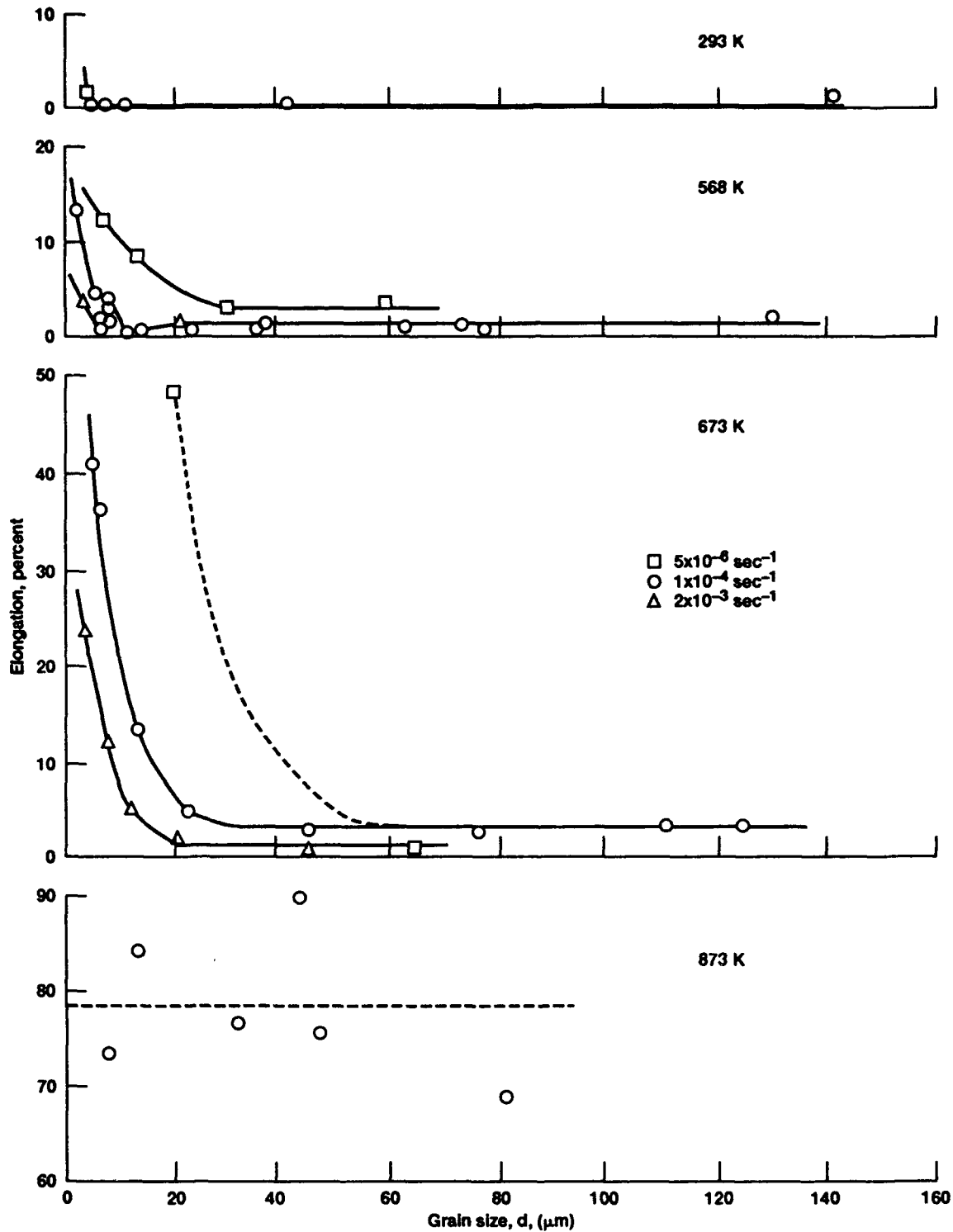
Figure 32.—Tensile elongation versus grain size for Ni-49Al at temperatures from 293 K to 873 K and strain rates from 5 \times 10^{-6} /s to 2 \times 10^{-3} /s (ref. 236).
