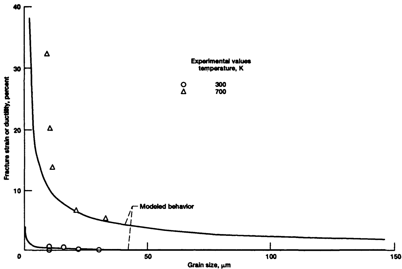
Figure 33.—Chen's model (ref. 258) for predicting tensile ductility of semibrittle materials as a function of grain size verified for NIAI (ref. 215). The figure shows experimental and theoretical ductility as a function of grain size for the alloy described in Table VIII.
