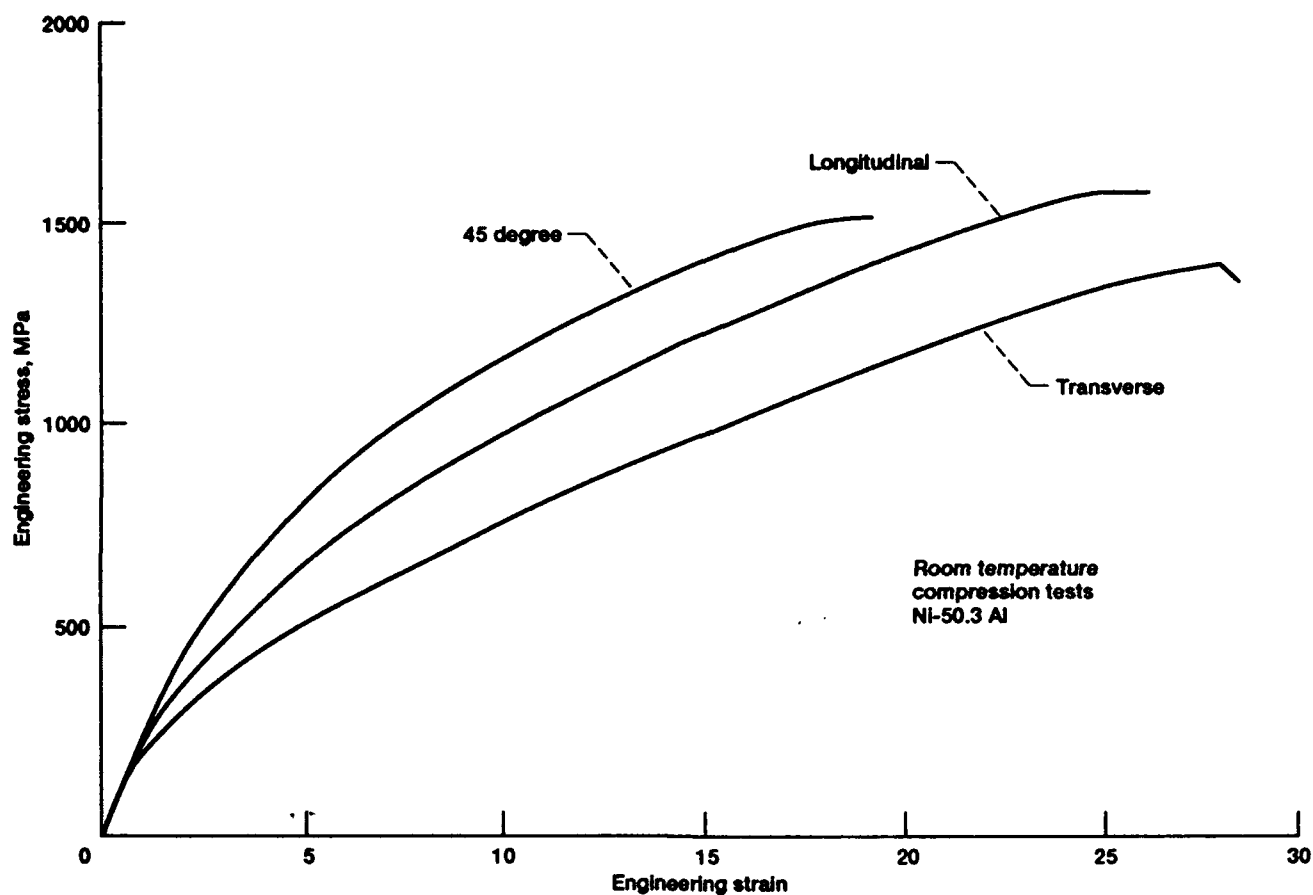
Figure 21.—The flow strength of extruded NIAI compression specimens taken from various orientations relative to the extrusion axis and tested at room temperature (ref. 178).
