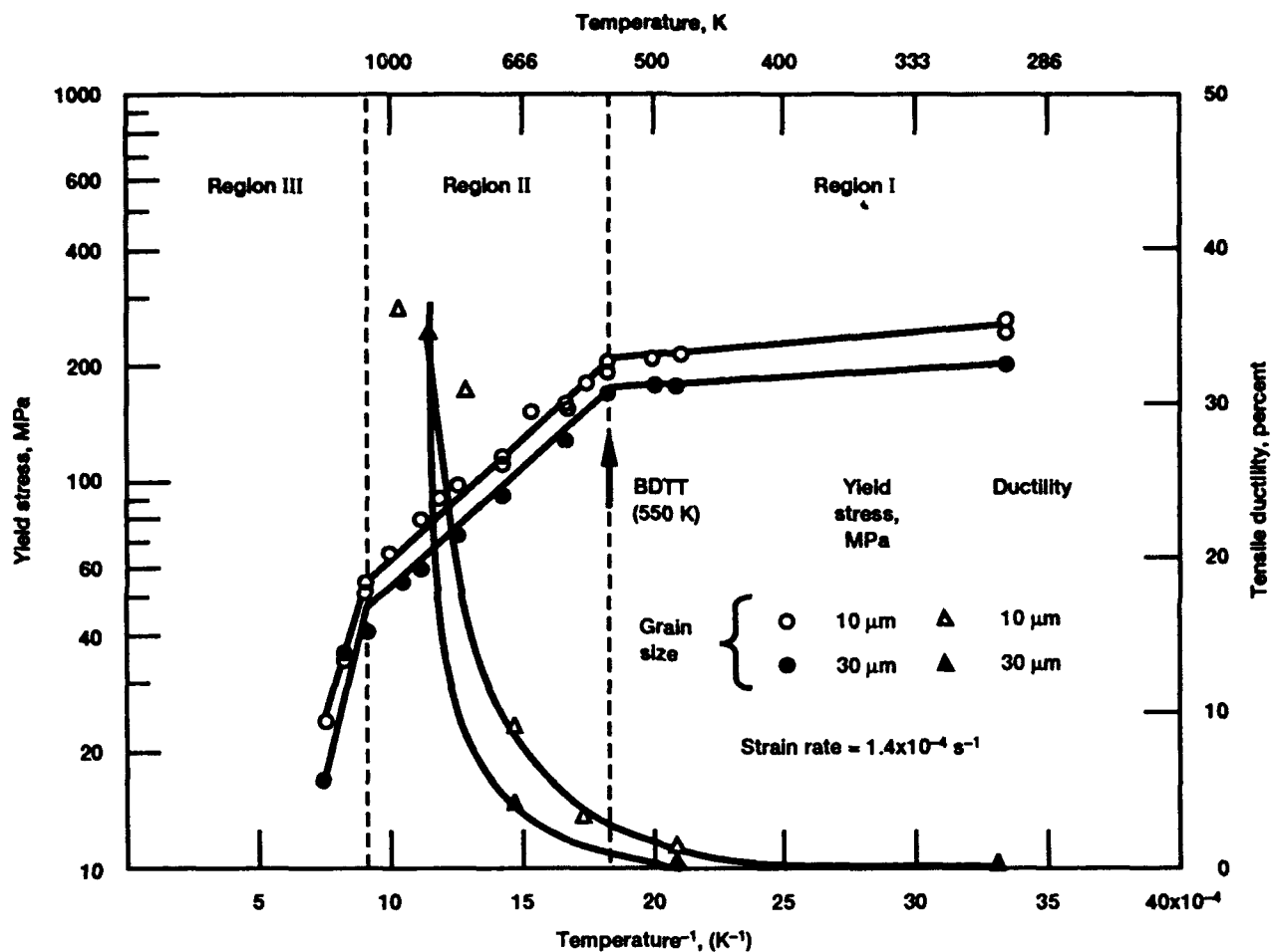
Figure 13.—Arrhenius representation of the yield stress of polycrystalline NiAl. The BDTT corresponds to a change in activation energy for plastic flow beginning at Region II (ref. 215).
