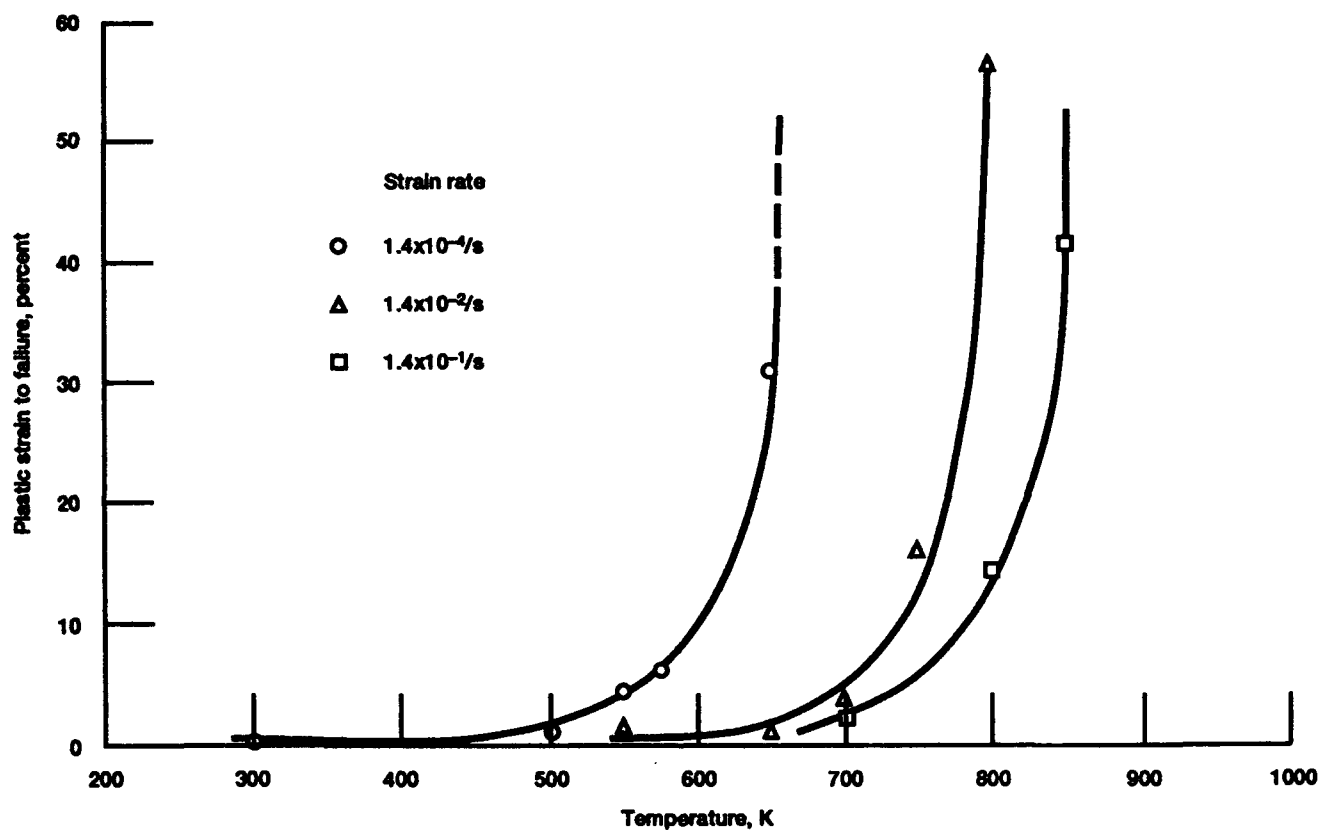
Figure 31.—The effect of strain rate on the tensile ductility and BDTT of cast and extruded NIAI (ref. 233).
