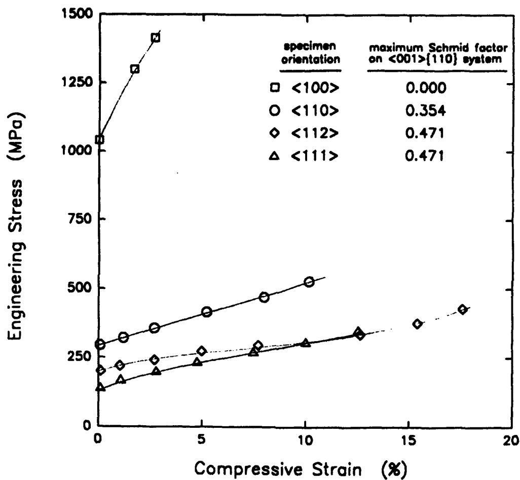
Figure 24.—The room temperature stress strain behavior of NIAI as a function of orientation (ref. 165).
