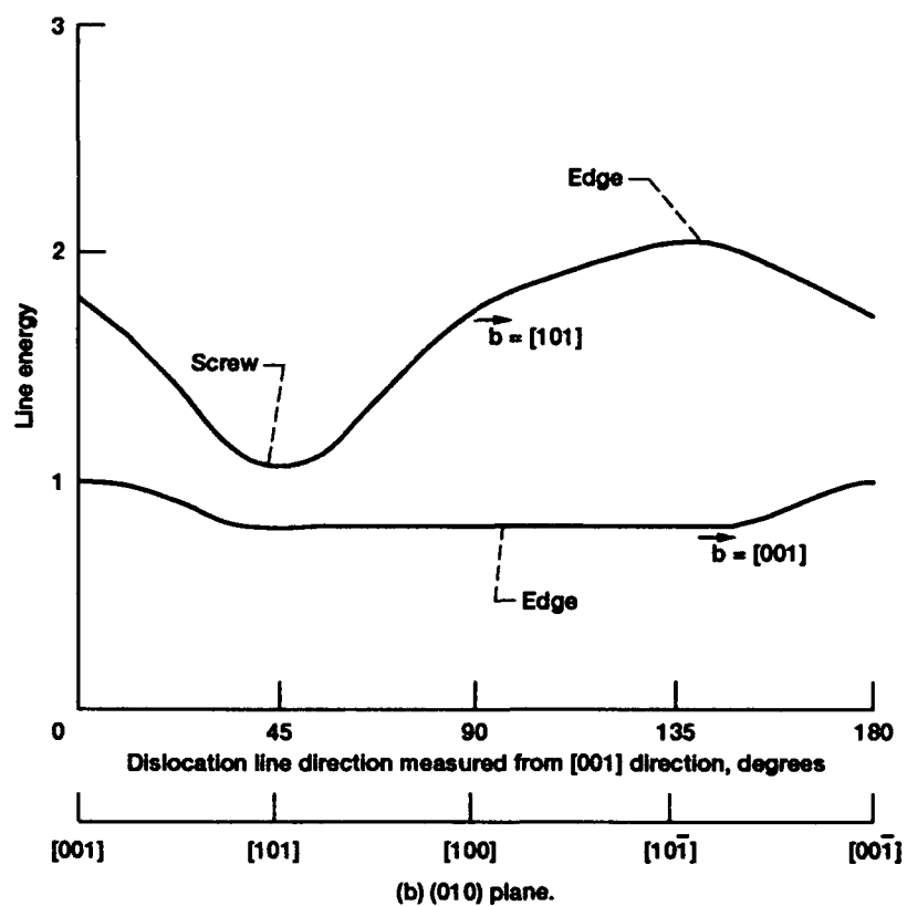
Figure 7.—Line energy for dislocations in stoichiometric NIAI at room temperature. (After Lloyd and Loretto ref. 140).
