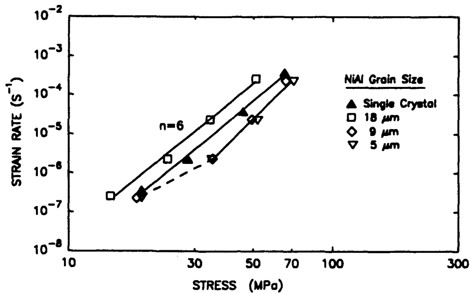
Figure 45.—The influence of grain size on the compressive creep strength of NiAl at 1300 K (refs. 316, 322).
