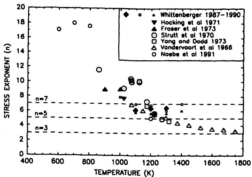
Figure 43.—The relationship between stress exponent and temperature for near stoichiometric NiAl as compiled from numerous studies (refs. 166, 170, 235, 316-319, 321, 322).
