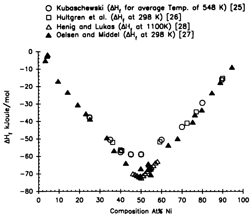
Figure 4.—Heats of formation for Ni-Al alloys.
