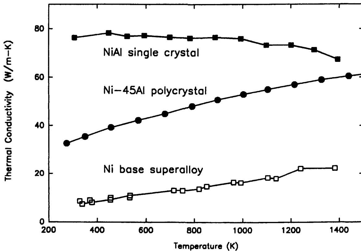
Figure 5.—Comparison of the thermal conductivity of single crystal NiAl (ref. 62), polycrystalline Ni-45Al (ref. 58), and a conventional nickel-base superalloy (ref. 62) as a function of temperature.
