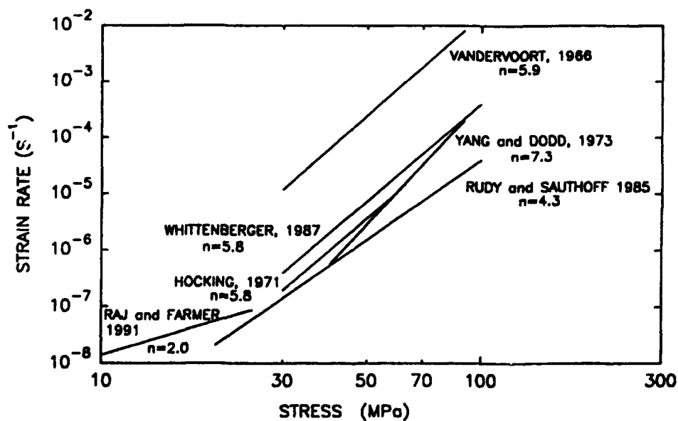
Figure 42.—Creep behavior of stoichiometric NiAl at 1175 K (refs. 235, 317, 319-321, 323).
