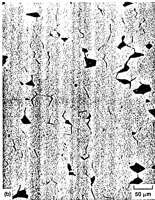
Figure 27.—Longitudinal sections of NiAl compression specimens deformed to (a) 5 percent plastic strain and (b) 15 percent plastic strain at room temperature illustrating the formation of grain boundary cracks (ref. 128).
