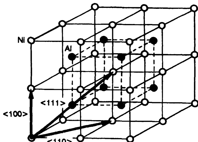
Figure 1.—The B2 crystal structure and unit lattice (slip) vectors for NiAl. Shown are eight unit cells illustrating the interpenetrating simple cubic sublattices of Ni and Al atoms.
