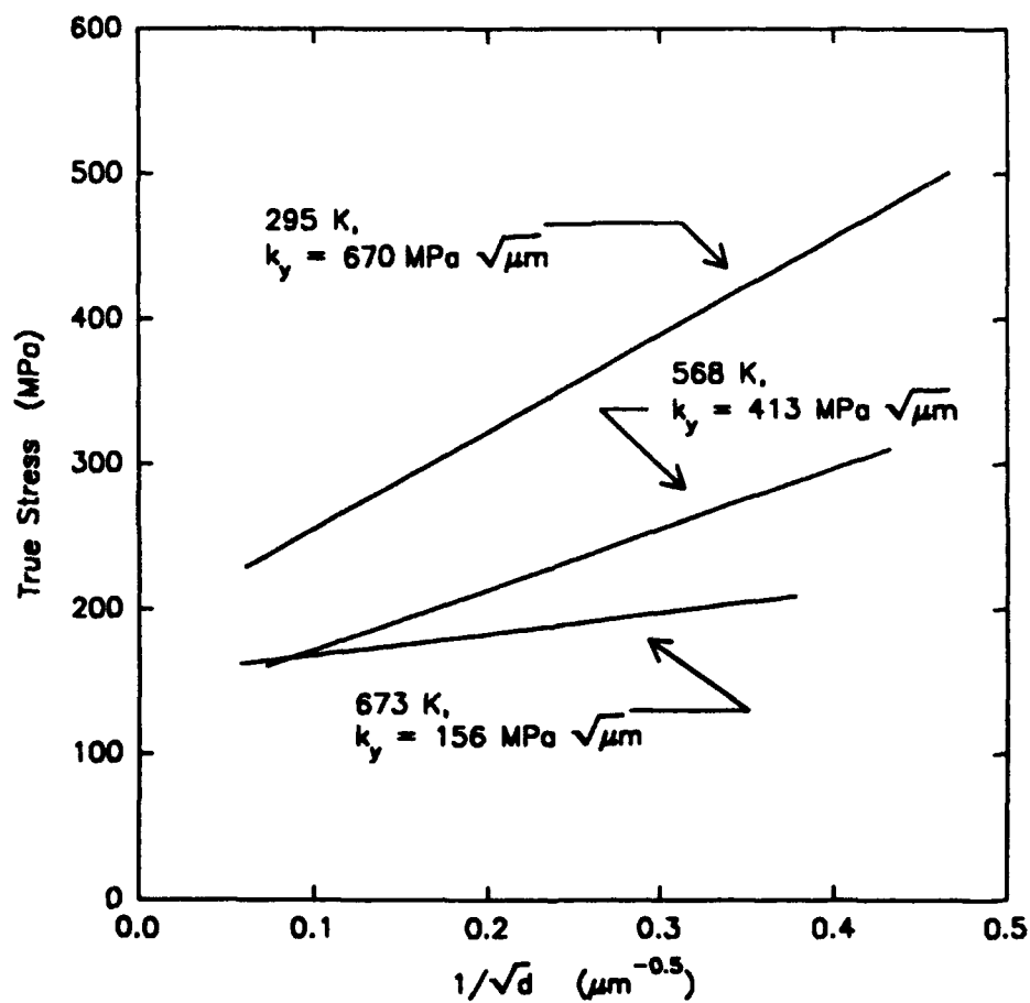
Figure 16.—The effect of temperature on the Hall-Petch slope of Ni-49Al-0.012Zr (ref. 251).
