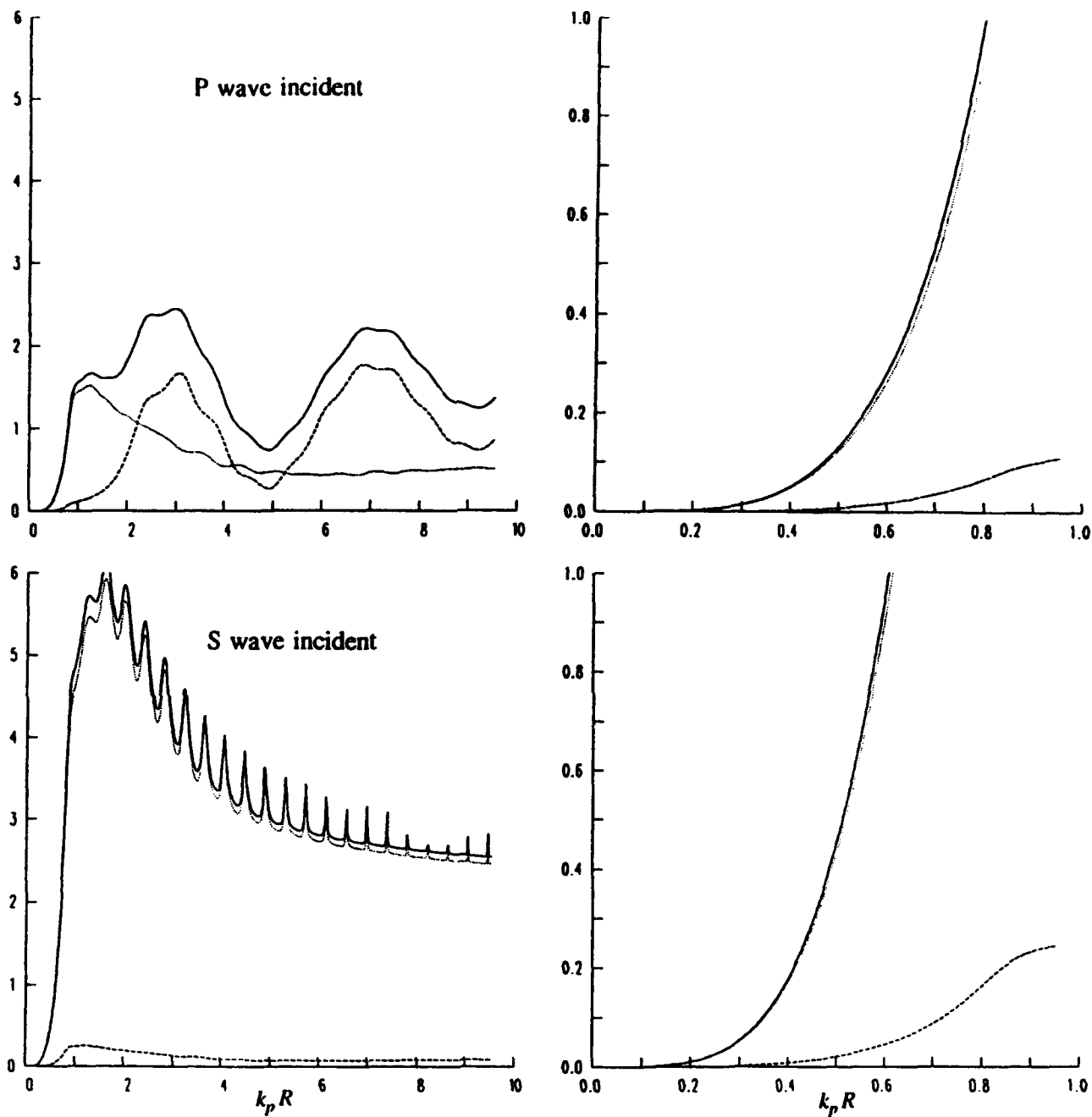
Figure 3 Similar to Figure 1 for the fluid inclusion which is listed as model 3 in the text.
