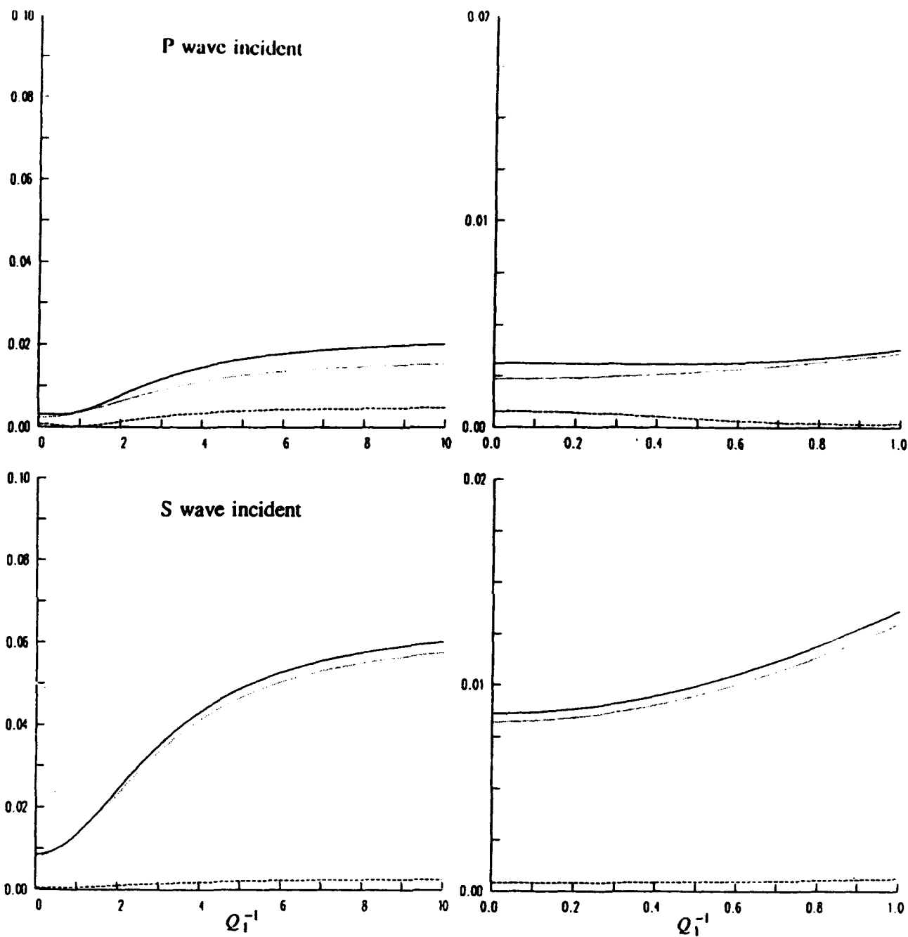
Figure 7 Similar to Figure 6 for the low-velocity inclusion which is listed as model 2 in the text.
