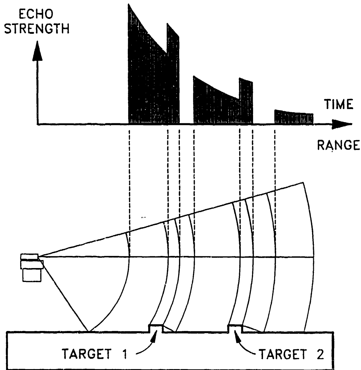
FIGURE 3-45. ECHO STRENGTH VS TIME WHEN FAN-SHAPED SONAR BEAM INTERSECTS WITH A FLAT BOTTOM AND TARGETS (Imagenex Operator's Manual)
