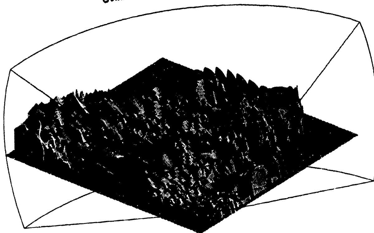
FIGURE 3-53. 3D CONTOUR PLOT OUTPUT OF CSARS SYSTEM (Jonathan Lott)
