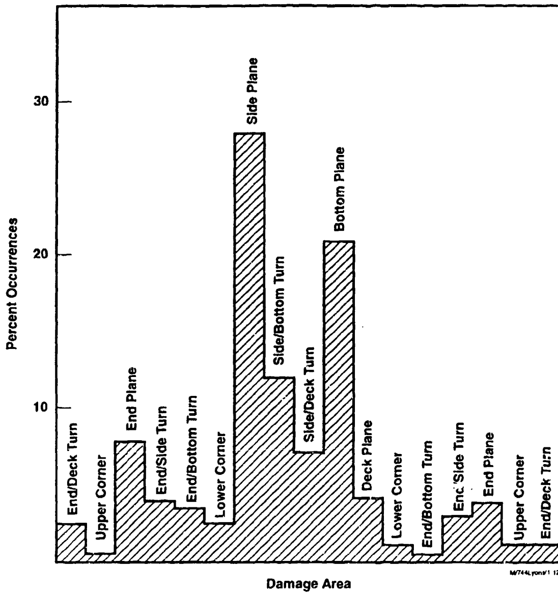
FIGURE 2-7. FREQUENCY OF DAMAGE IN MAJOR BARGE AREAS
