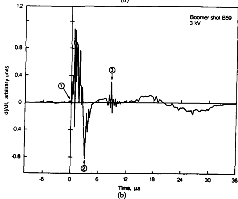
Figure 4: (a) Boomer I current waveform, Shot No. B59, fired at 3.0 kV. (b) The first time derivative of Boomer current in (a). (c) The second time derivative of Boomer current in (a). (d) The associated 1st breakwire waveform (digitized lower trace of Figure 5(a)). (e) The associated 2nd breakwire waveform (digitized upper trace of Figure 5(a)). The encircled numbers identify special features. (1) marks the time of onset of Boomer current, (2) the time of bridge burst, (3) the random discharge/switching noise, (4) the 1st wire break and (5) the second wire break.
