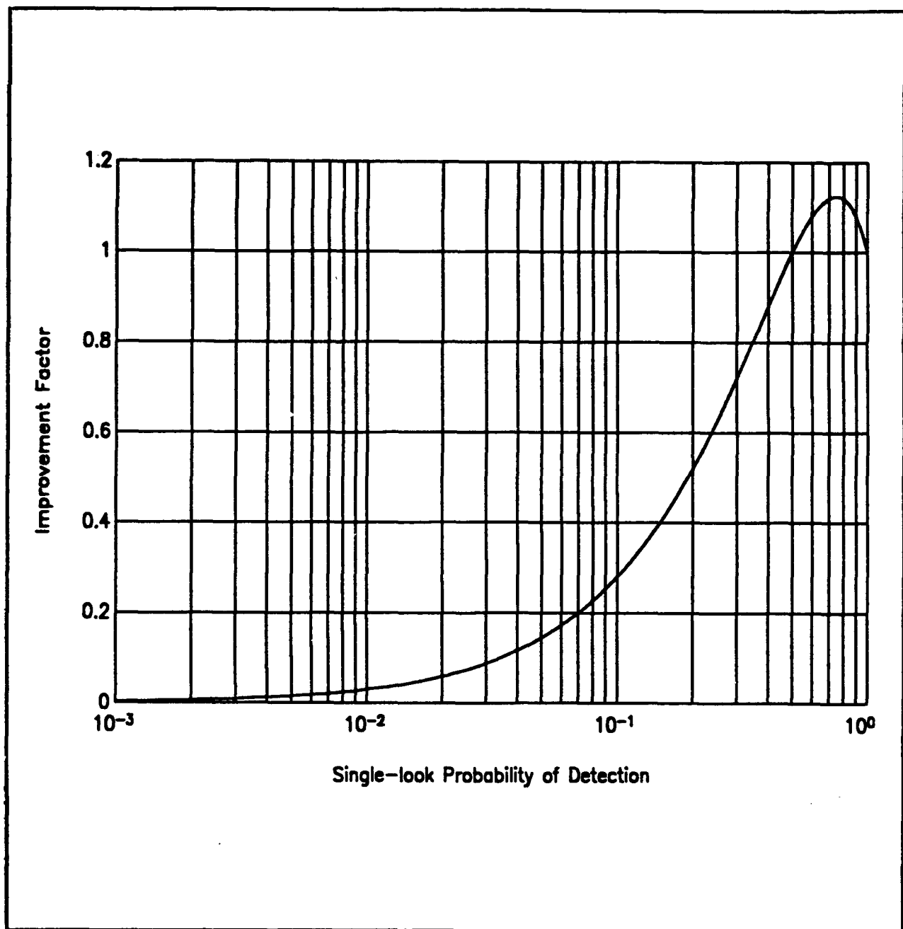
Figure 2-6 Improvement Factor for 2 Hits out of 3 Looks
