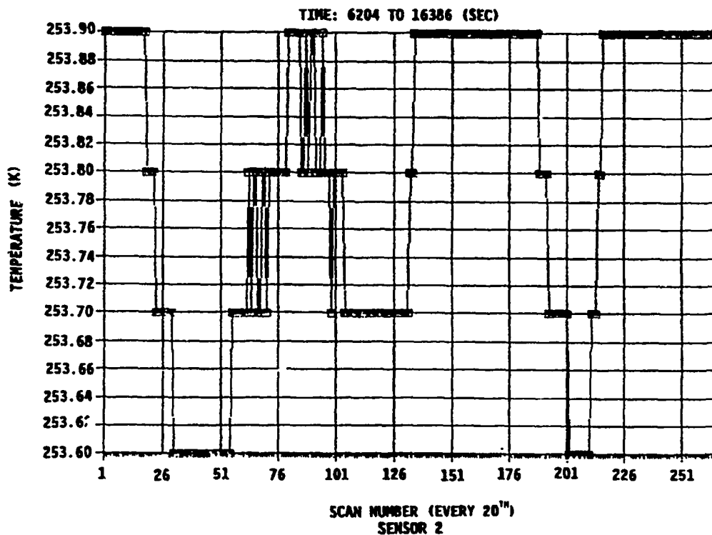
FIGURE 4.16 VARIATION OF HOT LOAD TEMPERATURE SENSORS 1 AND 2 (REV 438)
