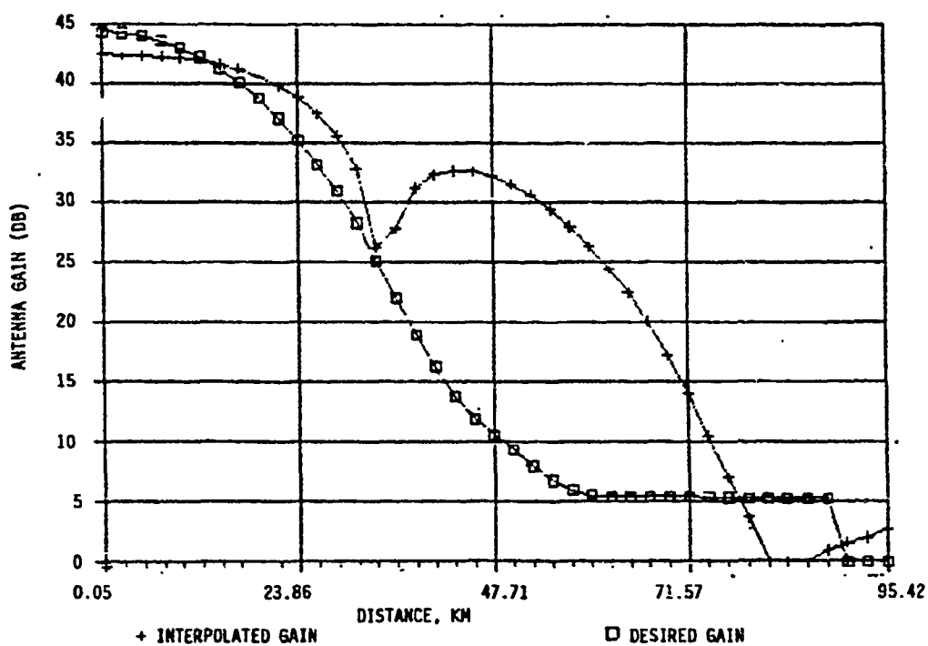
FIGURE 3.12. INTERPOLATED PATTERNS OF 37 GHz DATA (MIDPOINT / BETWEEN SCANS AND SAMPLES)
