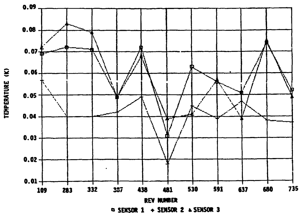
FIGURE 4.17 STANDARD DEVIATION OF HOT LOAD TEMPERATURES
