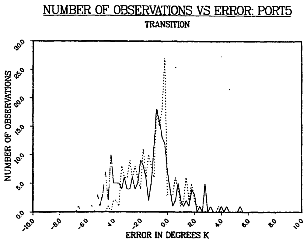
Figure-3.6. Histogram of Level 2 APC Errors at 37 GHz (— Current APC, --- No APC)
