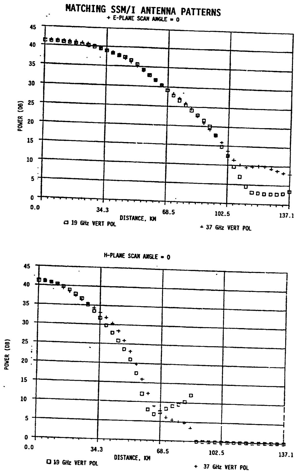
FIGURE 3.8 SMOOTHED 37 GHz ANTENNA PATTERN AND 19 GHz PATTERN
