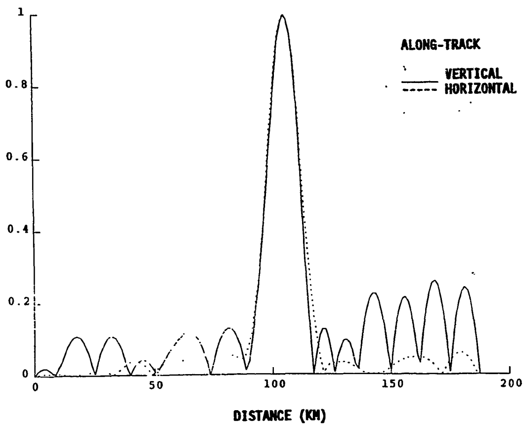
FIGURE 4.25 85 GHZ DERIVED ANTENNA GAIN FUNCTION
