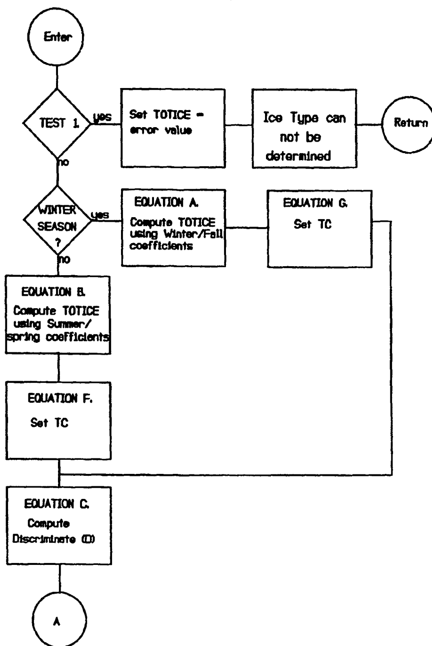
Figure 1-21. Flow Chart of Recommended Ice Concentration Algorithm
