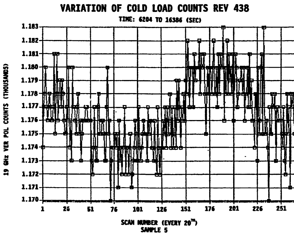
FIGURE 4.15 VARIATION OF 19 GHz VERTICAL POLARIZATION COLD LOAD SAMPLE 5 (REV 438)
