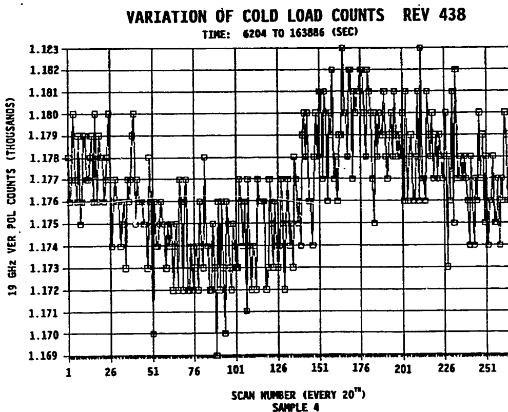
FIGURE 4.14 VARIATION OF 19 GHz VERTICAL POLARIZATION COLD LOAD SAMPLES 3 AND 4 (REV 438)
