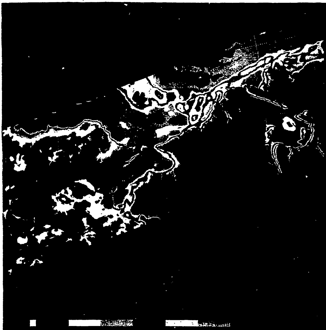
Figure 1.17. Hughes Algorithm Total Ice Concentration REV 2194
