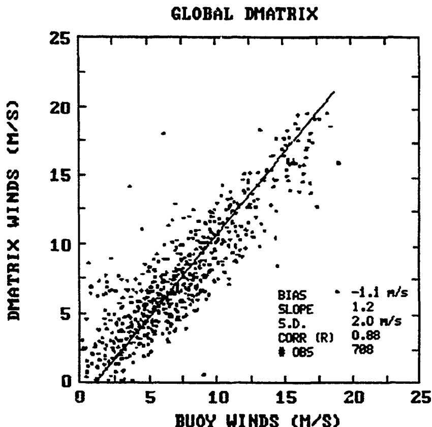
Figure 1.16. Performance of the Global D-Matrix Algorithm
