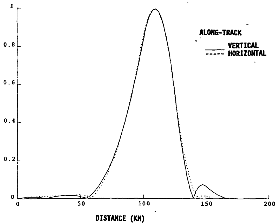
FIGURE 4.24 37 GHZ DERIVED ANTENNA GAIN FUNCTION
