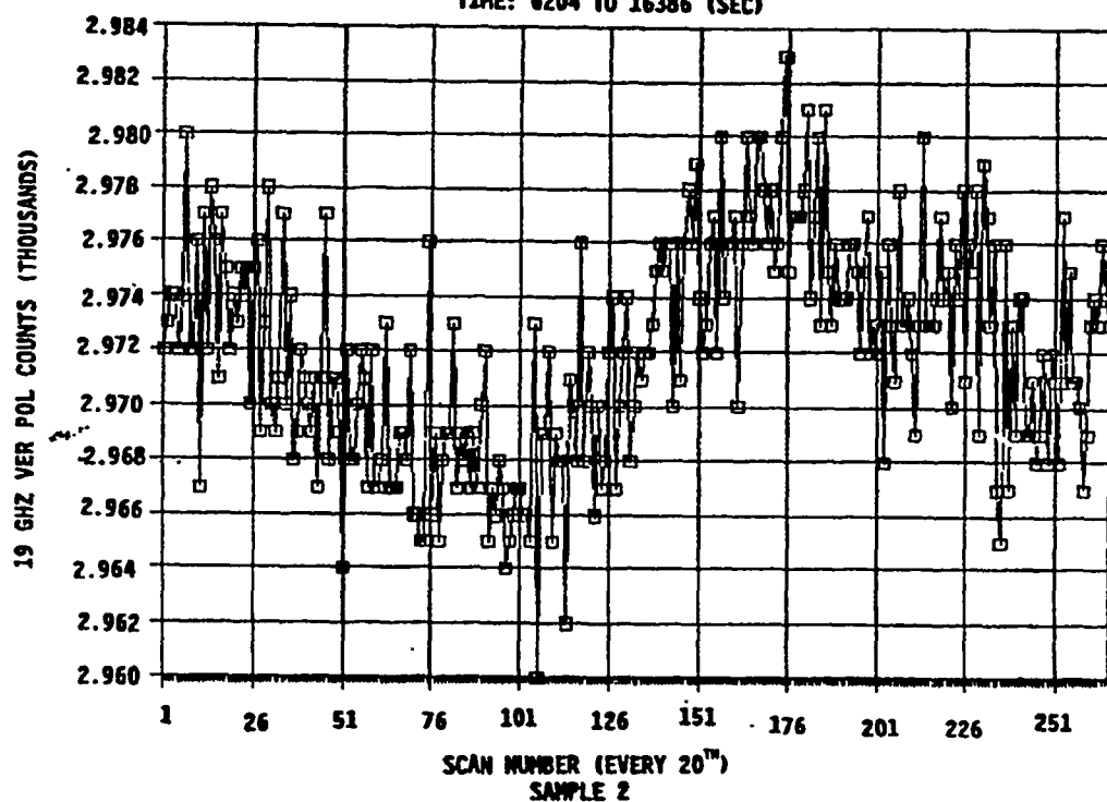
FIGURE 4.10 VARIATION OF 19 GHz VERTICAL POLARIZATION HOT LOAD SAMPLES 1 AND 2 (REV 438)
