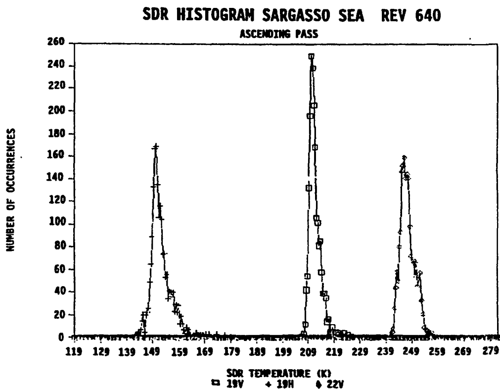
FIGURE 4.21 19 AND 22 GHZ HISTOGRAMS OF THE SARGASSO SEA REVS 407 (7/18/87) AND 640 (8/4/87)
