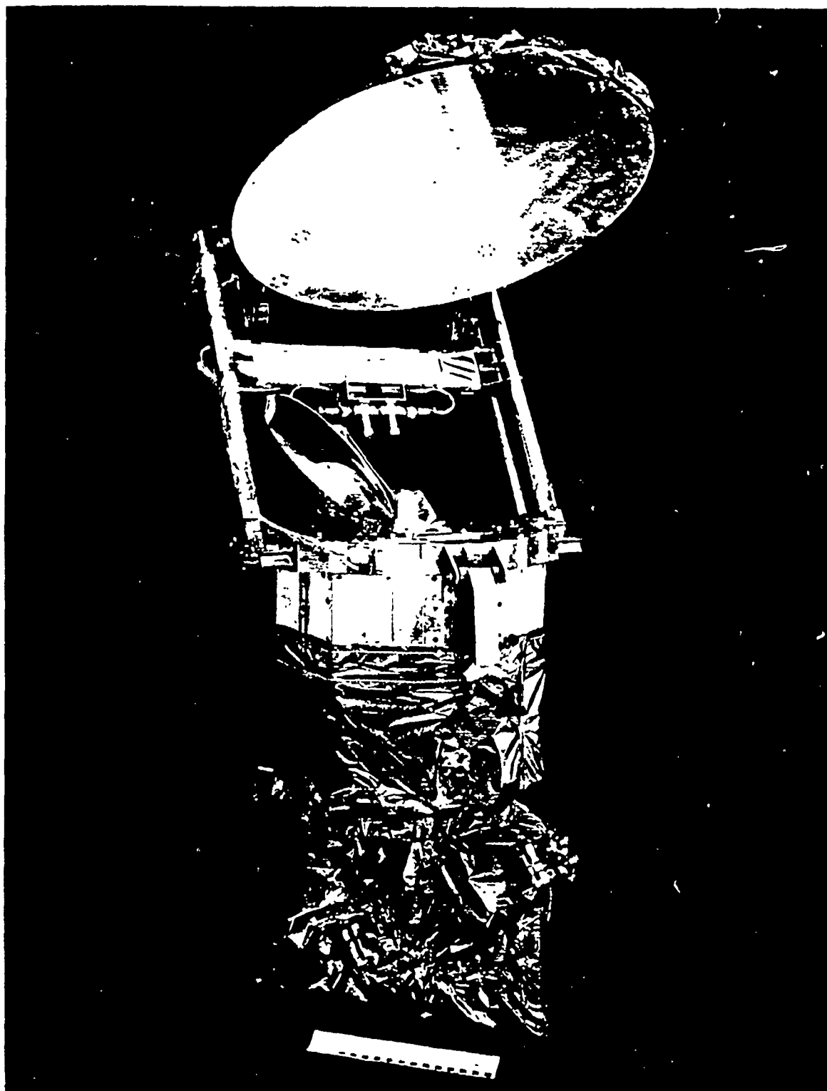
Figure 2.4 SSM/I in Deployed Position
