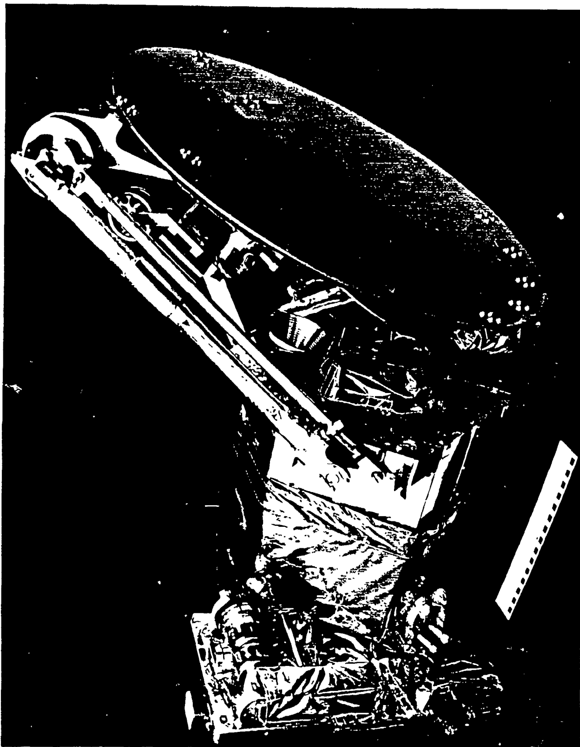
Figure 2.3 SSM/I in Stowed Position
