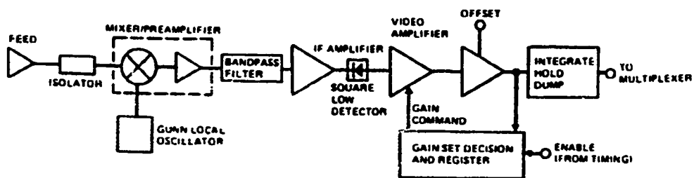
Figure 2.2 Radiometer Block Diagram
