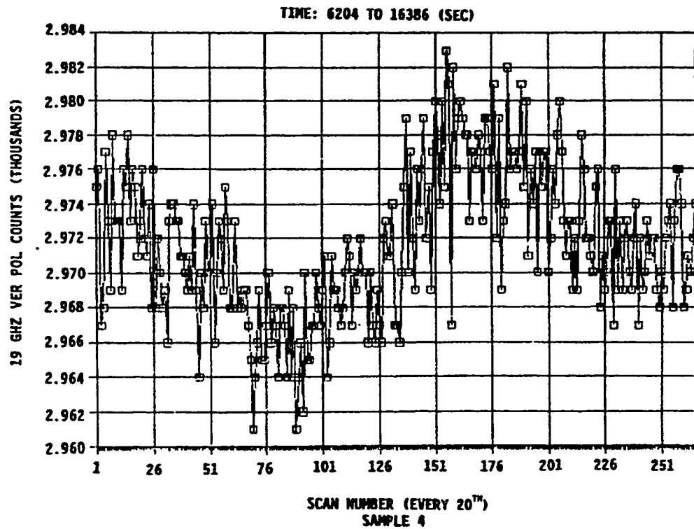
FIGURE 4.11 VARIATION OF 19 GHZ VERTICAL POLARIZATION HOT LOAD SAMPLES 3 AND 4 (REV 438)
