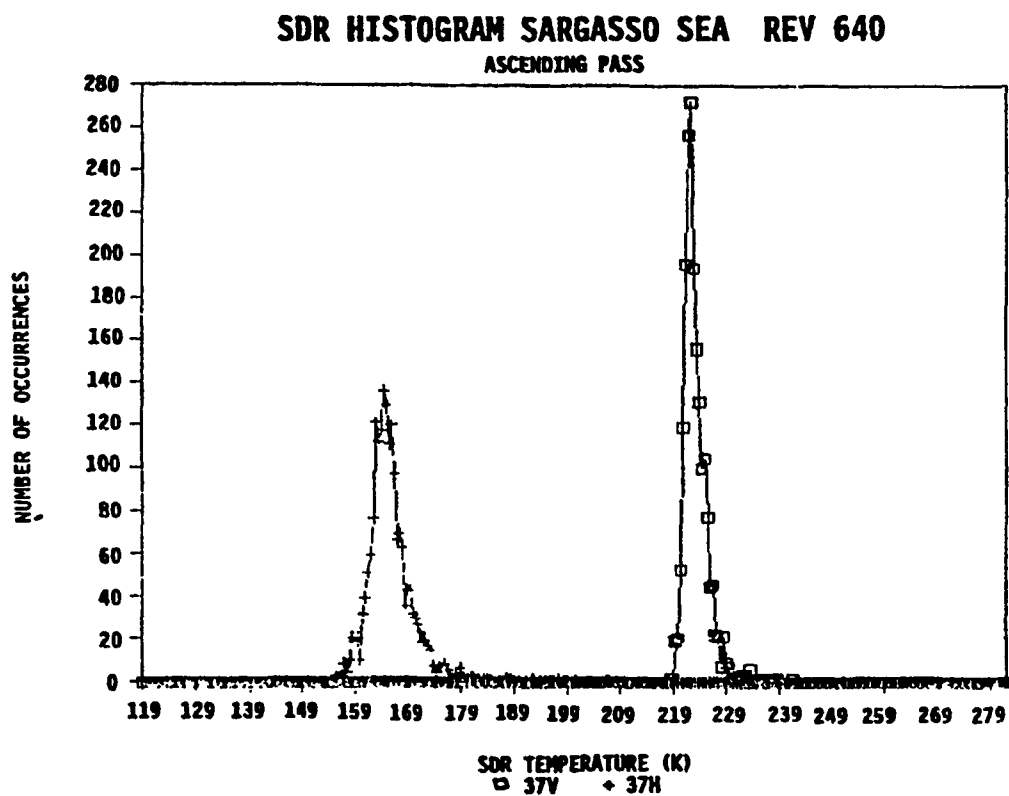
FIGURE 4.22 37 GHZ HISTOGRAMS OF THE SARGASSO SEA REVS 407 (7/18/87) AND 640 (8/4/87)
