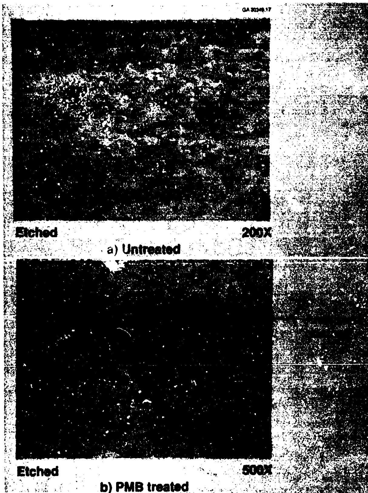
Figure 3.30 Sections Through 0.032 in. Anodized 2024-T3 Sheet
