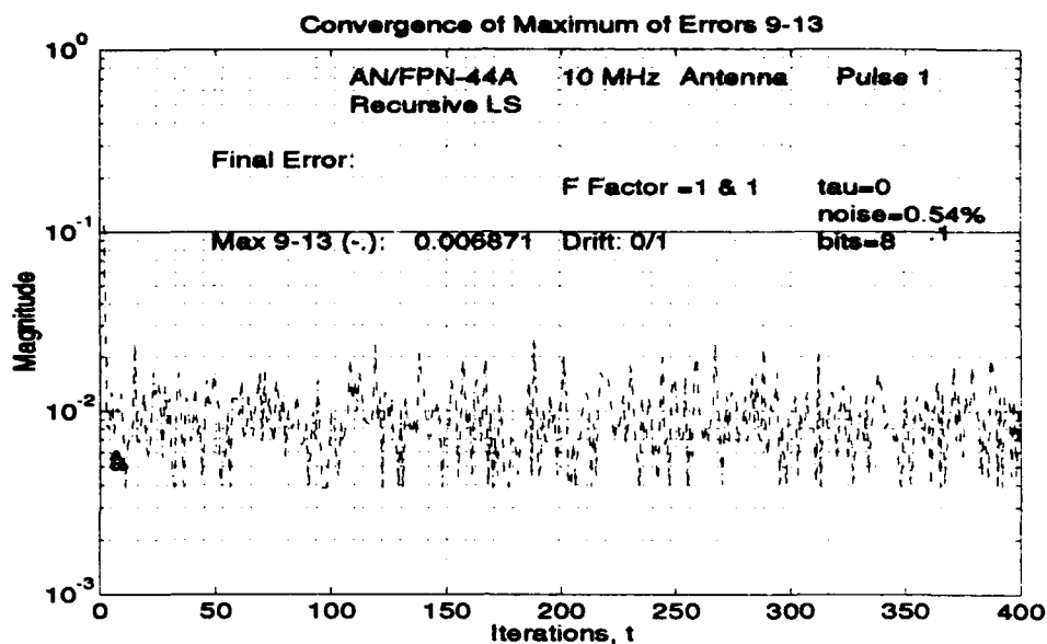
Figure A.4: Maximum error of peaks 9-13 using the RLS control algorithm (8 bits, noise variance of 9.3\text{e-}4 ).
