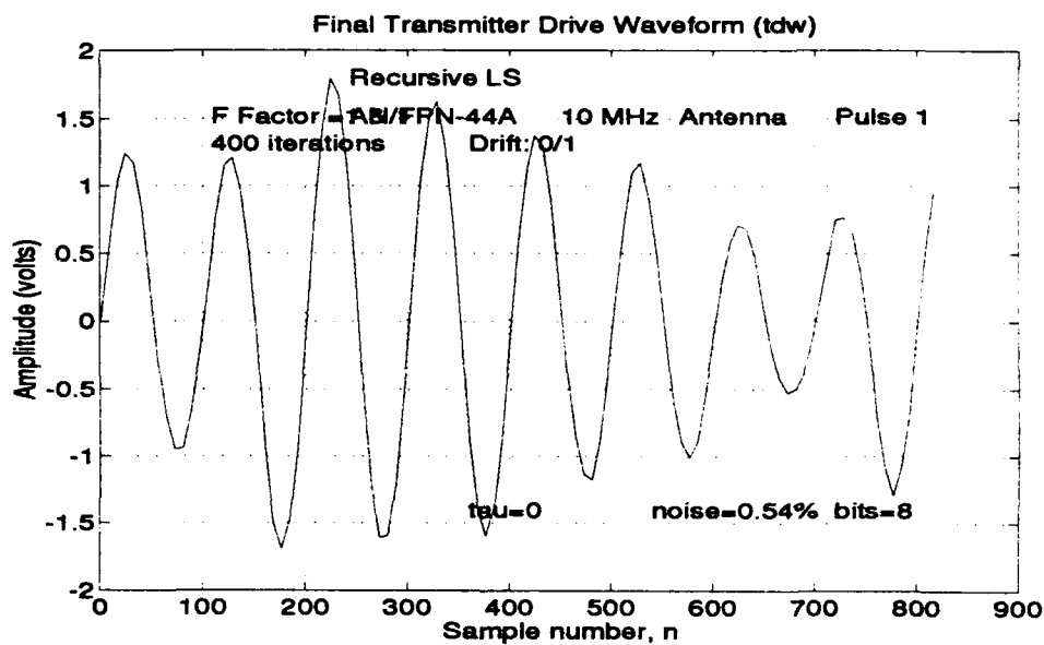
Figure A.5: TDW produced after 400 iterations using the RLS control algorithm (8 bits, noise variance of 9.3\text{e-}4 ).
