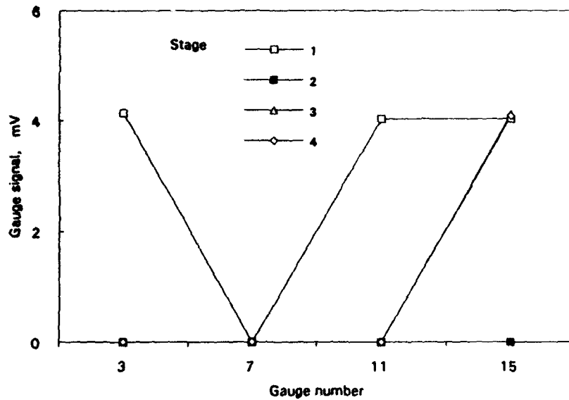
Figure 13: Span signals (0 to 125 kN) of adhesive longitudinal gauges L1G3, L1G7, L2G11 and L2G15. Spans of the gauges were not measured following Stage 2. Gauges L1G3 and L1G11 were unserviceable after Stage 2. Gauge L1G7 remained unserviceable after attachment. Note small changes in span for gauge L2G15 after each stage.
